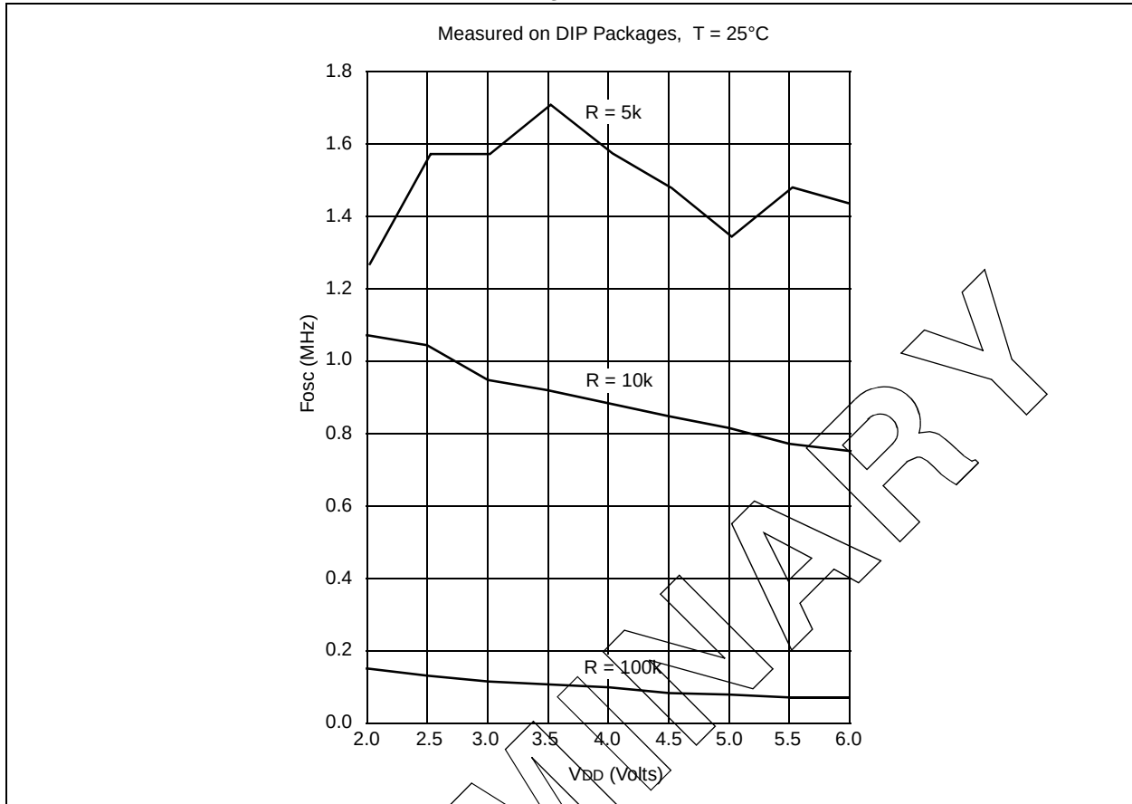
FIGURE 13-4: TYPICAL RC OSCILLATOR FREQUENCY vs. V_{DD} , C_{EXT} = 300\text{ pF}
