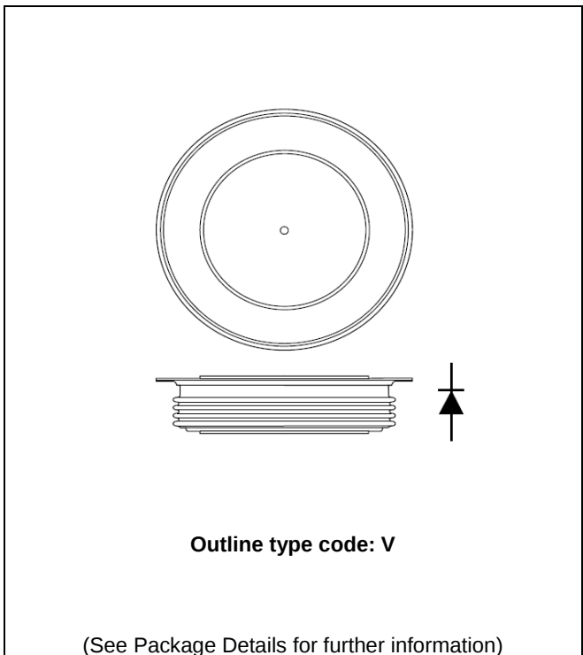
Fig. 1 Package outline
