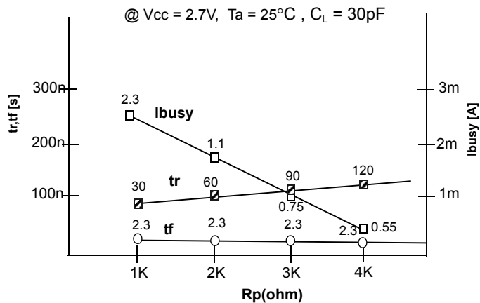
Fig 23 R_p vs t_r, t_f & R_p vs i_{busy}
