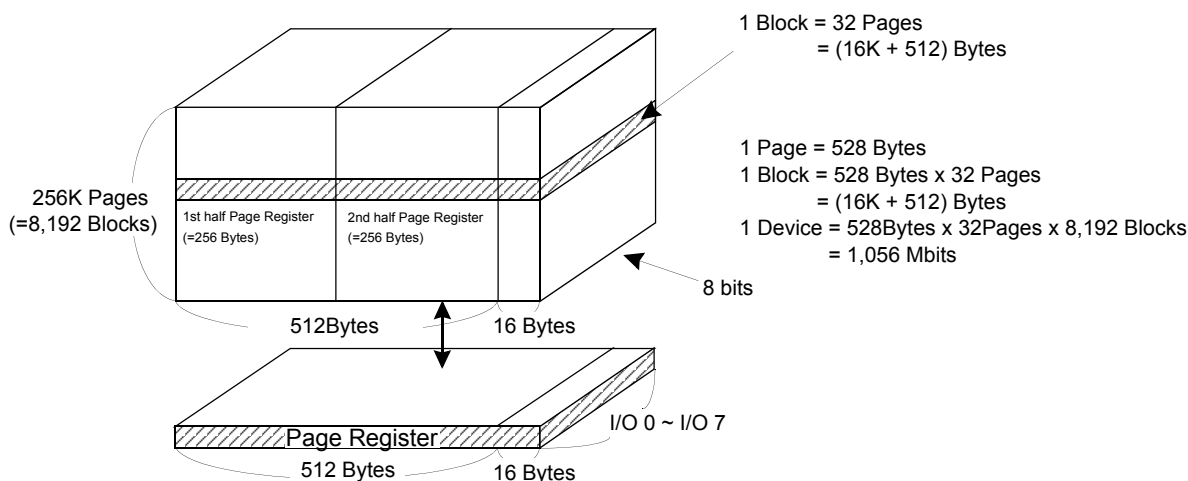
Figure 2. K9T1G08B0M ARRAY ORGANIZATION
