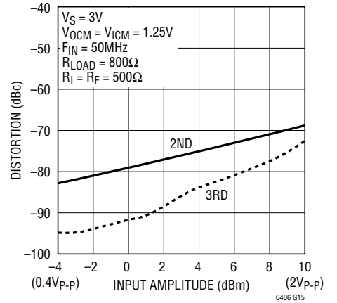
Single-Ended Harmonic Distortion vs Input Amplitude
