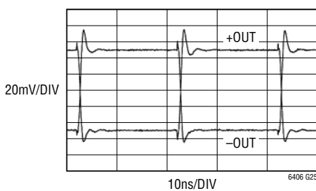
Small Signal Step Response
