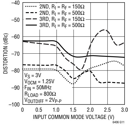
Single-Ended Harmonic Distortion vs Input Common Mode Voltage
