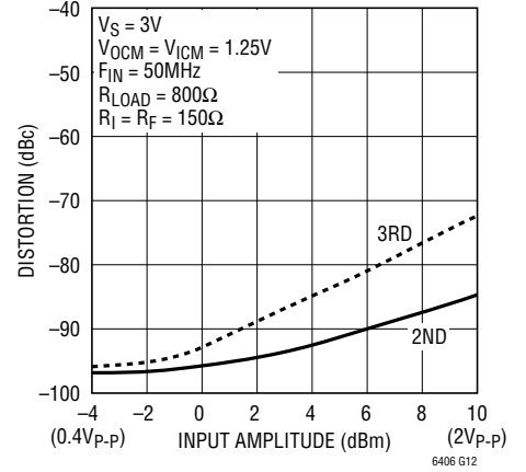
Differential Harmonic Distortion vs Input Amplitude
