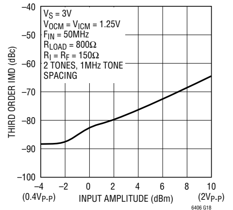
Differential Intermodulation Distortion vs Input Amplitude
