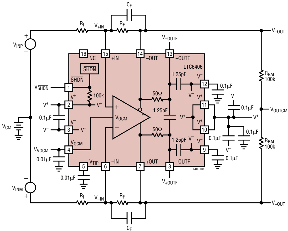
Figure 1. DC Test Circuit
