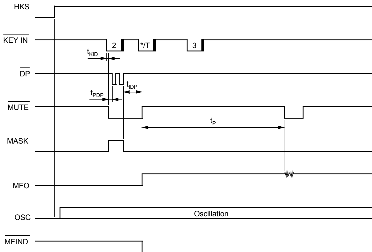
Figure 10. Pulse-to-tone Operation
