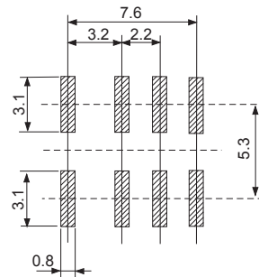
Recommended mounting pad (Tolerance: \pm 0.1\text{mm} )
