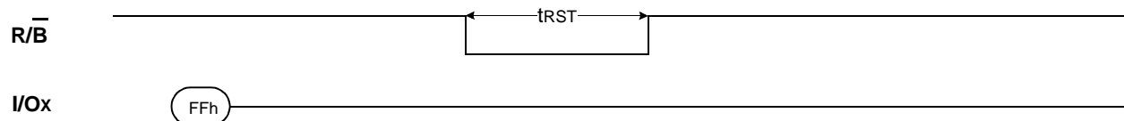
Figure 12. RESET Operation
