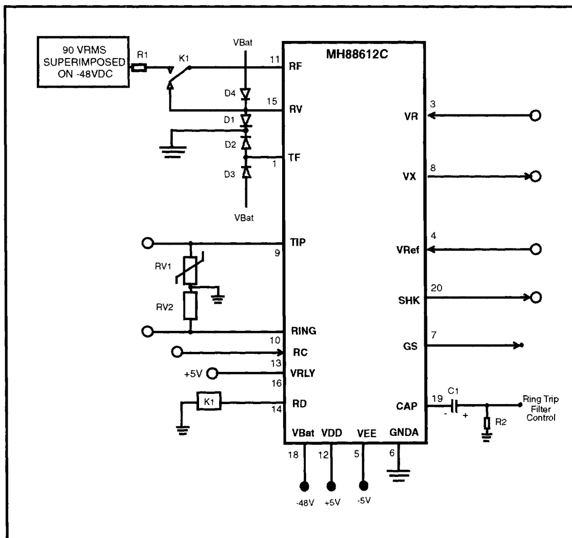
Figure 3 - Application Circuit
