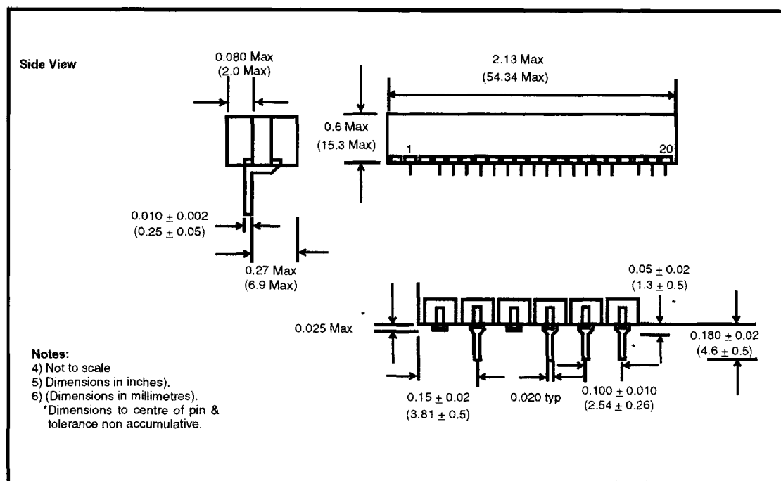
Figure 4 - Mechanical Data
