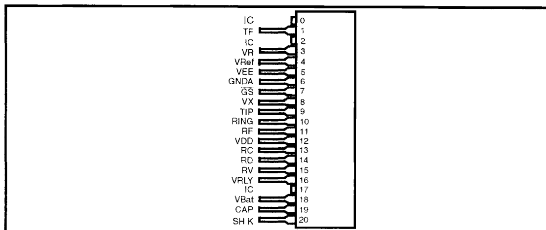
Figure 2 - Pin Connections
