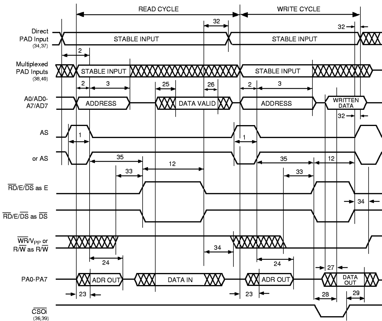
Figure 36. Port A as AD0–AD7 Timing (Track Mode), CRRWR = 1 (PSD3X2/3X3/3X4R)
