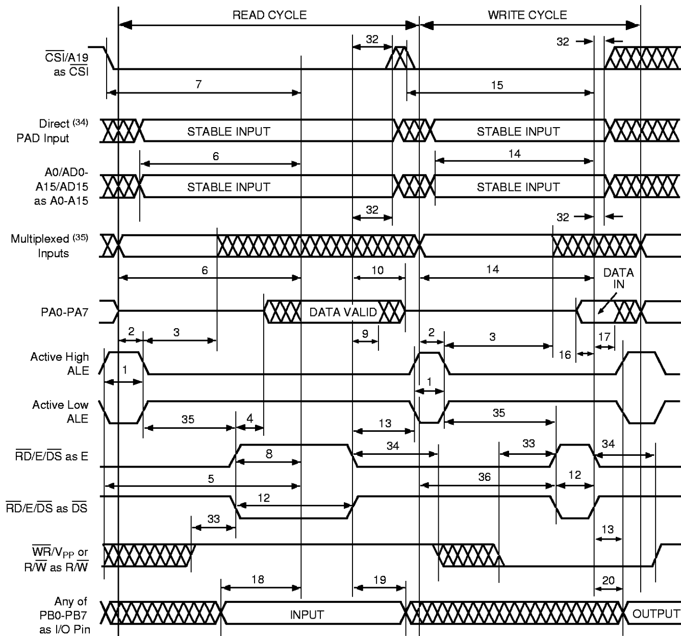
Figure 27. Timing of 8-Bit Non-Multiplexed Address/Data Bus, CRRWR = 1 (PSD3X2/3X3/3X4R)
