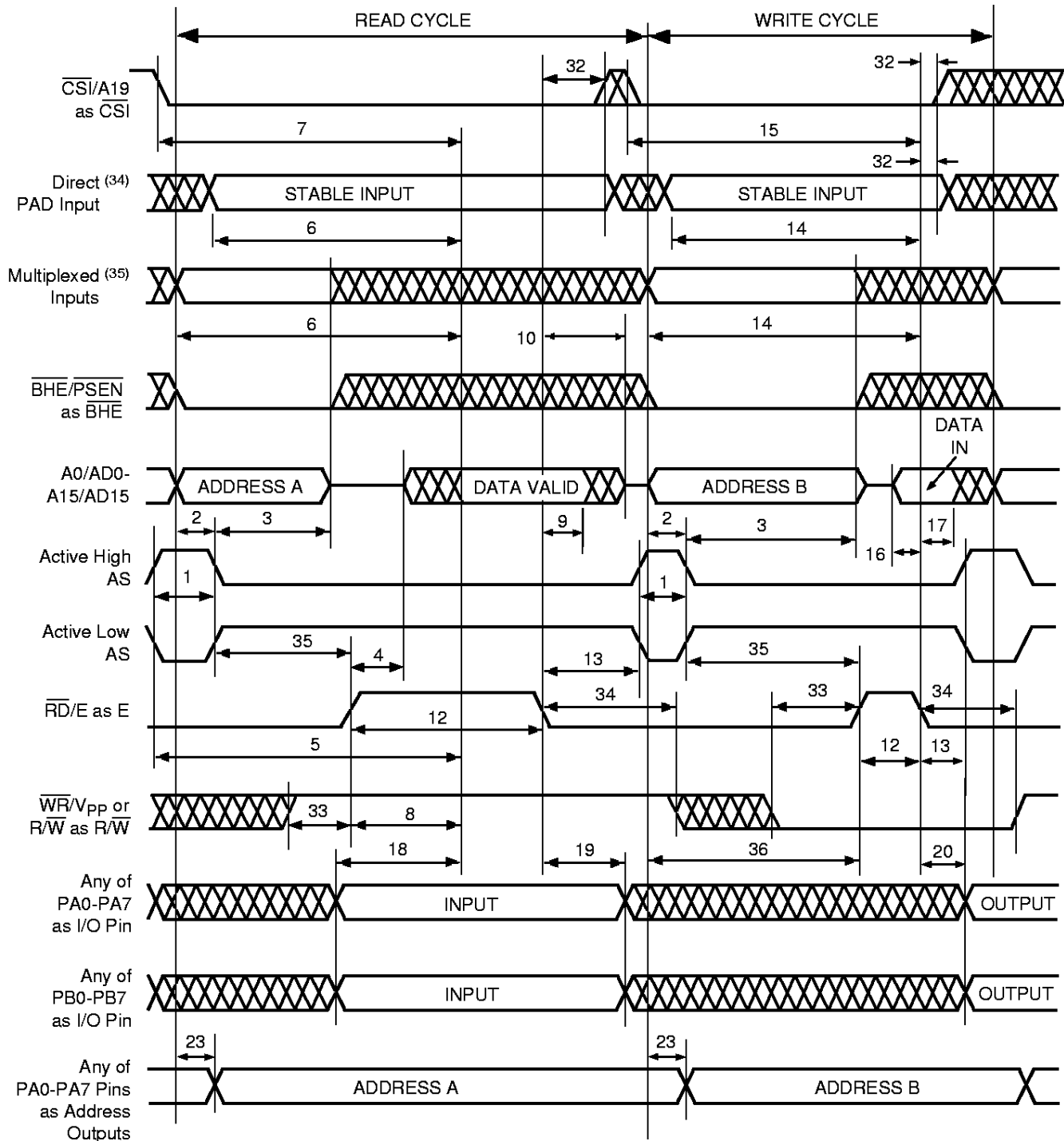
Figure 22. Timing of 16-Bit Multiplexed Address/Data Bus, CRRWR = 1 (PSD3X1)
