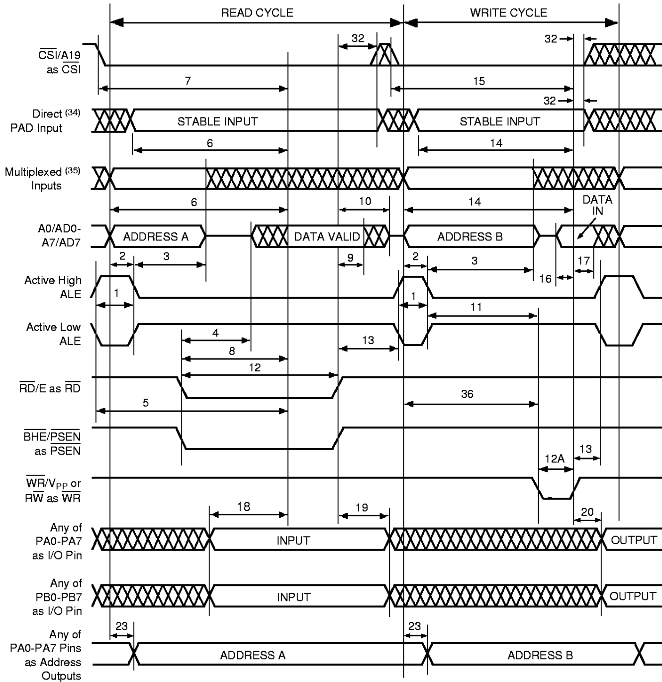
Figure 16. Timing of 8-Bit Multiplexed Address/Data Bus, CRRWR = 0 (PSD3X1)
