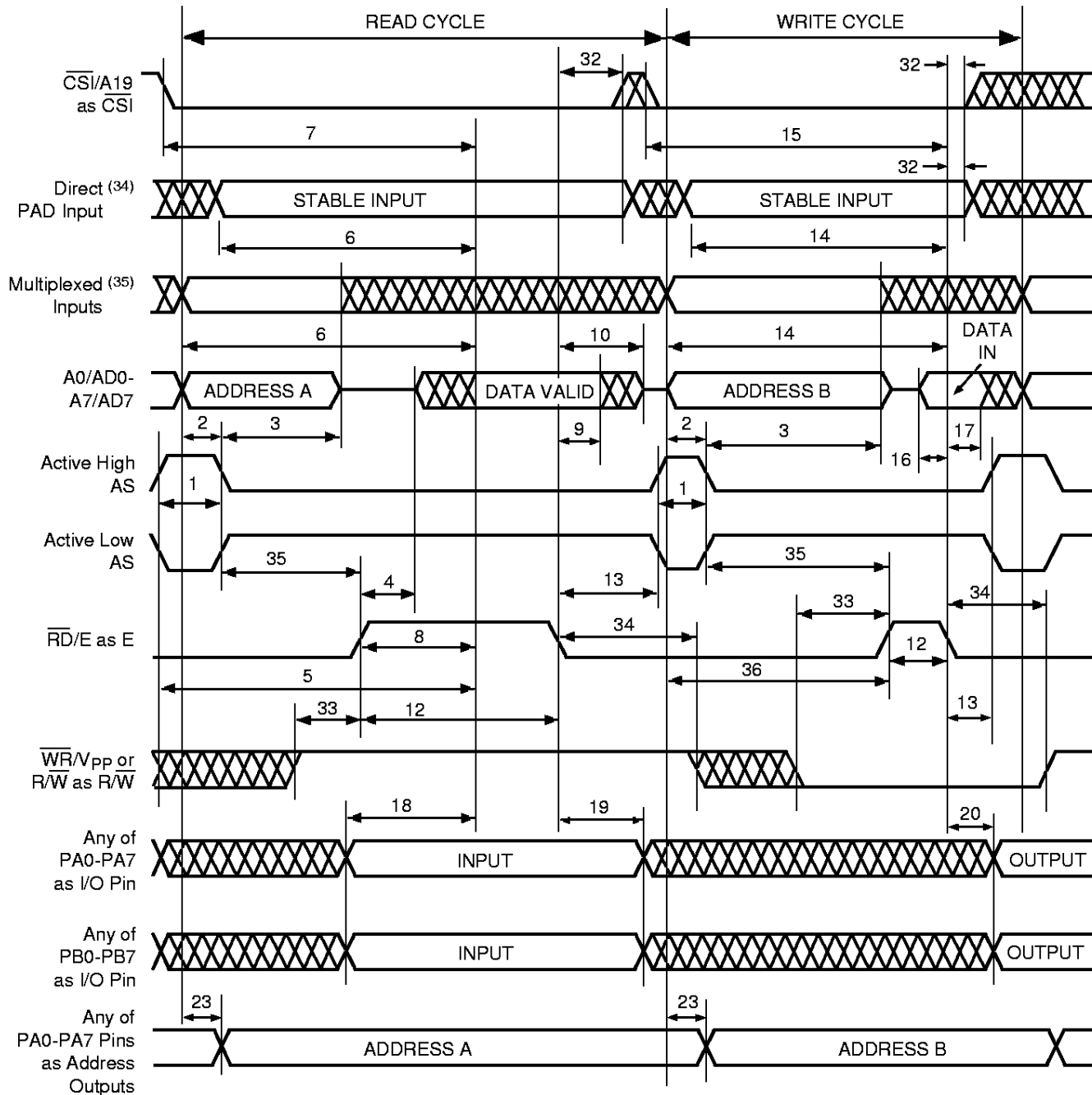
Figure 18. Timing of 8-Bit Multiplexed Address/Data Bus, CRRWR = 1 (PSD3X1)
