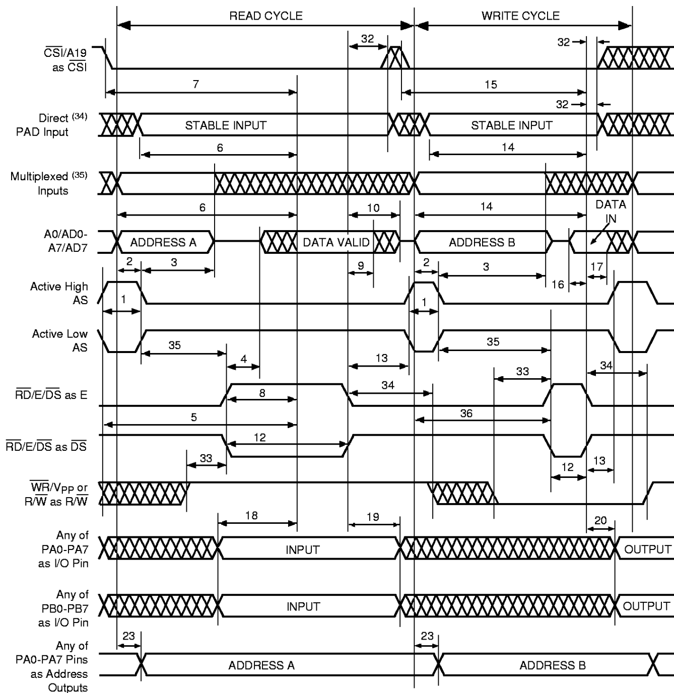
Figure 19. Timing of 8-Bit Multiplexed Address/Data Bus, CRRWR = 1 (PSD3X2/3X3/3X4R)
