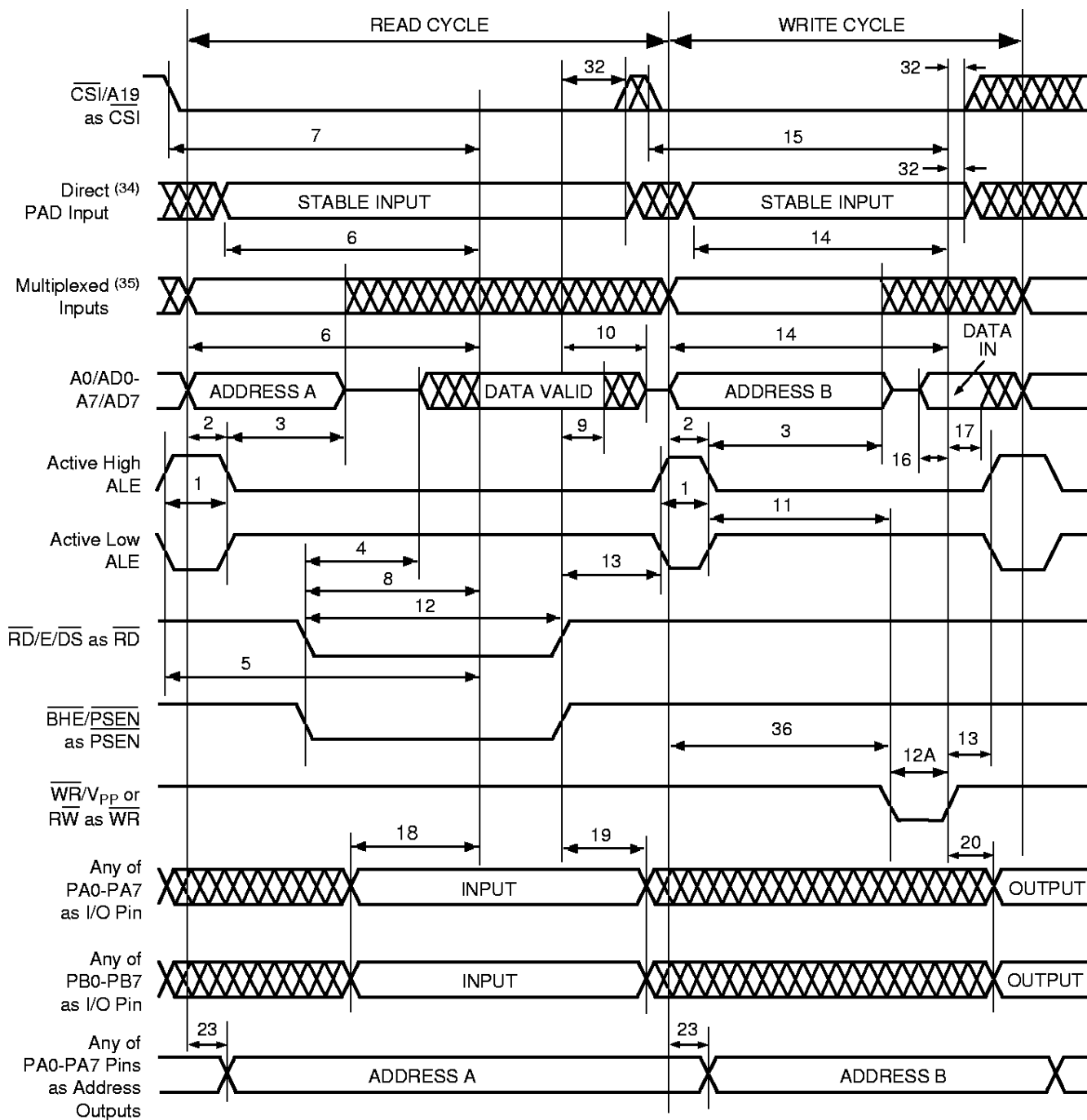
Figure 17. Timing of 8-Bit Multiplexed Address/Data Bus, CRRWR = 0 (PSD3X2/3X3/3X4R)
