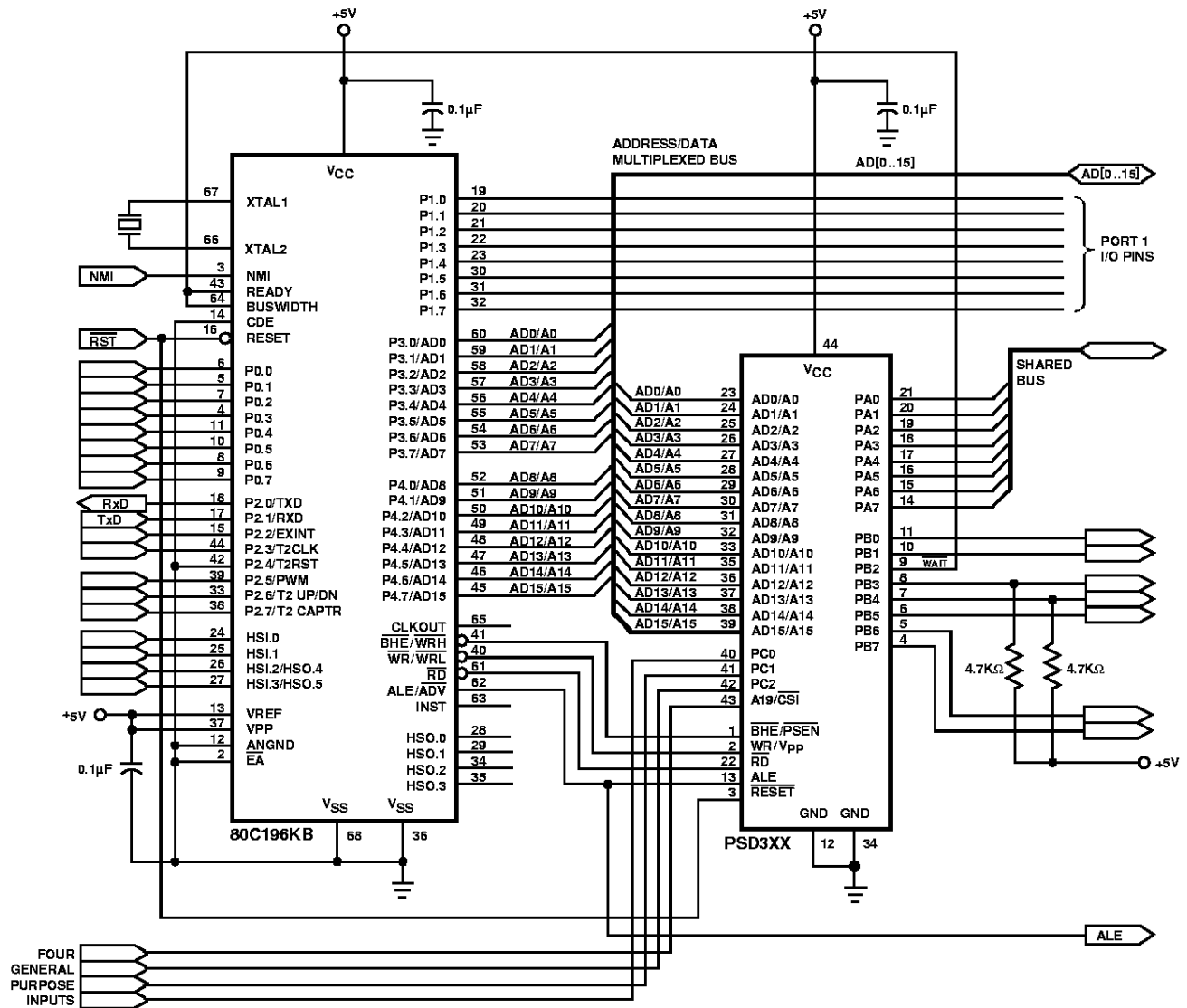
Figure 14. PSD3XX Interface With Intel's 80C196KB.
