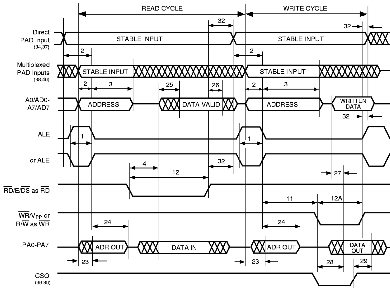
Figure 34. Port A as AD0-AD7 Timing (Track Mode), CRRWR = 0 (PSD3X2/3X3/3X4R)
