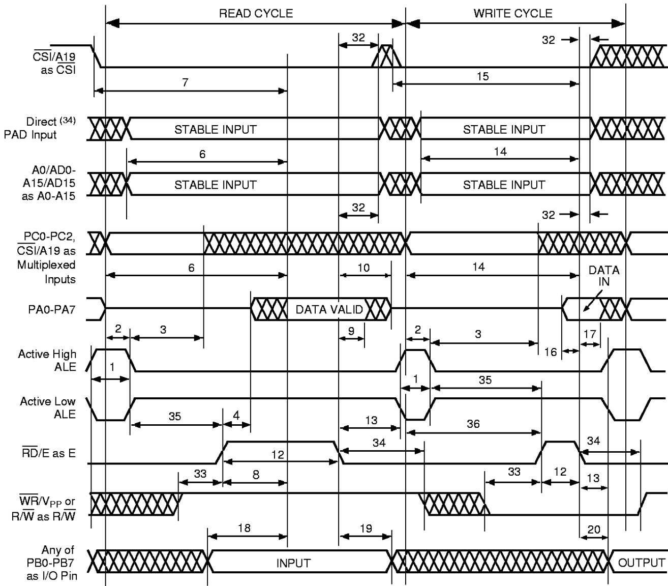
Figure 26. Timing of 8-Bit Non-Multiplexed Address/Data Bus, CRRWR = 1 (PSD3X1)
