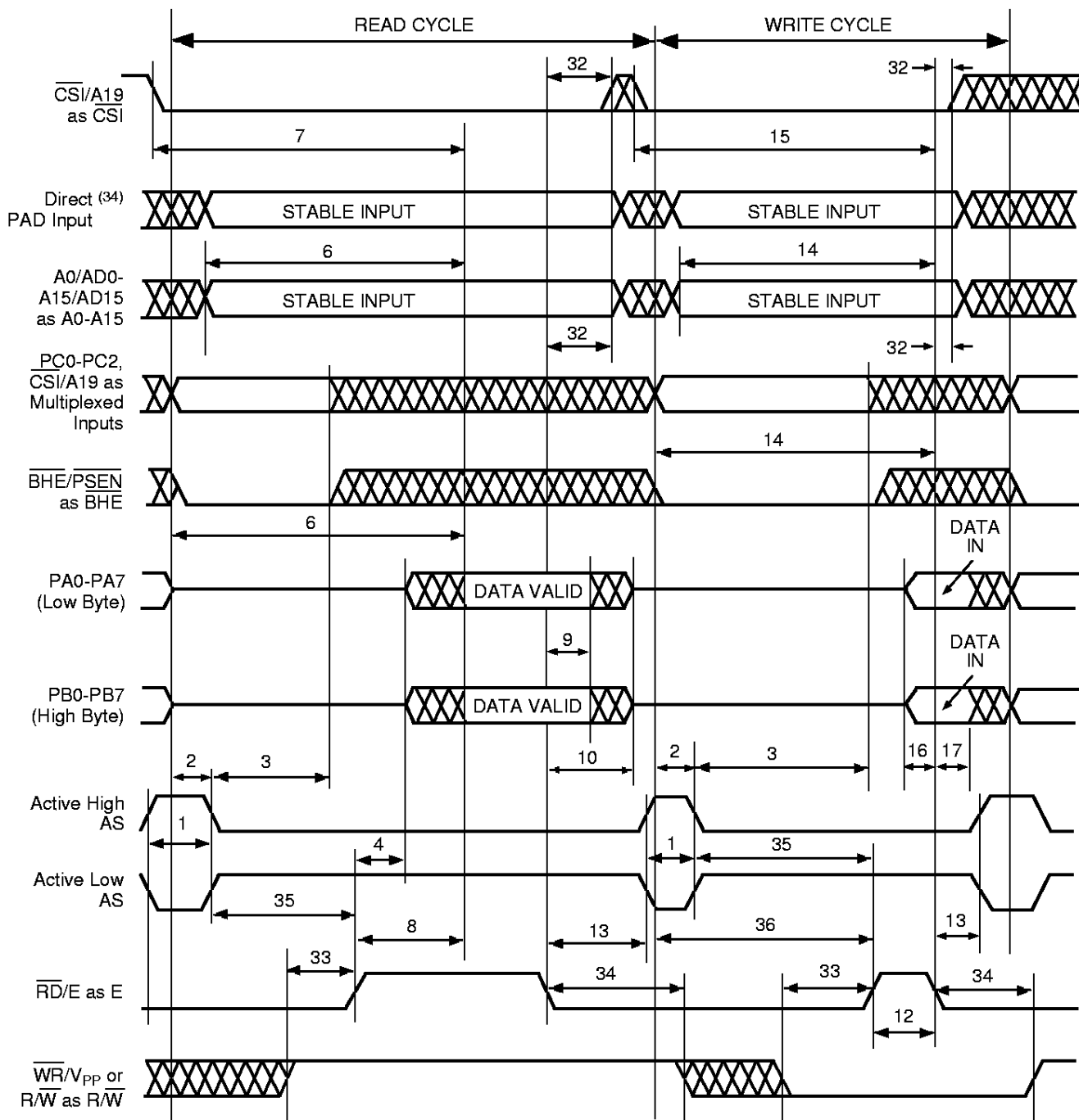
Figure 30. Timing of 16-Bit Non-Multiplexed Address/Data Bus, CRRWR = 1 (PSD3X1)
