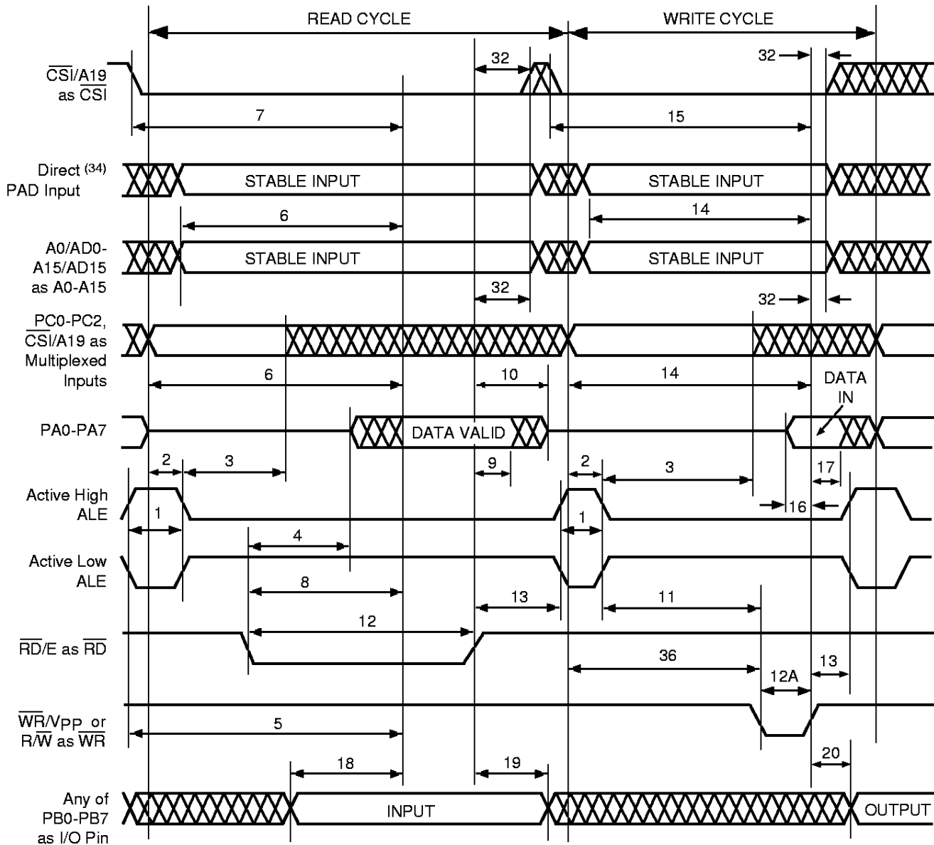
Figure 24. Timing of 8-Bit Non-Multiplexed Address/Data Bus, CRRWR = 0 (PSD3X1)
