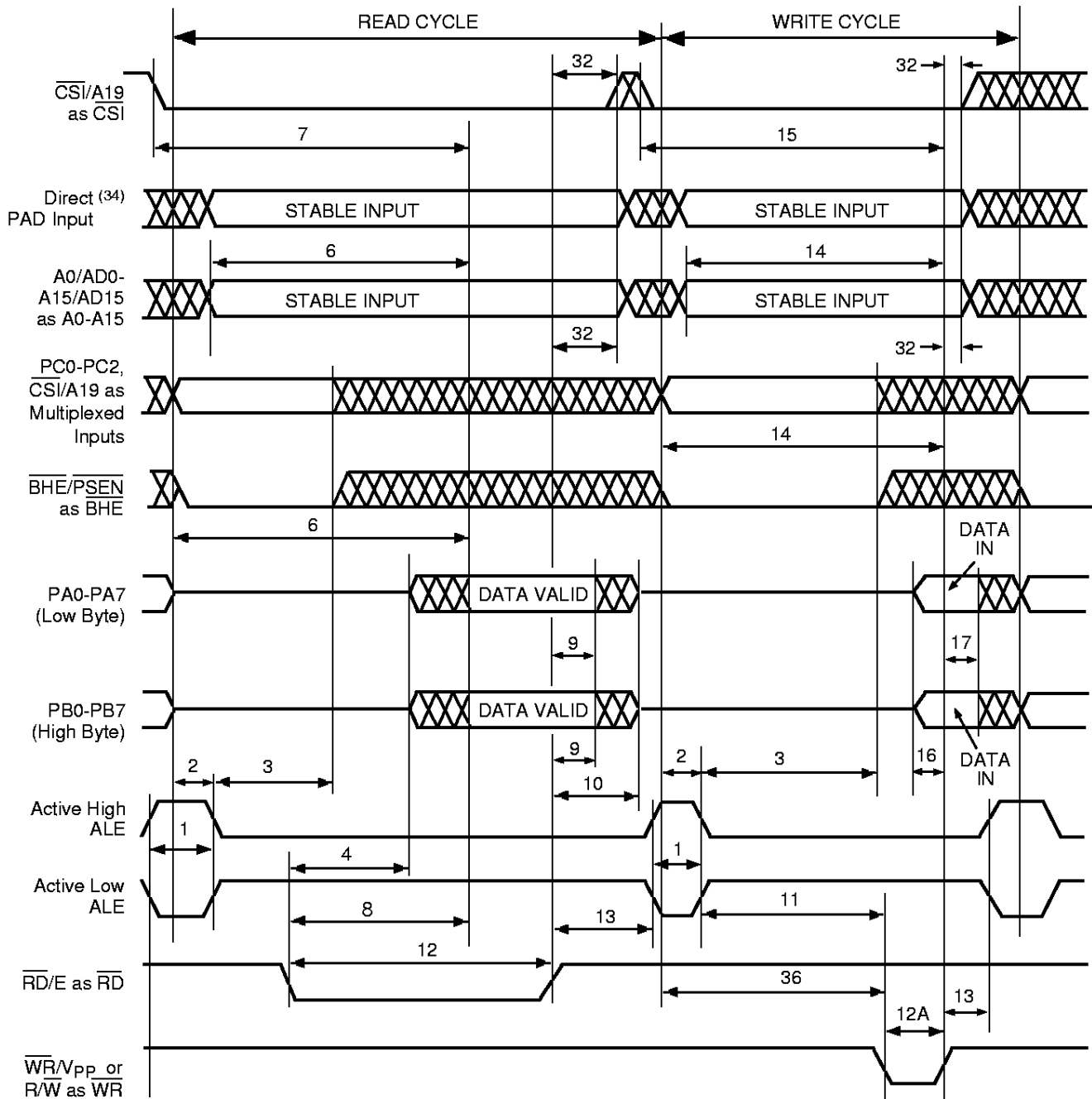
Figure 28. Timing of 16-Bit Non-Multiplexed Address/Data Bus, CRRWR = 0 (PSD3X1)
