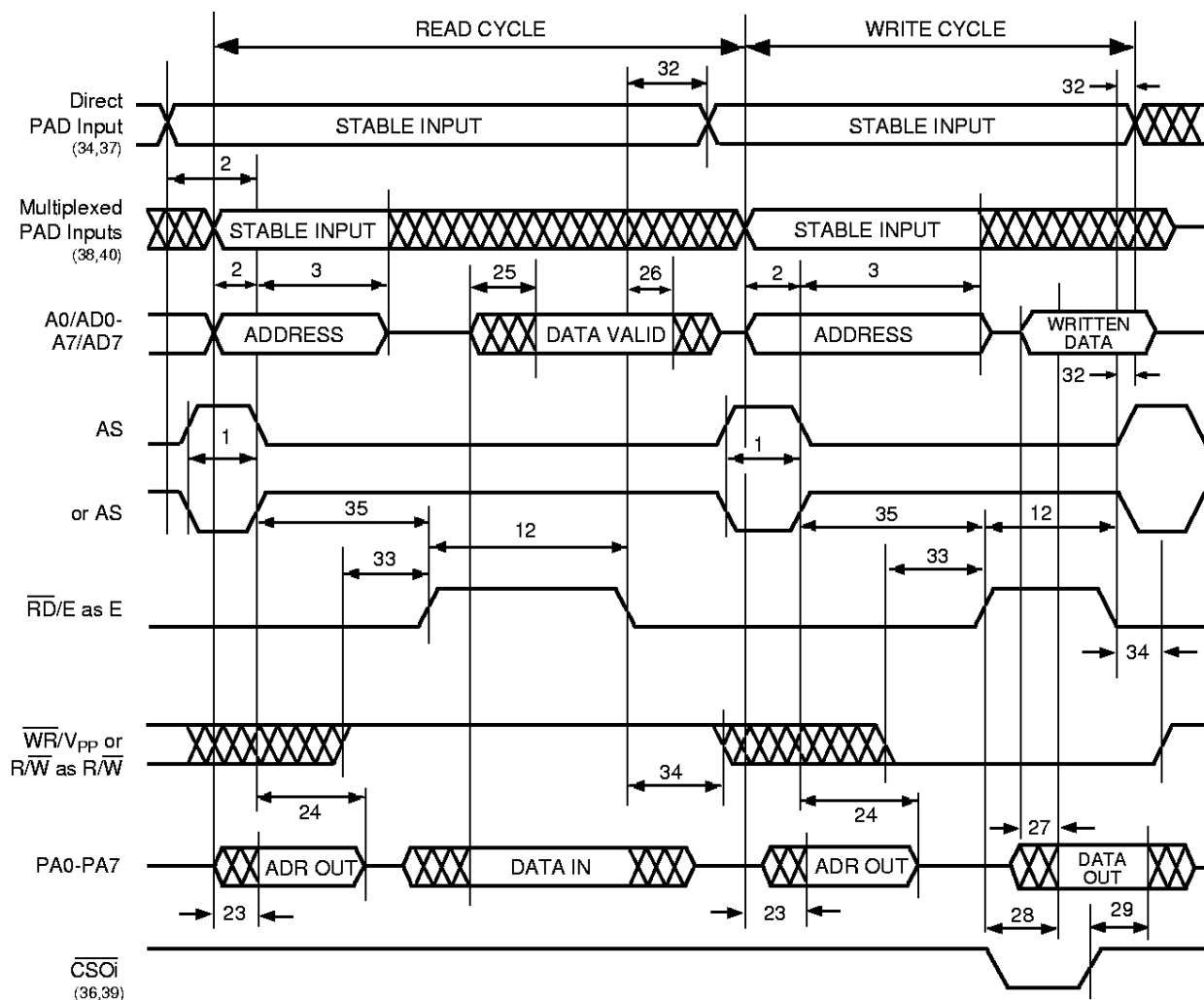
Figure 35. Port A as AD0-AD7 Timing (Track Mode), CRRWR = 1 (PSD3X1)
