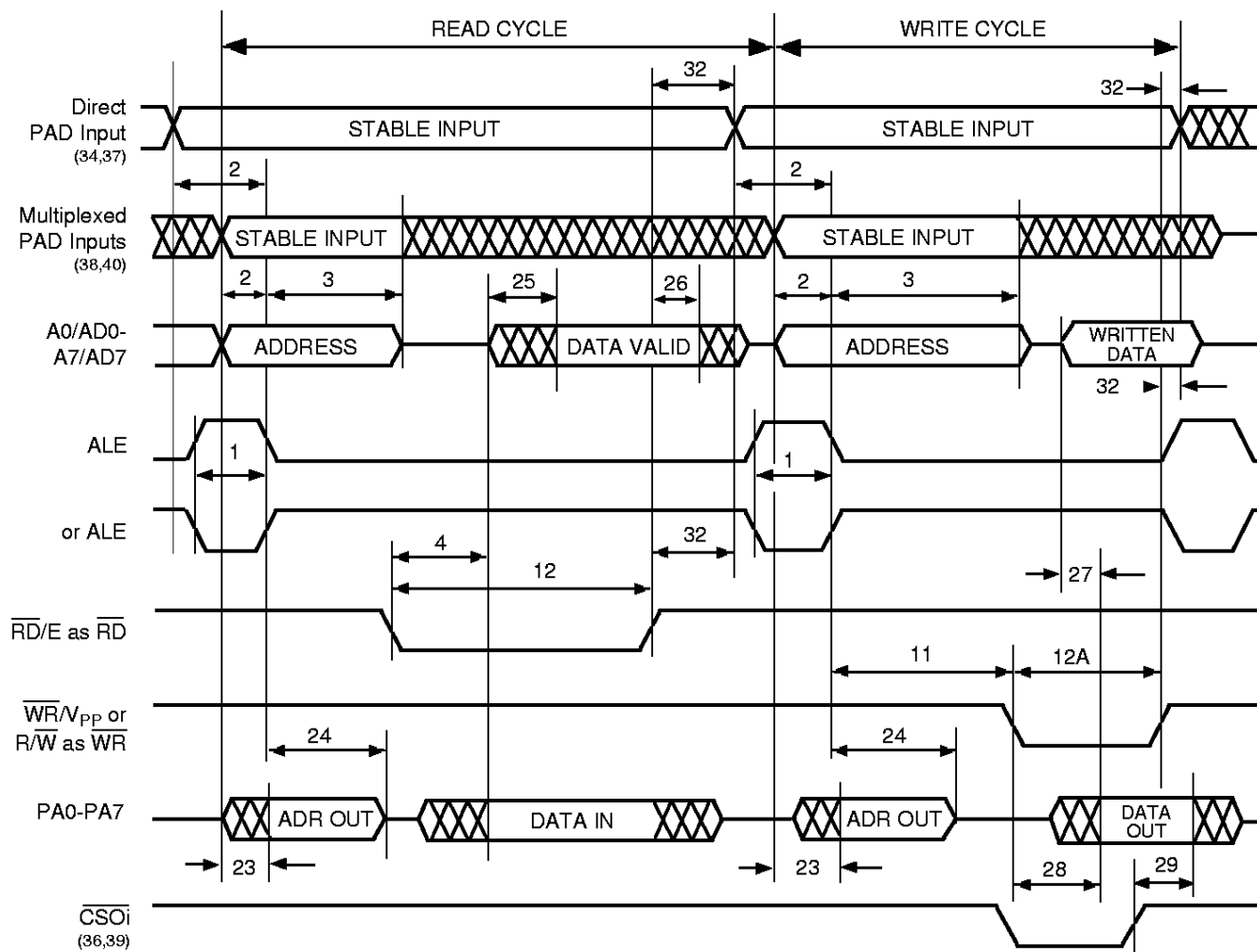
Figure 33. Port A as AD0–AD7 Timing (Track Mode), CRRWR = 0 (PSD3X1)
