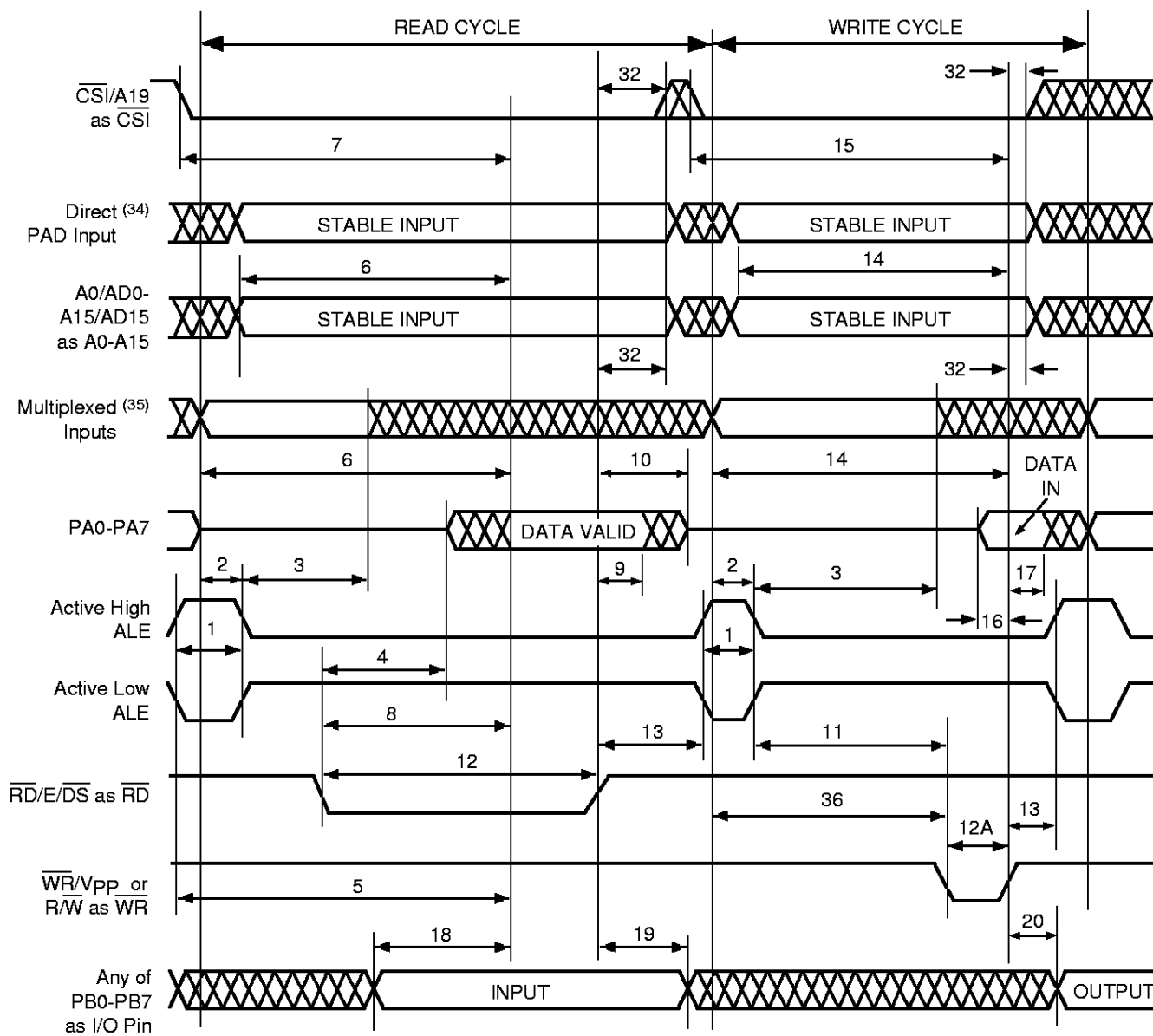
Figure 25. Timing of 8-Bit Non-Multiplexed Address/Data Bus, CRRWR = 0 (PSD3X2/3X3/3X4R)
