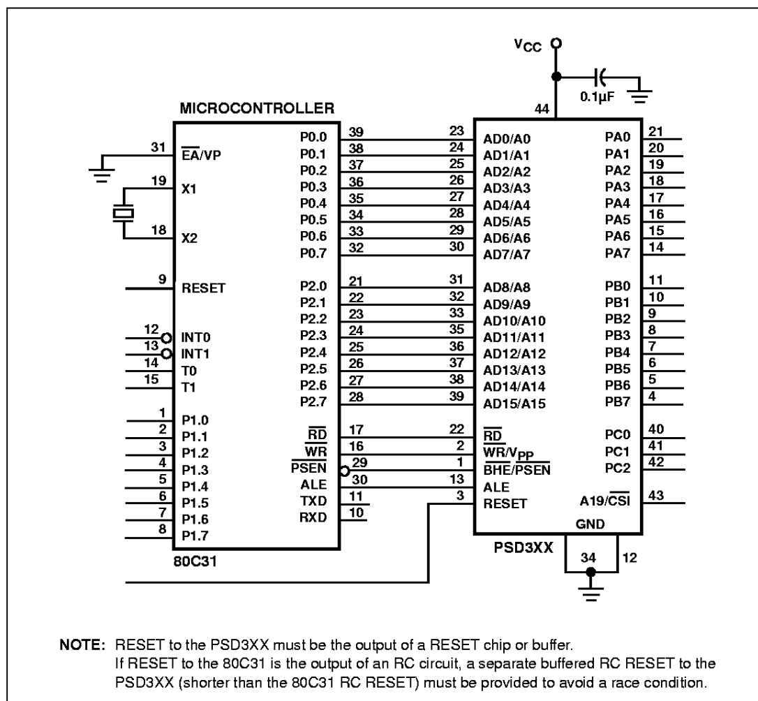
Figure 12. PSD3XX Interface With Intel's 80C31
