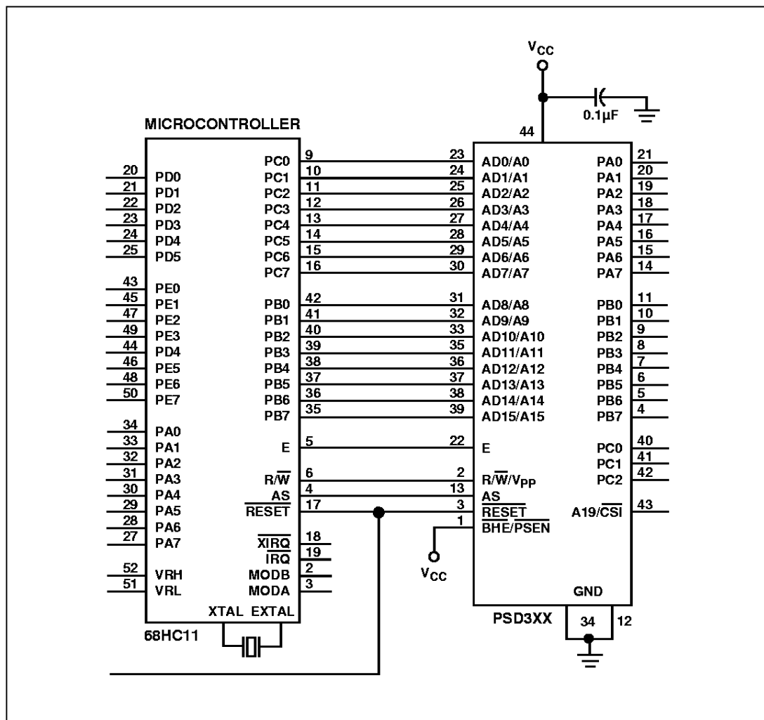
Figure 13. PSD3XX Interface With Motorola's 68HC11
