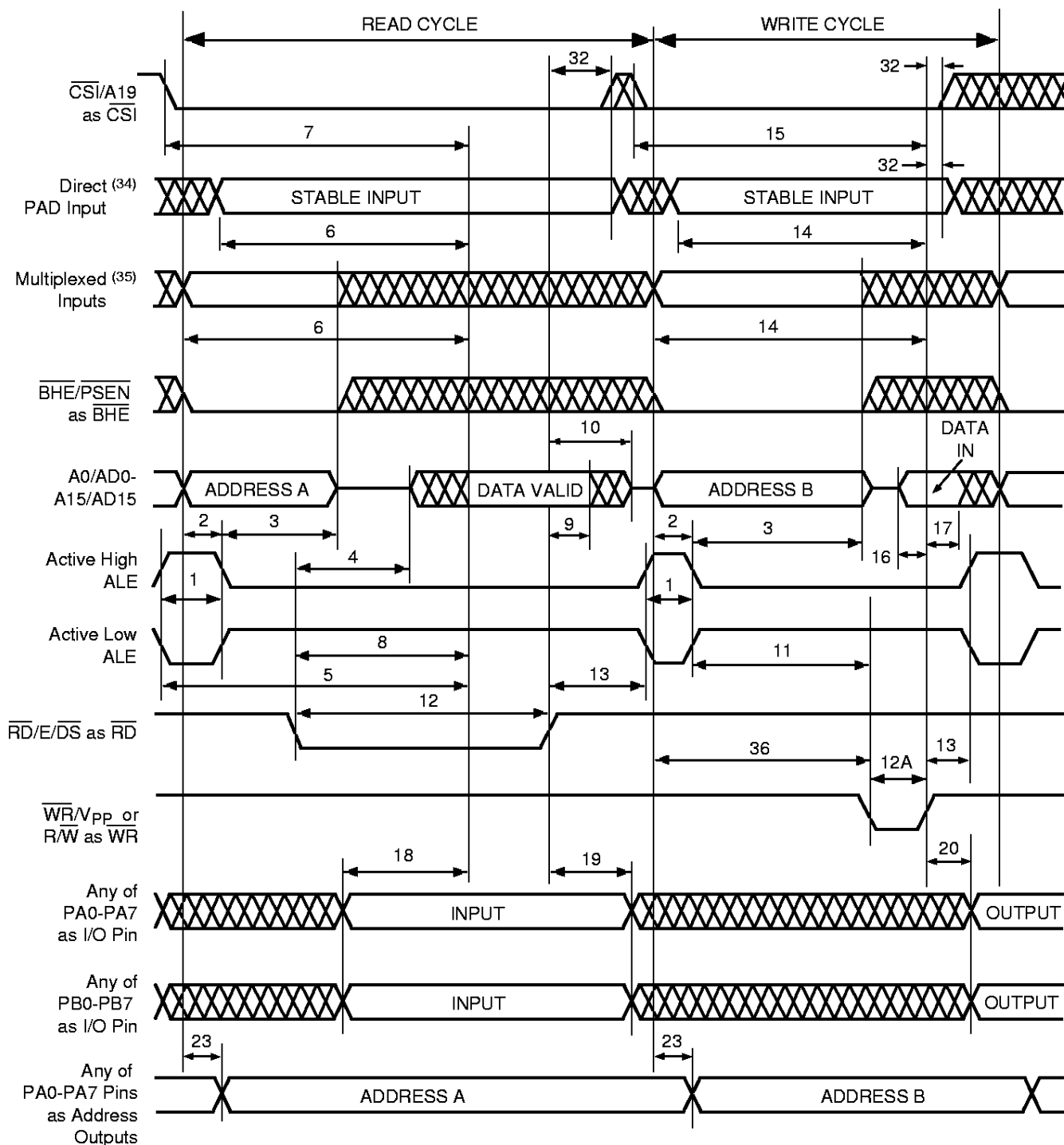
Figure 21. Timing of 16-Bit Multiplexed Address/Data Bus, CRRWR = 0 (PSD3X2/3X3/3X4R)
