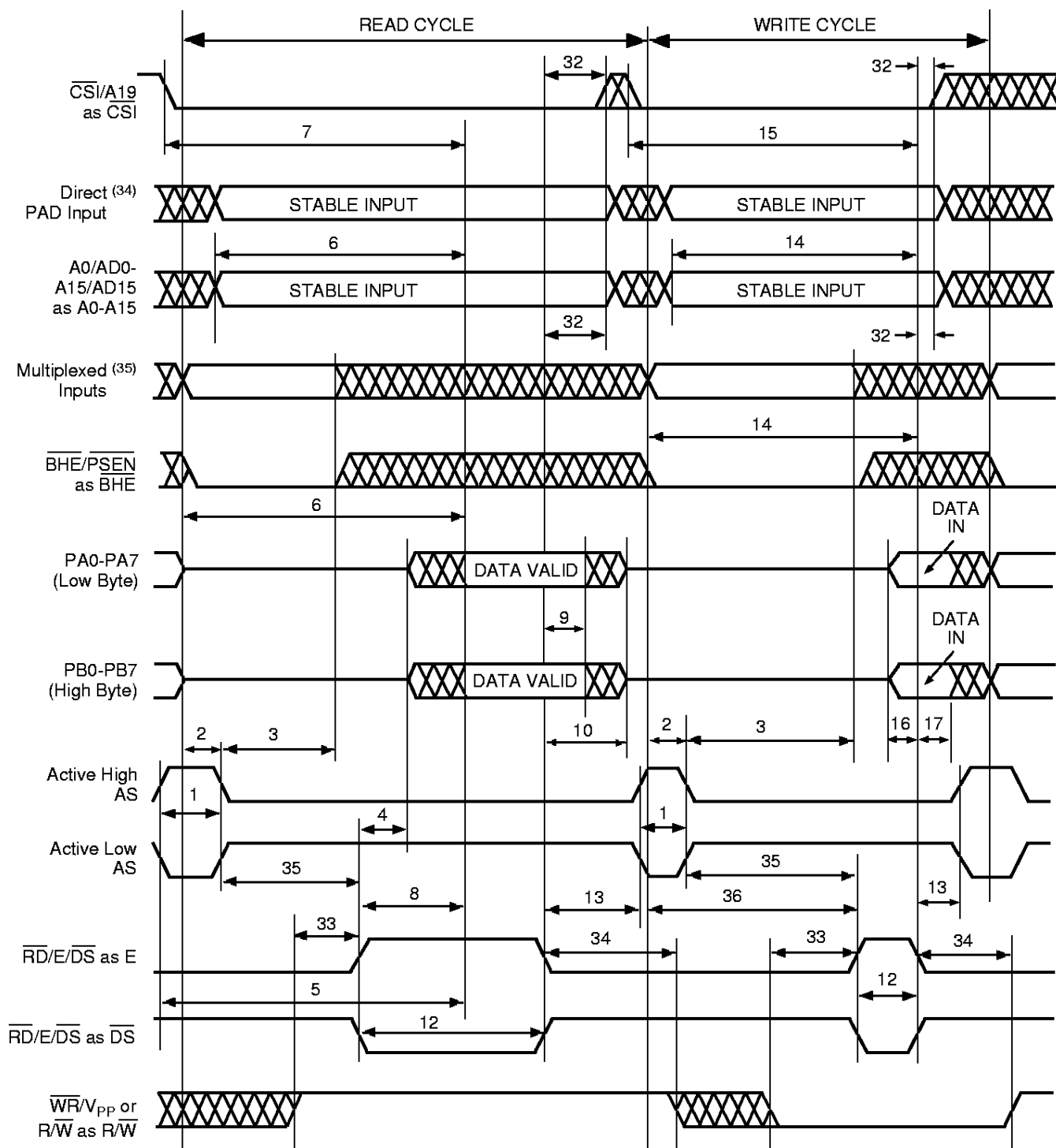
Figure 31. Timing of 16-Bit Non-Multiplexed Address/Data Bus, CRRWR = 1 (PSD3X2/3X3/3X4R)
