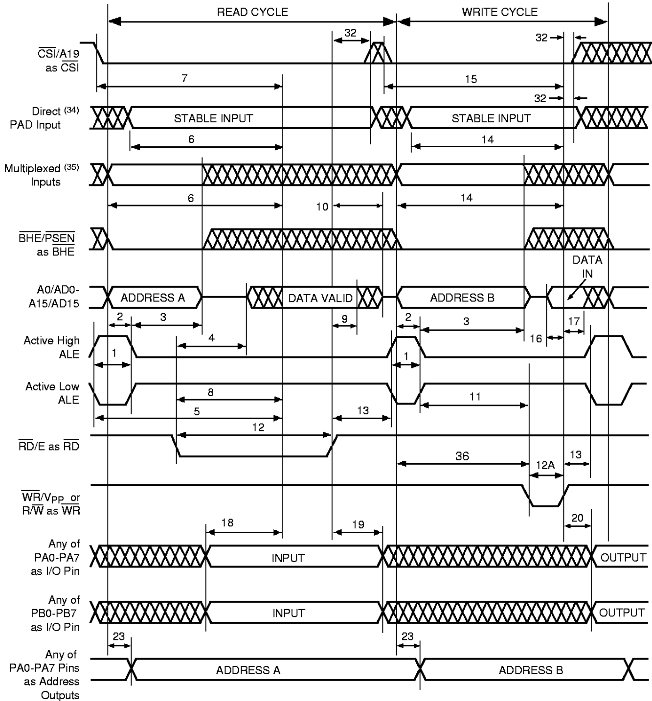
Figure 20. Timing of 16-Bit Multiplexed Address/Data Bus, CRRWR = 0 (PSD3X1)
