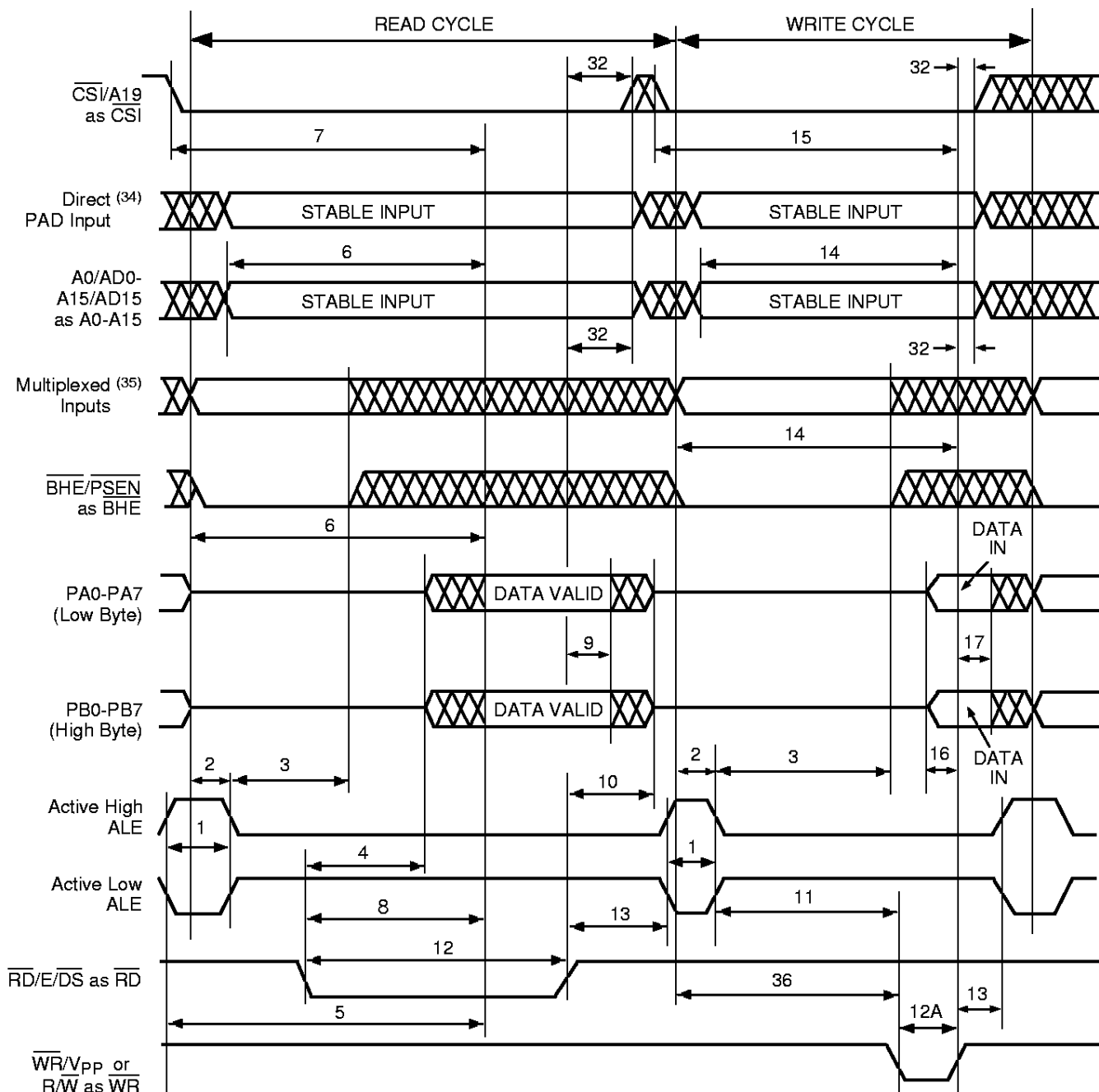
Figure 29. Timing of 16-Bit Non-Multiplexed Address/Data Bus, CRRWR = 0 (PSD3X2/3X3/3X4R)
