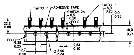
TAPE STYLE T3
