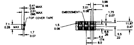
TAPE STYLE SP & RP
