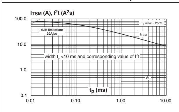
Figure 7. Non-repetitive surge peak on-state current and corresponding value of I^2t sinusoidal pulse width
