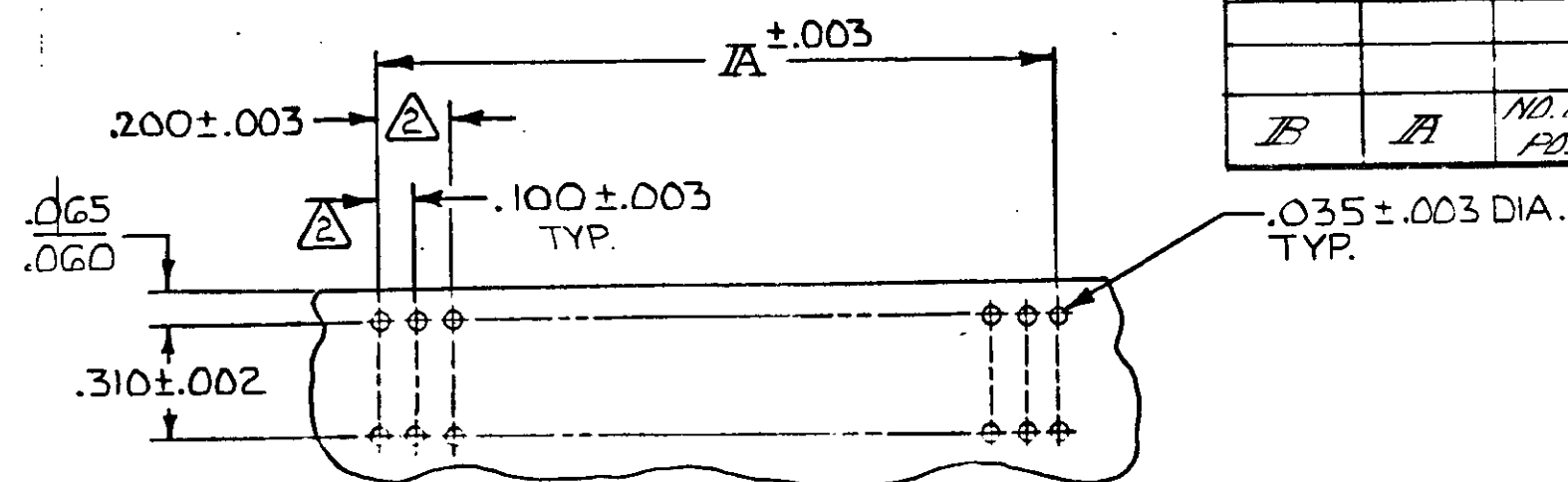
RECOMMENDED P.C. BOARD HOLE LAYOUT
