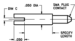
Part No. PPM-0020-CC-YYY-01
