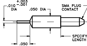
Part No. PPM-0040-06-YYY-01
