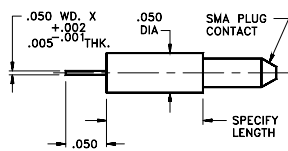
Part No. PPM-0030-05-YYY-01
