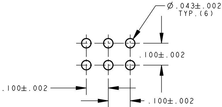
RECOMMENDED HOLE PATTERN GAUGE
