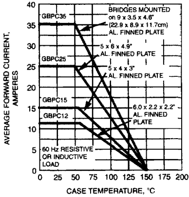
FIG. 1 - MAXIMUM OUTPUT RECTIFIED CURRENT
