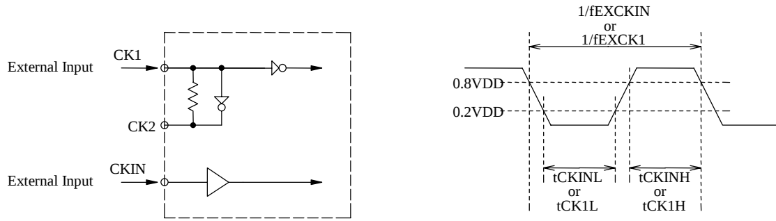
Figure1 External Clock Input
