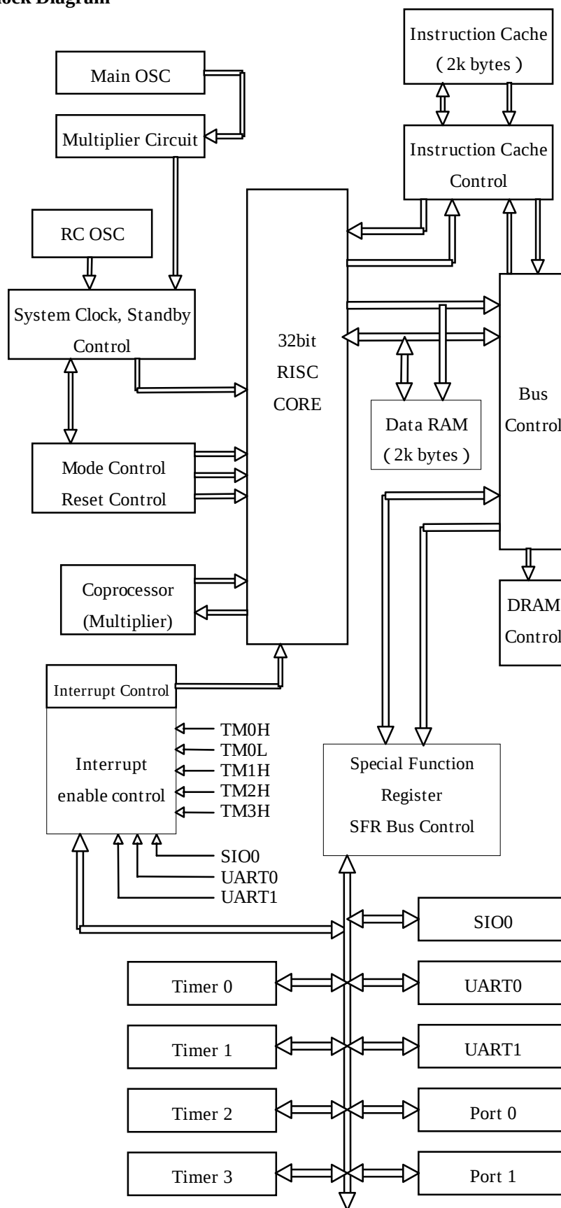
Figure 1 LC680100A System Block Diagram
