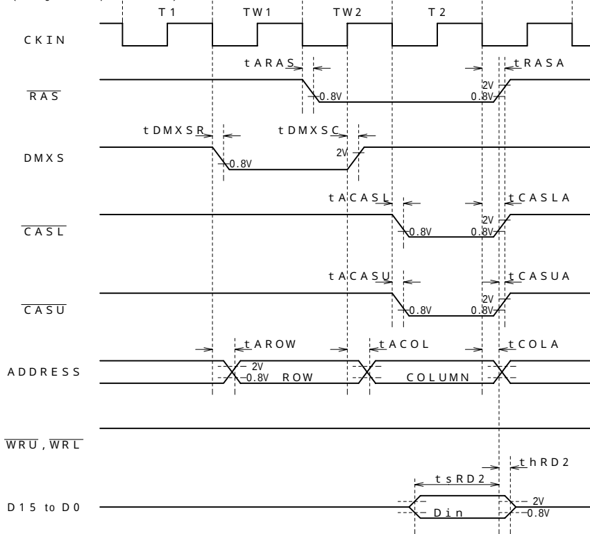
Figure9 DRAM Read Timing
