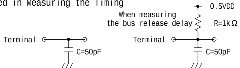
Figure14 The Load Used in Measuring the Timing
