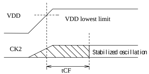
Figure3 Oscillation Stabilizing Time
