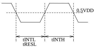
Figure4 External Pulse Input
