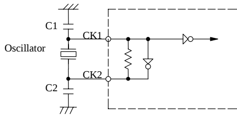
Figure2 Ceramic Oscillation
