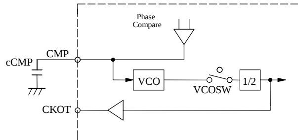
Figure5 VCO
