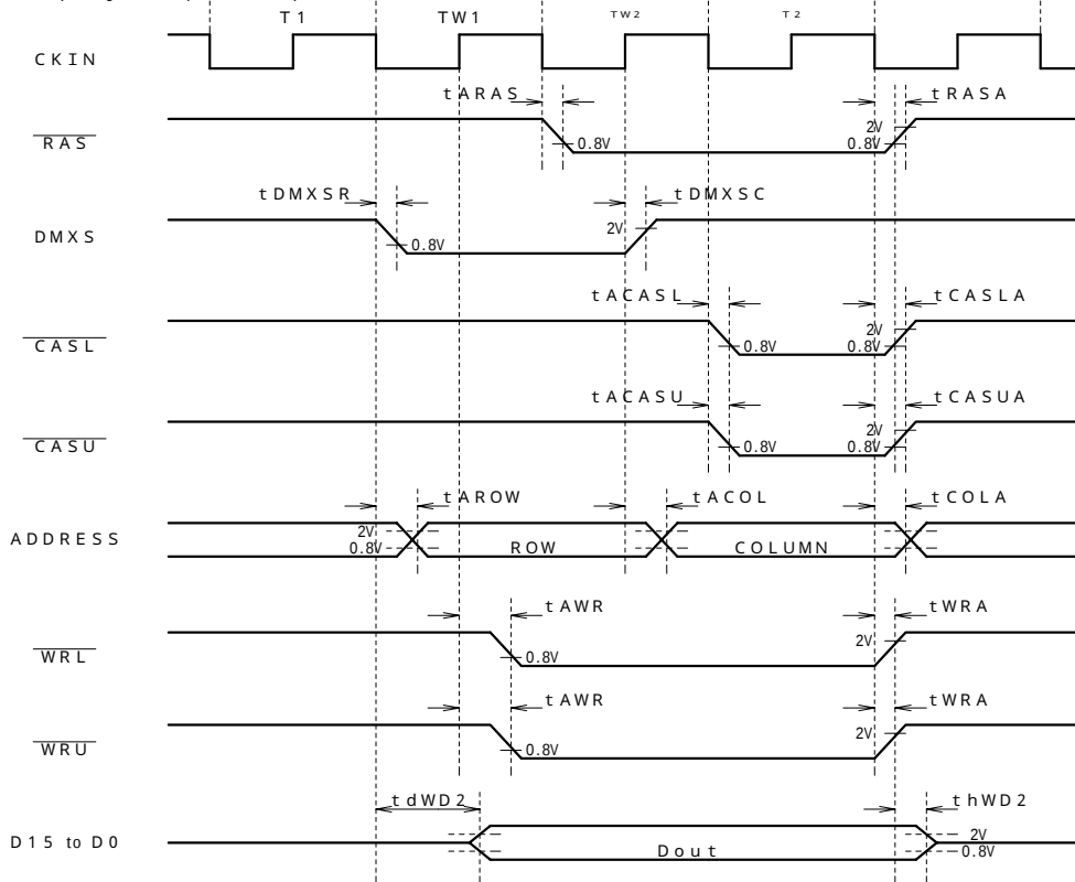
Figure10 DRAM Write Timing
