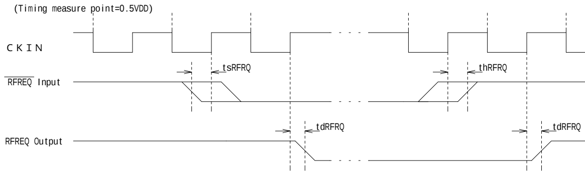
Figure11 RFREQ Input/Output Timing
