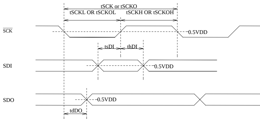
Figure6 Serial Input/Output Timing
