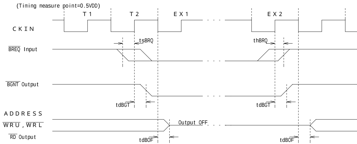
Figure12 Bus Request/Release Timing
