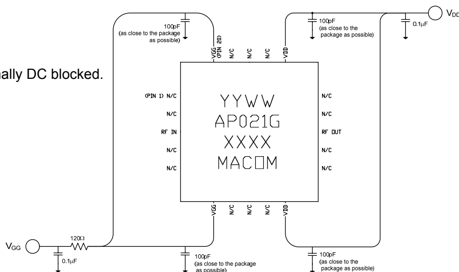
Figure 28. Recommended Bias Configuration.
