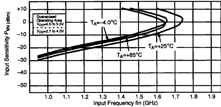
Input Sensitivity vs. Input Frequency (Temperature Dependence)
