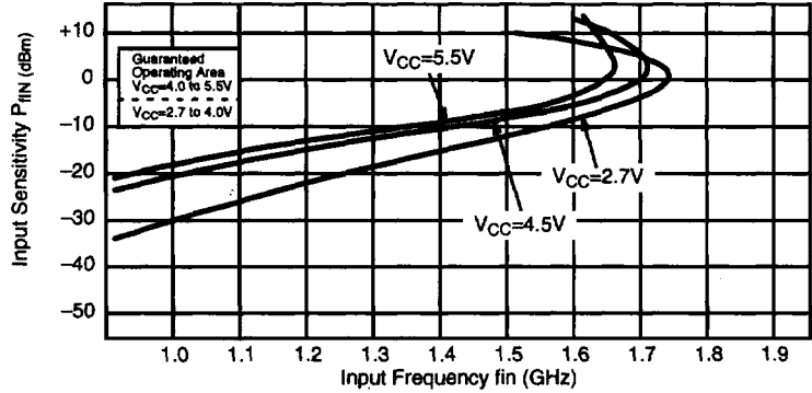
Input Sensitivity vs. Input Frequency (Supply Voltage Dependence)
