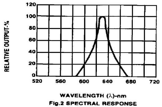
Fig.2 SPECTRAL RESPONSE
