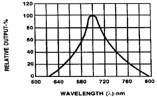
Fig.2 SPECTRAL RESPONSE
