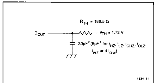
Figure 2. Thevenin Equivalent
