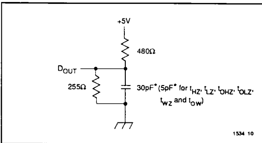
Figure 1. Output Load
