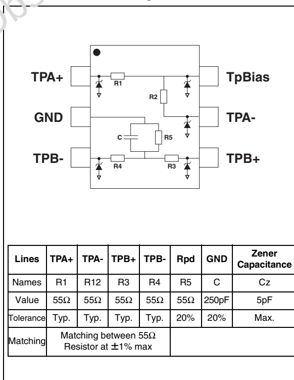
Figure 1: Pinout Configuration
