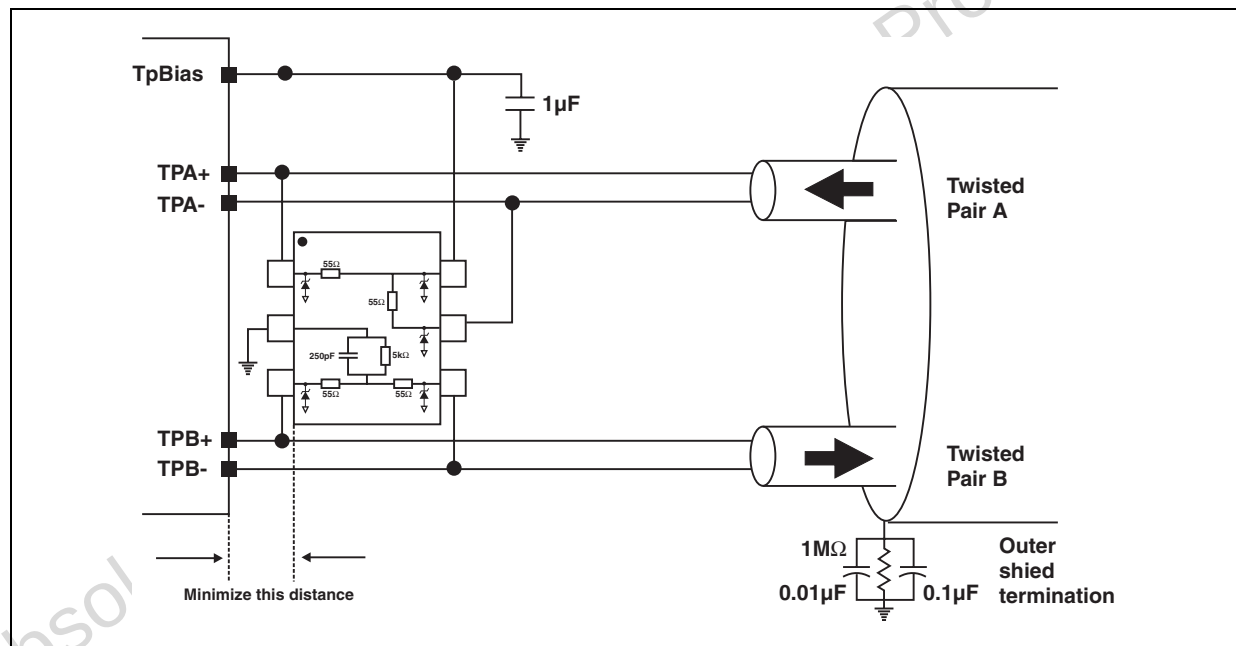
Figure 2: Functionnal Diagram
