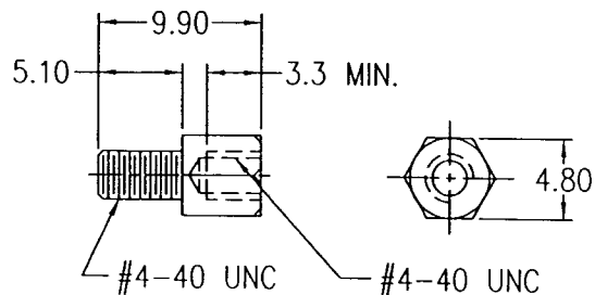
FEMALE SCREWLOCK (SEE ORDERING DATA LEGEND)
