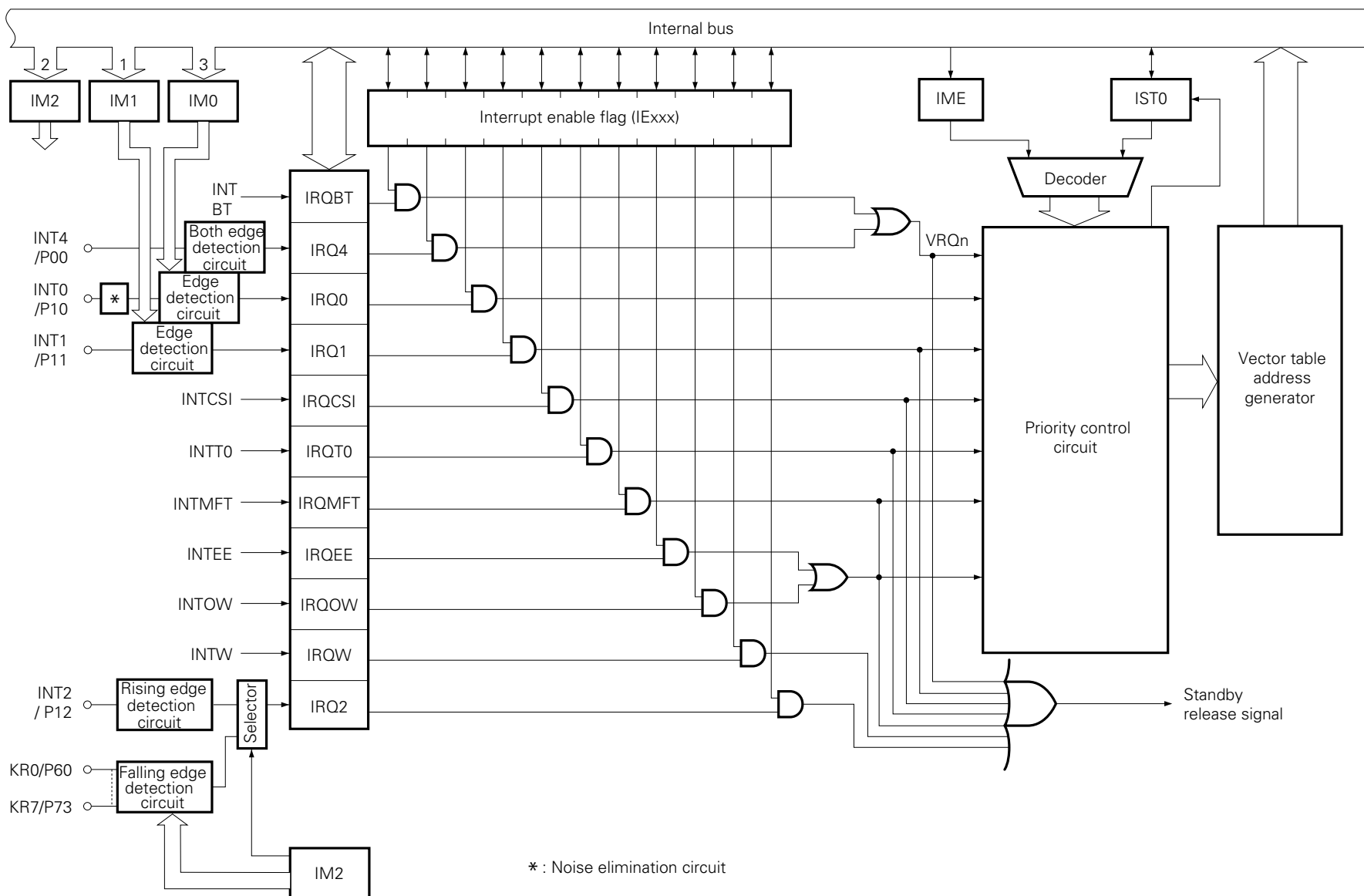
Fig. 7-1 Interrupt Control Circuit Block Diagram
