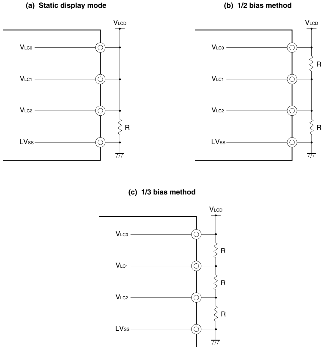
Figure 17-29. Examples of LCD Drive Power Connections (External Resistance Division Method)
