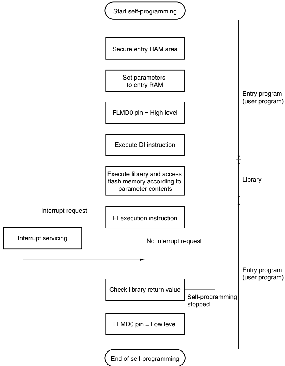
Figure 26-18. Self-Programming Procedure
