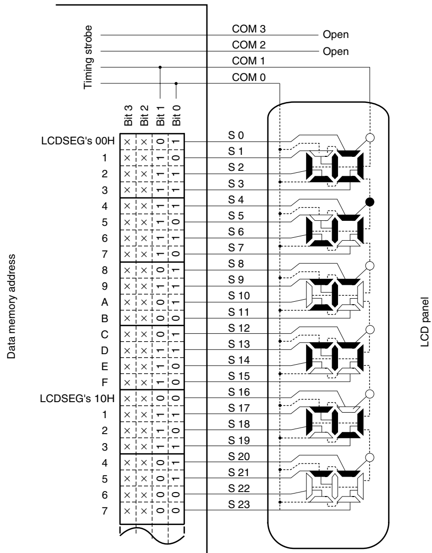
Figure 17-19. Example of Connecting Two-Time-Slice LCD Panel
