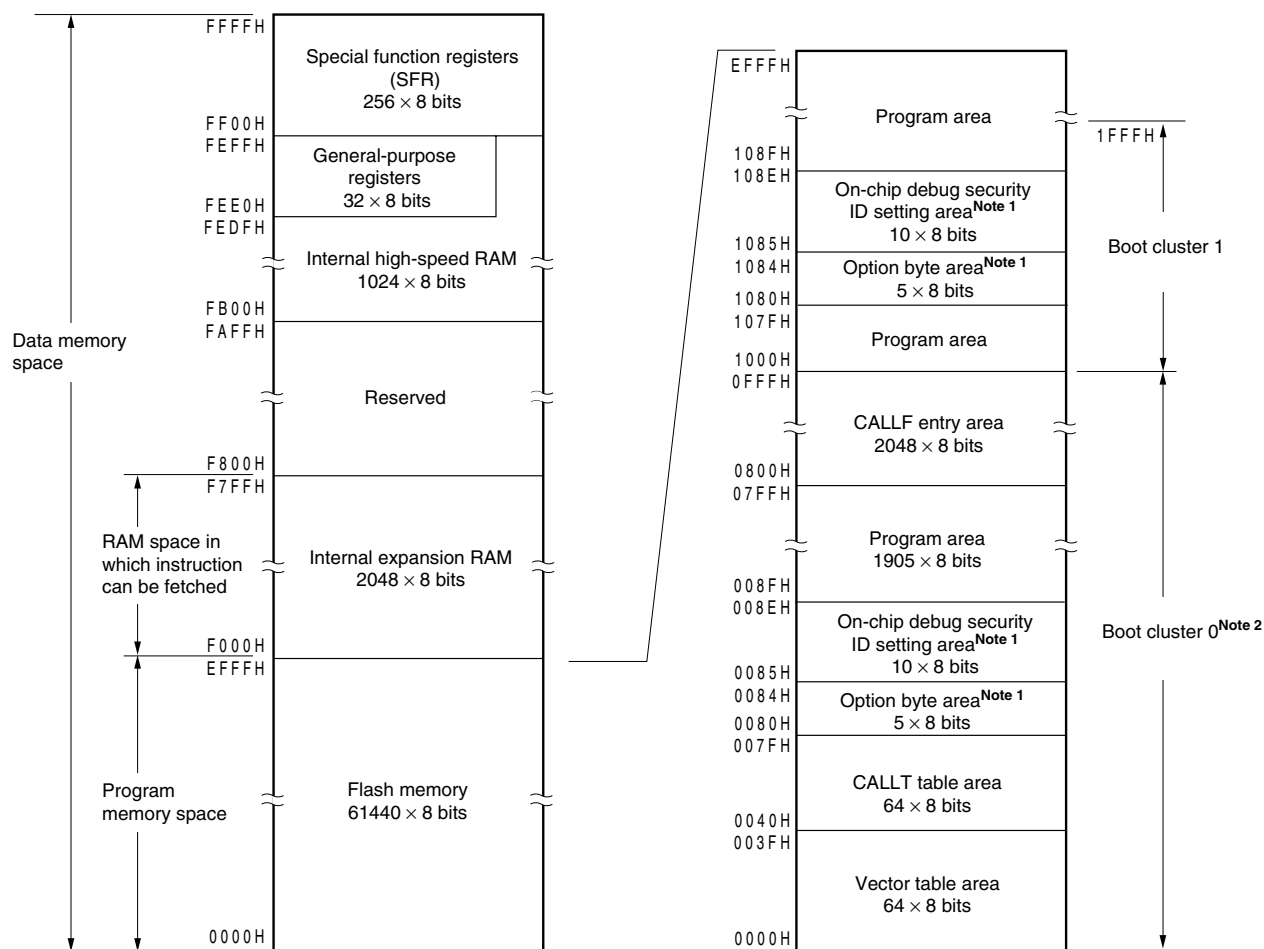
Figure 3-4. Memory Map ( \mu PD78F0375D, 78F0385D)
