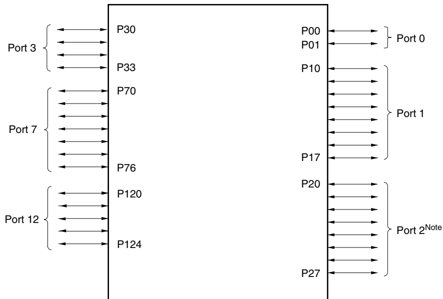
Figure 4-1. Port Types
