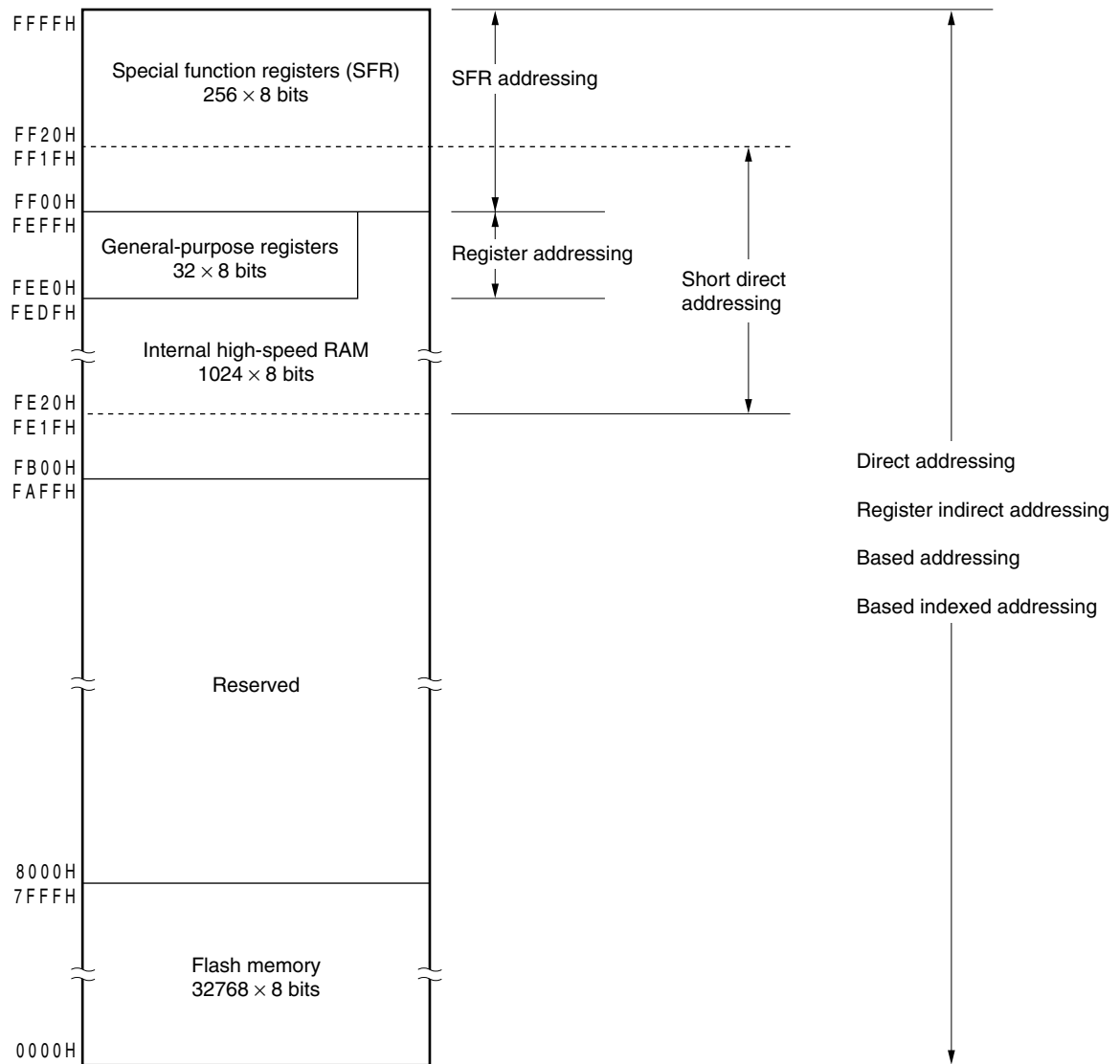
Figure 3-6. Correspondence Between Data Memory and Addressing ( \mu PD78F0373, 78F0383)
