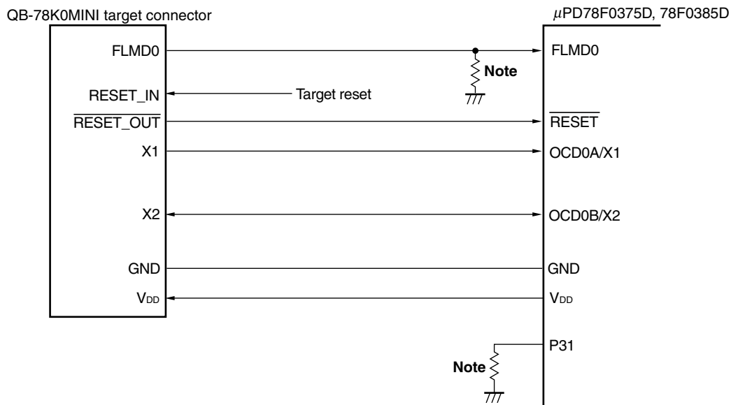
Figure 27-1. Connection Example of QB-78K0MINI and \mu PD78F0375D and 78F0385D (When OCD0A/X1 and OCD0B/X2 Are Used)
