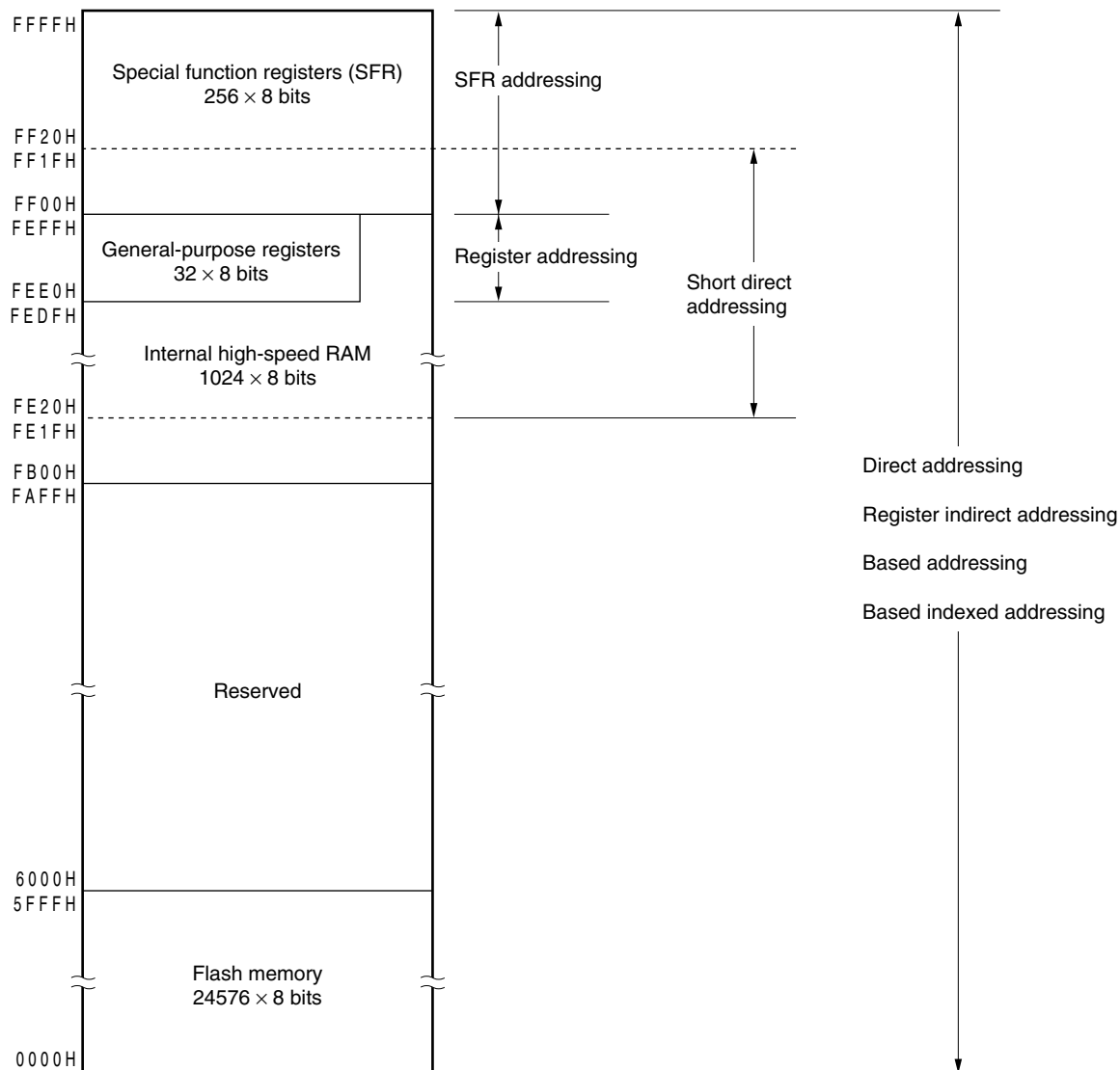
Figure 3-5. Correspondence Between Data Memory and Addressing ( \mu PD78F0372, 78F0382)
