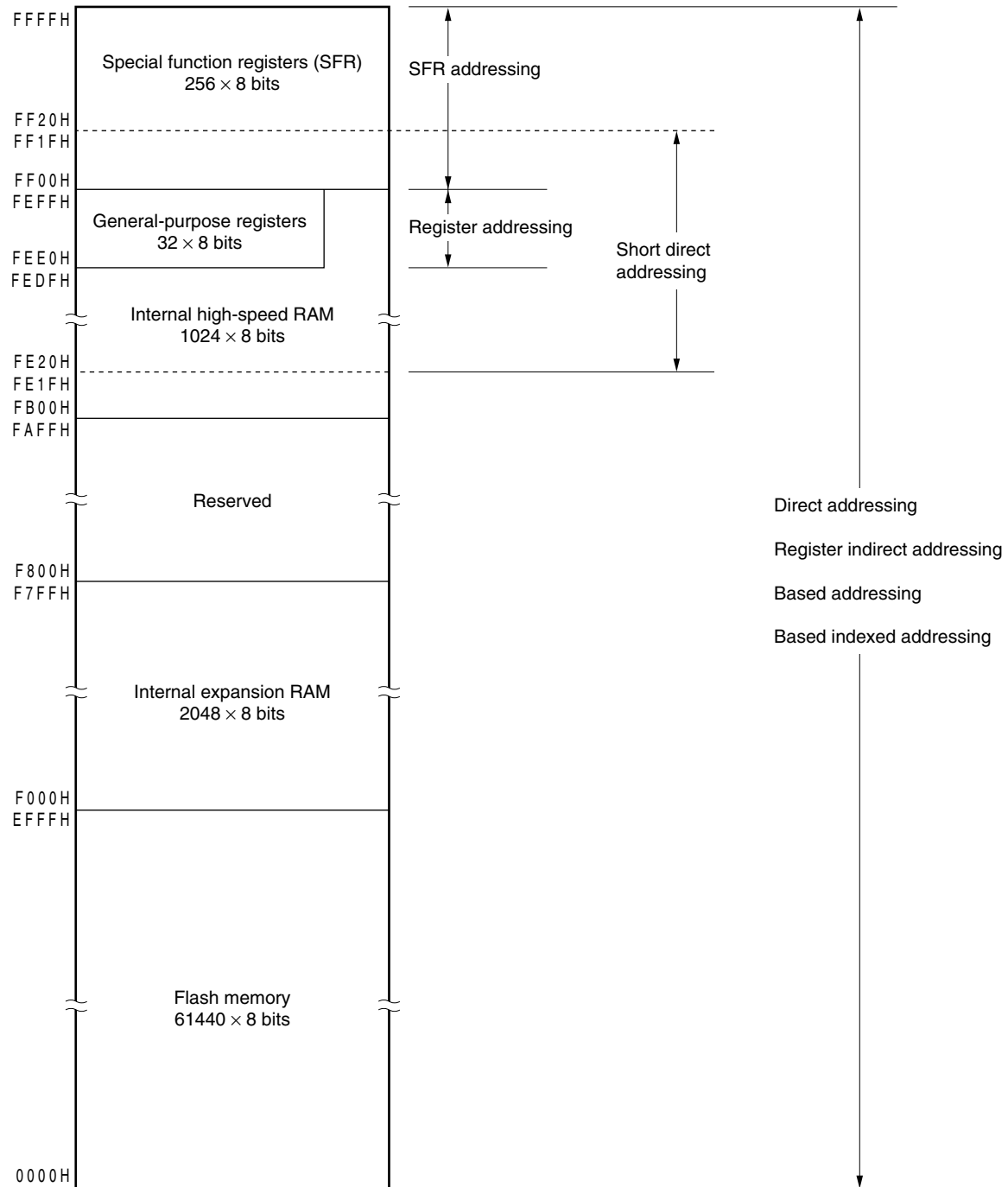
Figure 3-7. Correspondence Between Data Memory and Addressing (μPD78F0375, 78F0375D, 78F0385, 78F0385D)
