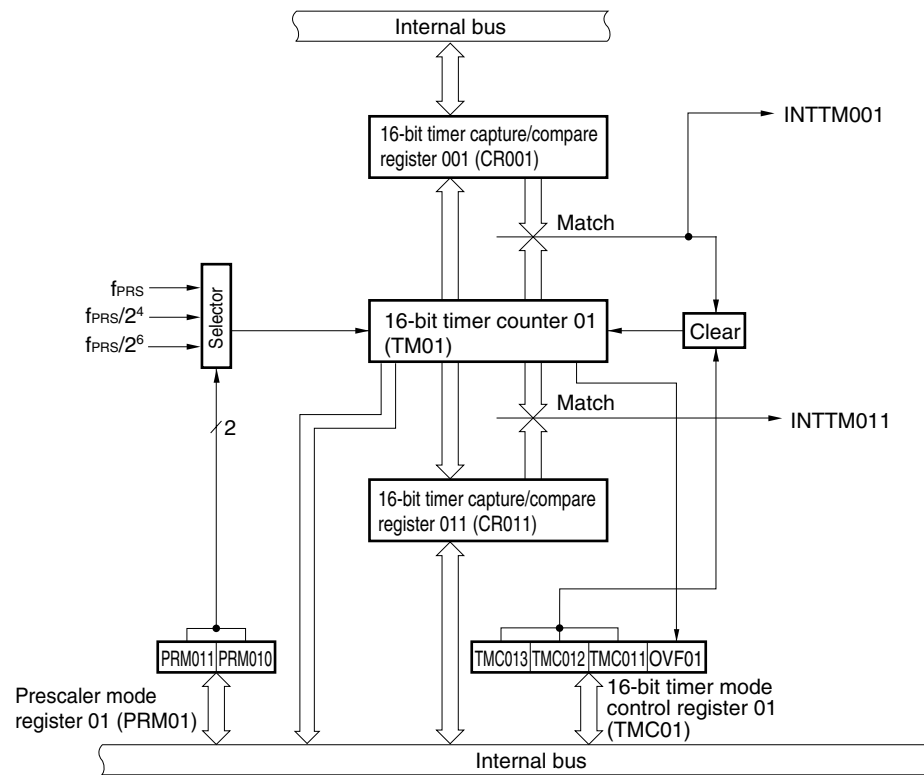
Figure 6-2. Block Diagram of 16-Bit Timer/Event Counter 01 (μPD78F0375, 78F0375D, 78F0385, and 78F0385D Only)
