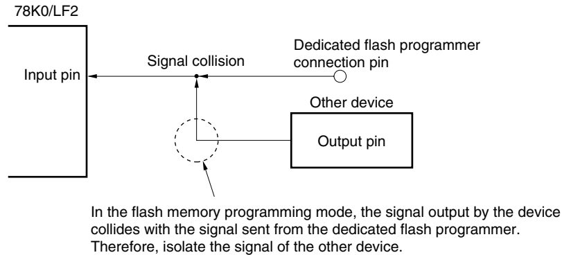
Figure 26-11. Signal Collision (Input Pin of Serial Interface)
