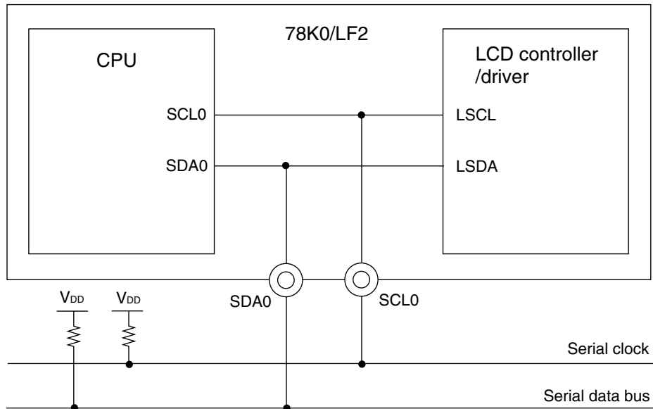
Figure 16-29. System configuration
