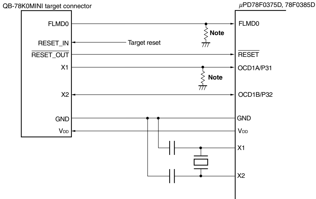
Figure 27-2. Connection Example of QB-78K0MINI and \mu PD78F0375D and 78F0385D (When OCD1A and OCD1B Are Used)
