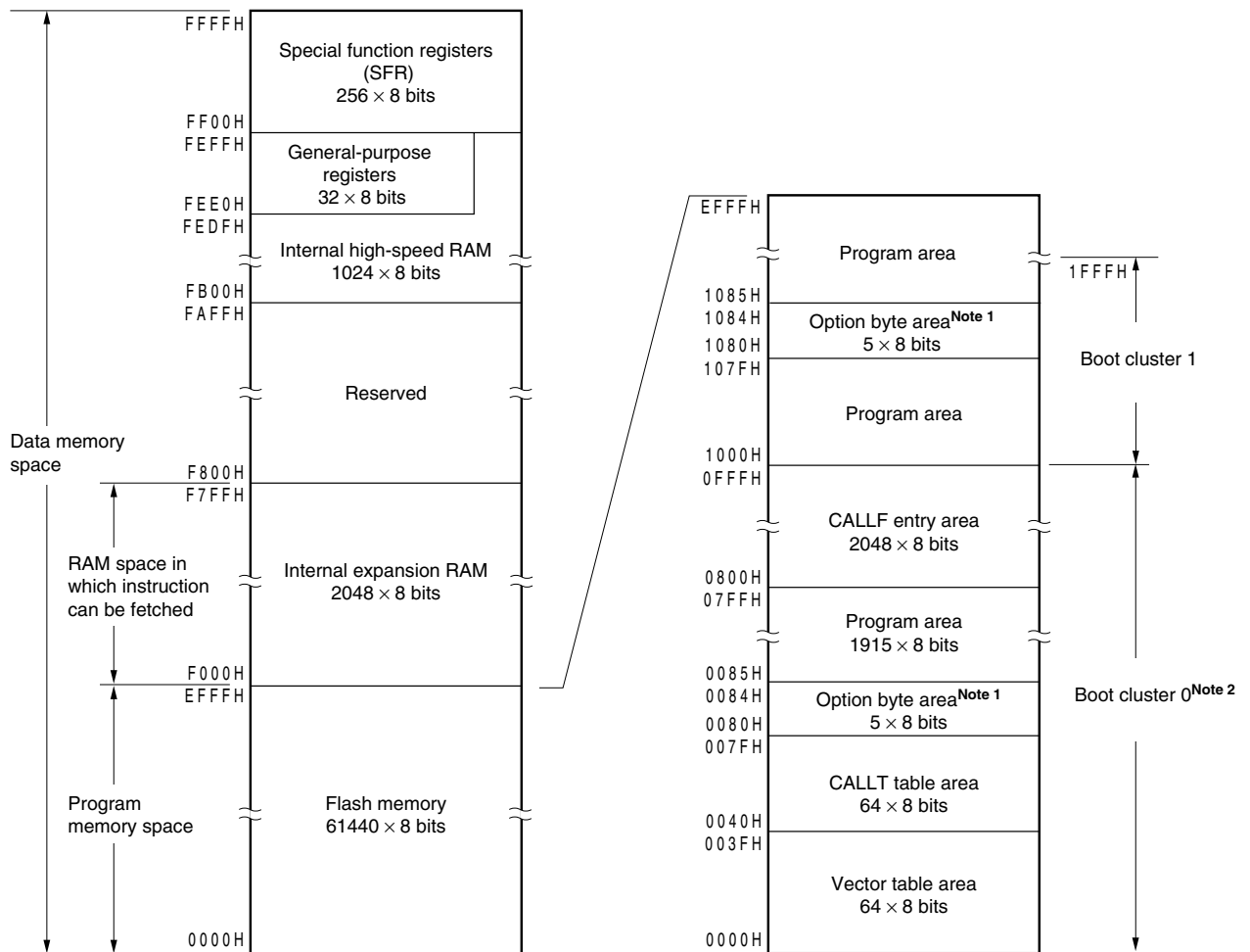
Figure 3-3. Memory Map ( \mu PD78F0375, 78F0385)
