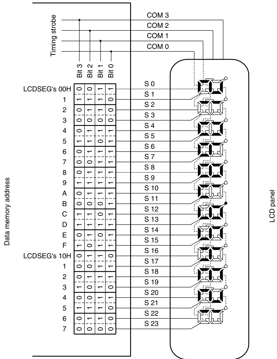
Figure 17-26. Example of Connecting Four-Time-Slice LCD Panel
