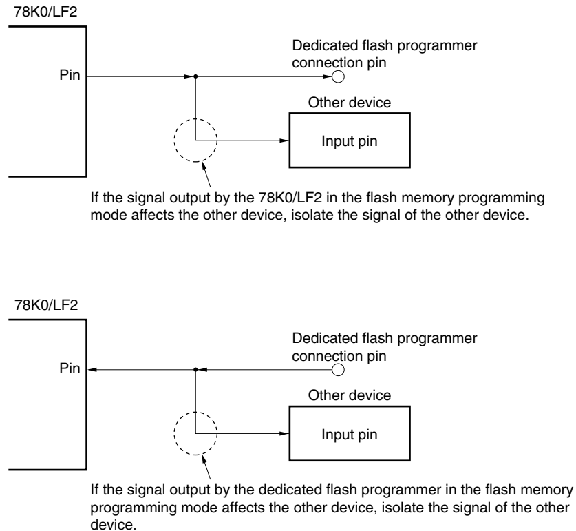
Figure 26-12. Malfunction of Other Device
