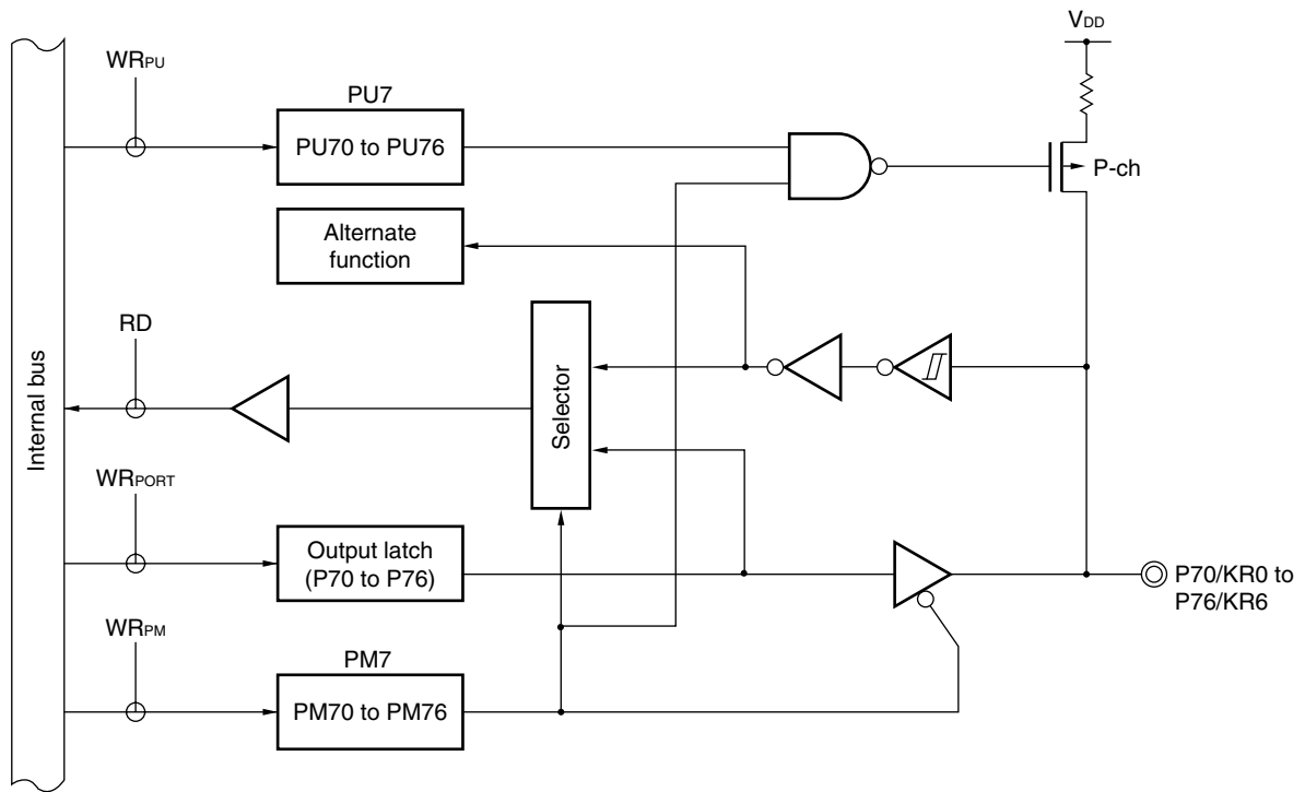
Figure 4-12. Block Diagram of P70 to P76
