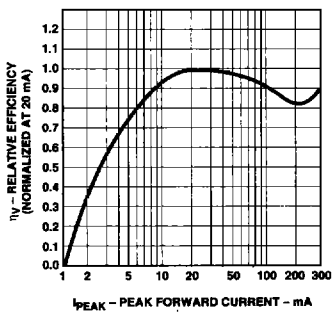
Figure 11. Relative Efficiency vs. Peak Forward Current.
