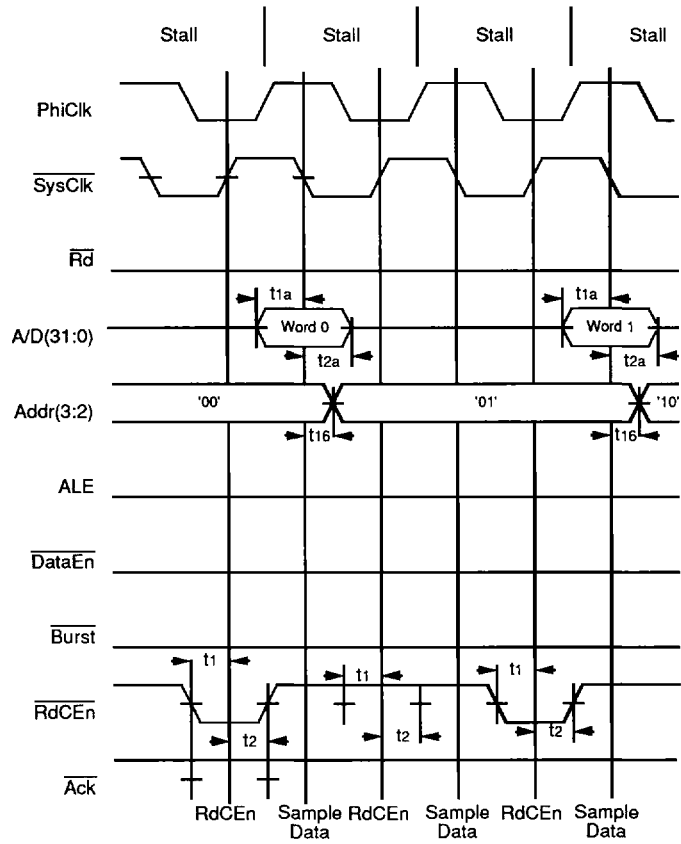
Figure 14 (a). Start of Throttled Quad Read
