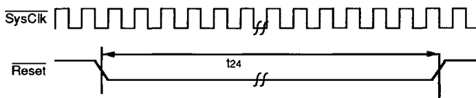
Figure 10. Warm Reset Sequence
