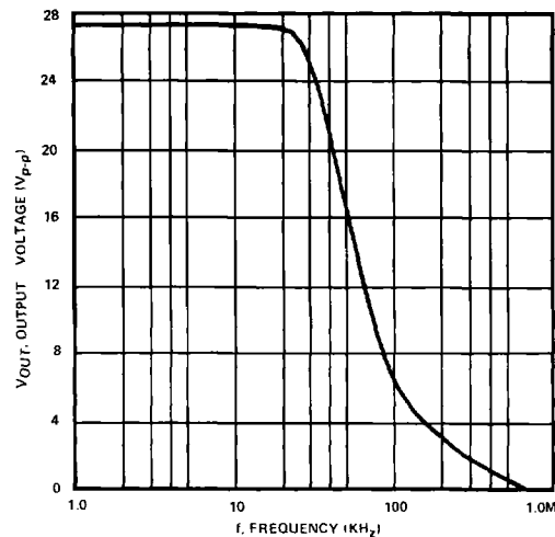
POWER BANDWIDTH
