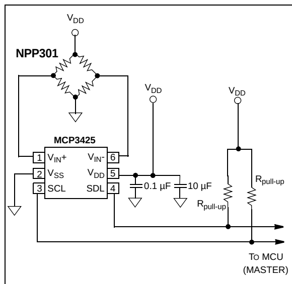
FIGURE 6-6: Example of Pressure Measurement.
