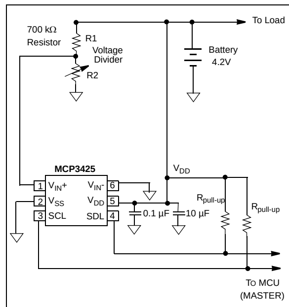
FIGURE 6-5: Example of Battery Voltage Measurement.
