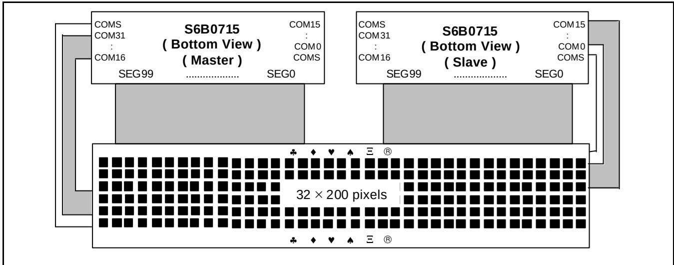
Figure 46. SHL = 0, ADC = 1
