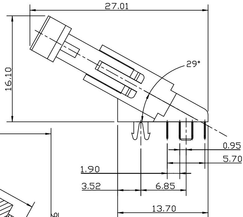
SIDE VIEW SCALE 3.000
