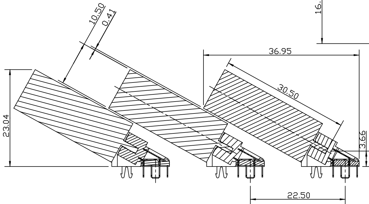
SECTION H-H (WITH MODULE CARD)
