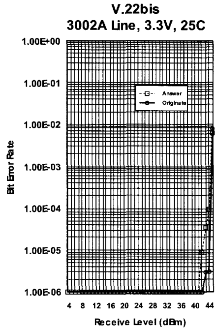
BER VS RECEIVE LEVEL
