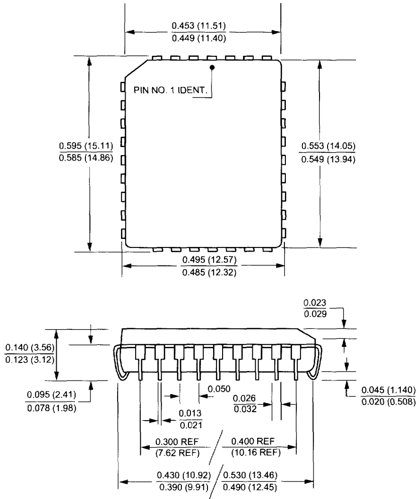
32-Pin PLCC
