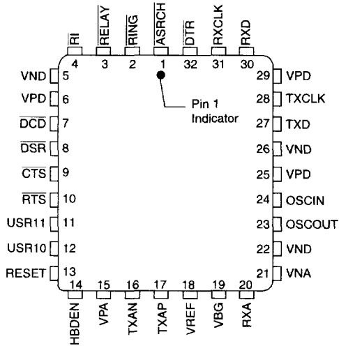
32-Lead PLCC 73M2901-32IH/3
