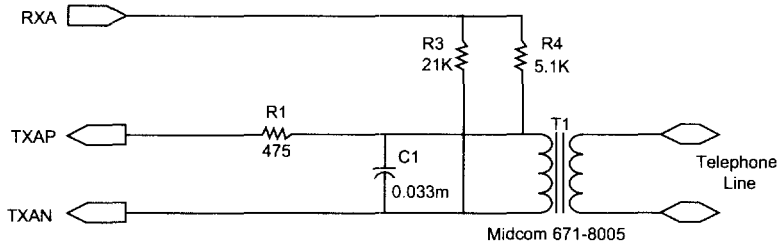
Recommended Line Interface
