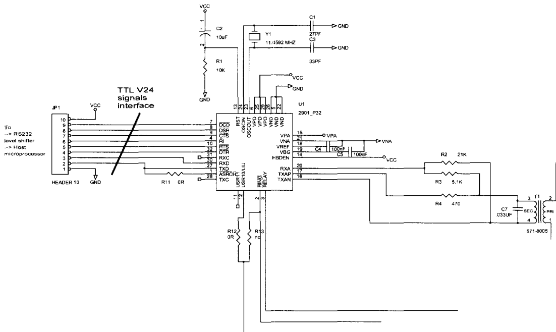
Recommended Schematics Arrangement
