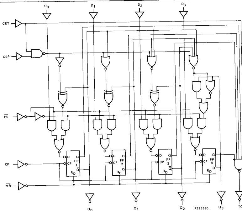
Fig. 7 Logic diagram.
