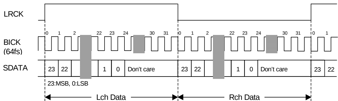
Figure 3. Mode 2 Timing
