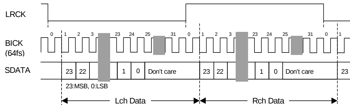
Figure 4. Mode 3 Timing
