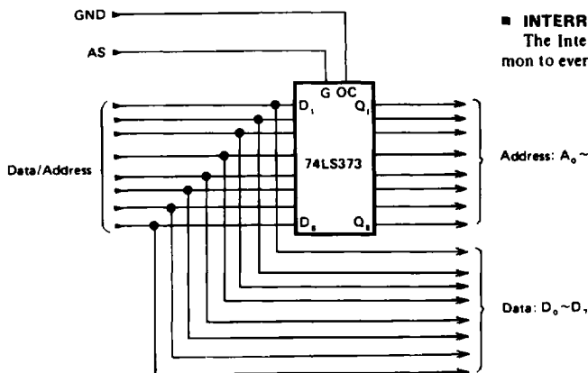
Figure 11 Latch Connection
