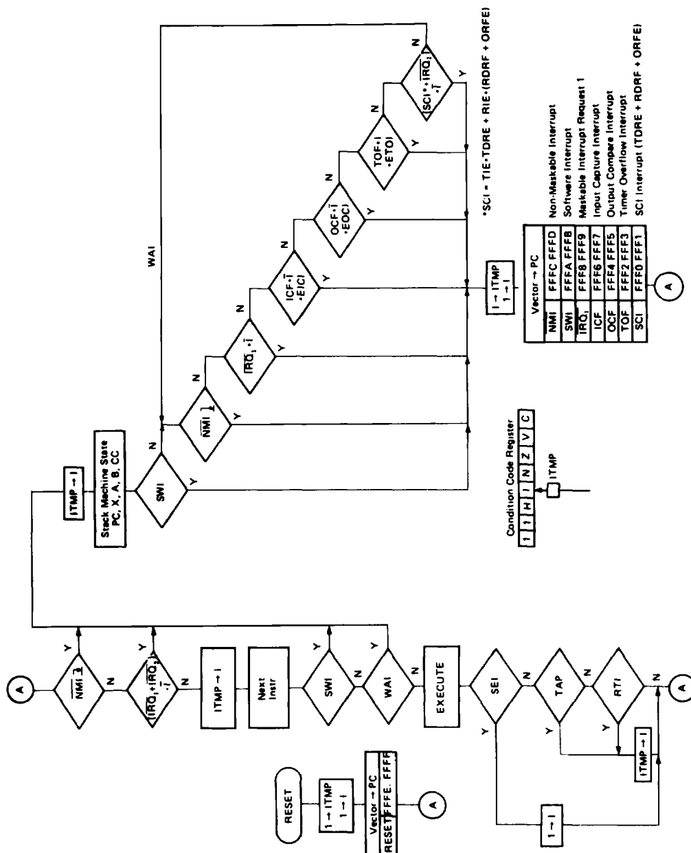
Figure 16 Interrupt Flowchart
