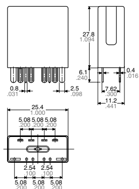
External dimensions
