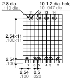
PC board pattern
