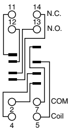
Schematic
