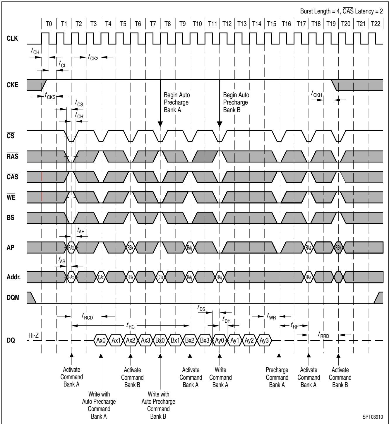
Figure 17 AC Parameters for a Write Timing
