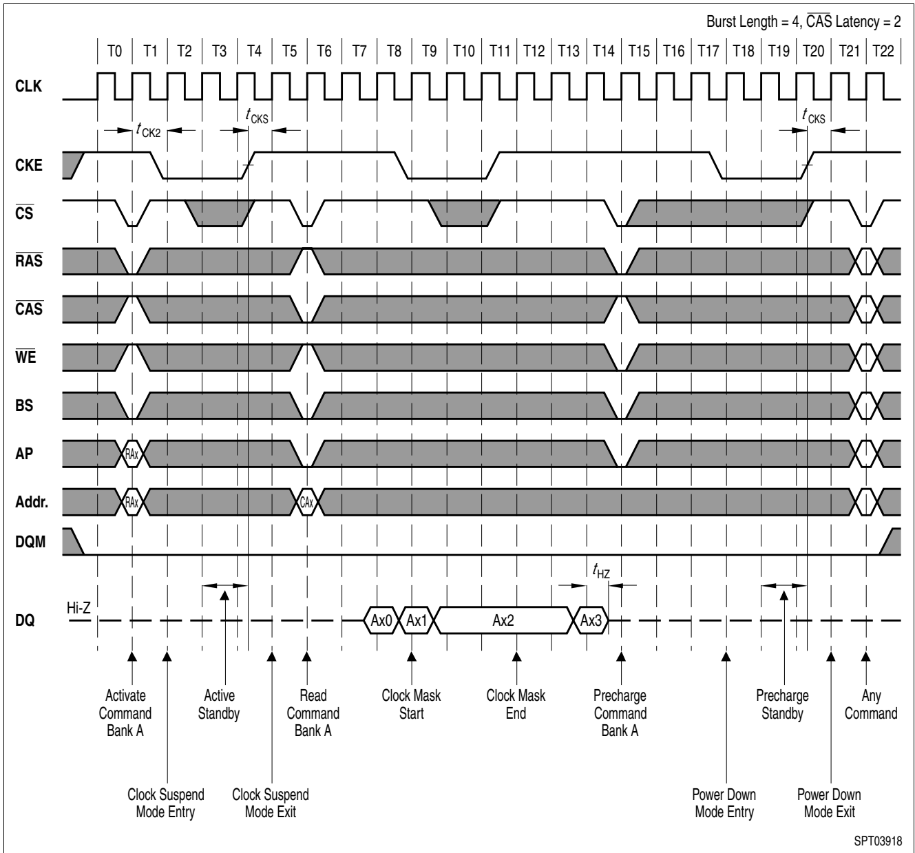
Figure 25 Power Down Mode and Clock Suspend
