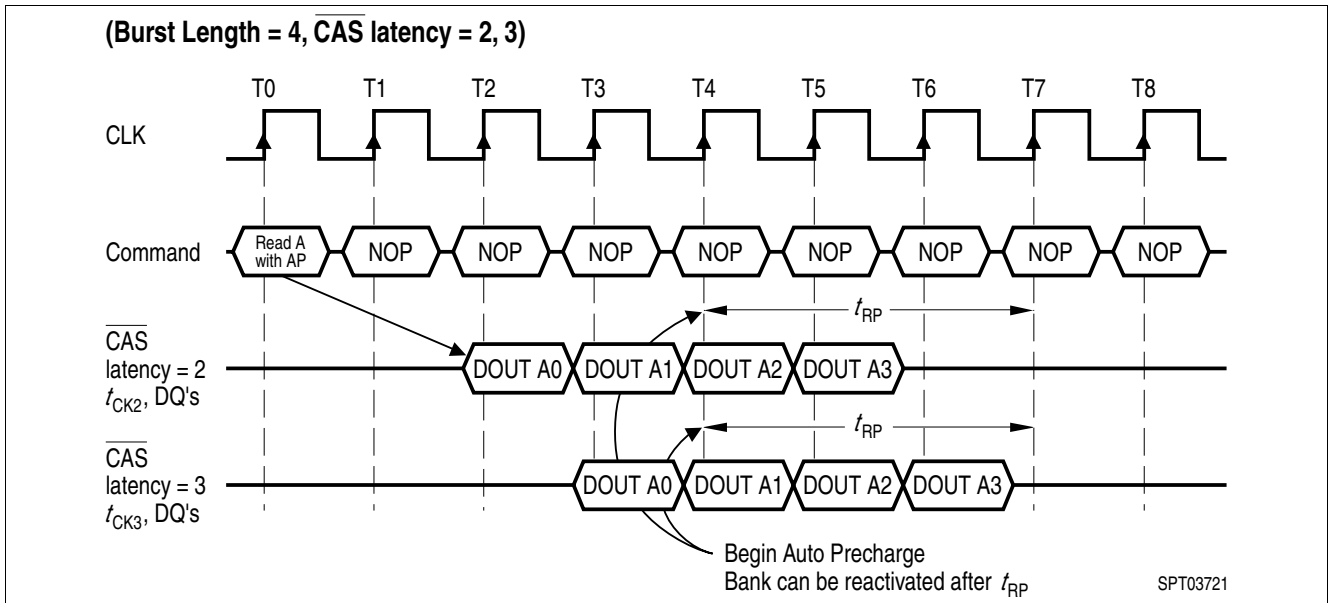
Figure 16 Burst Read with Auto-Precharge
