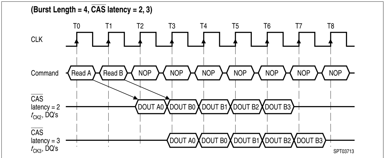
Figure 8 Read Interrupted by a Read
