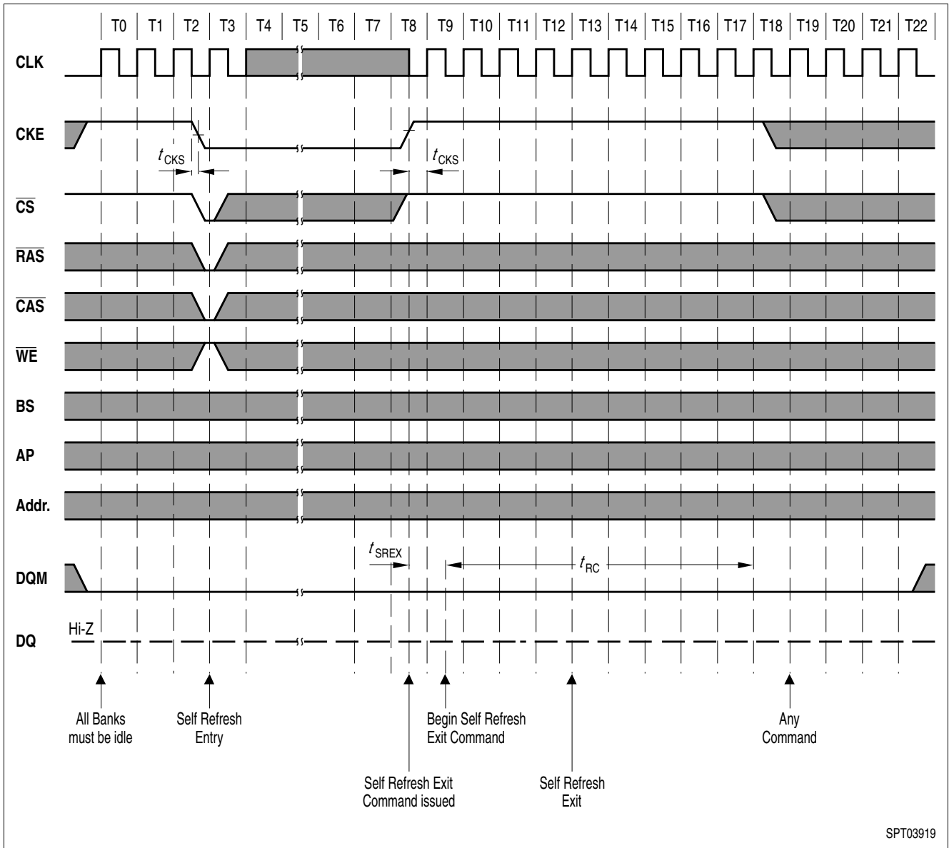
Figure 26 Self Refresh (Entry and Exit)
