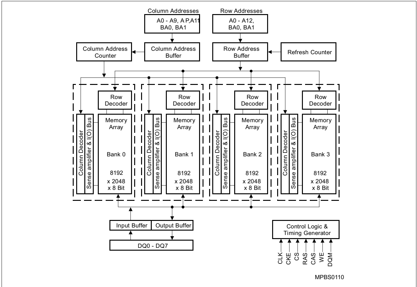
Figure 3 Block Diagram for 64M x 8 SDRAM (13/11/2 Addressing)
