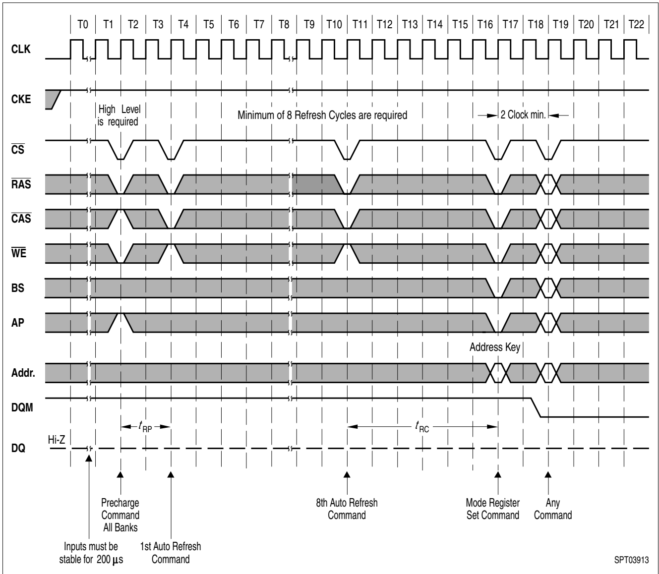
Figure 20 Power on Sequence and Auto Refresh (CBR)
