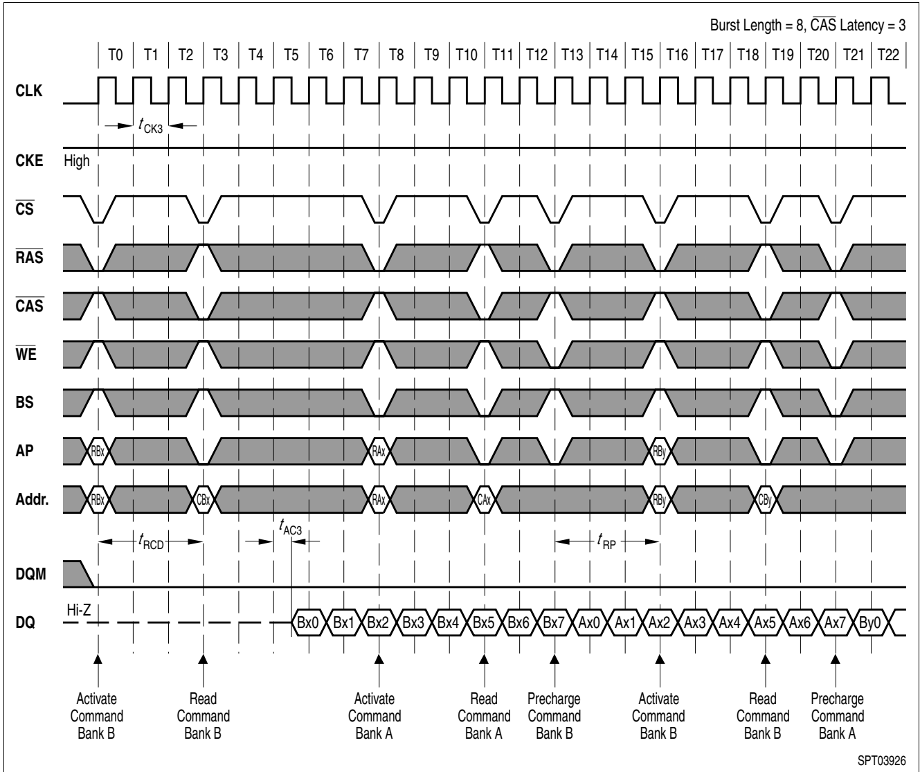
Figure 33 CAS Latency = 3
