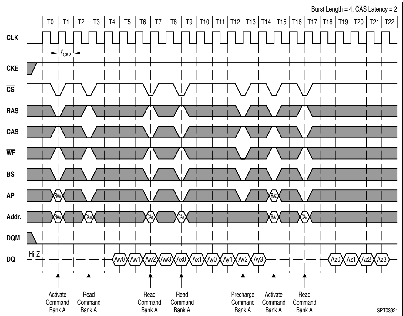
Figure 28 CAS Latency = 2
