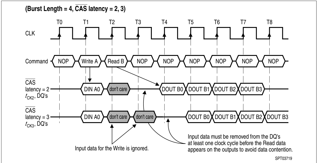
Figure 14 Write Interrupted by a Read
