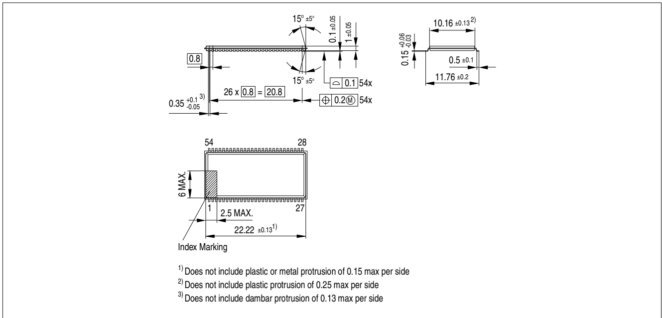
Figure 39 Package Outline P-TSOPII-54-1 (top view)
