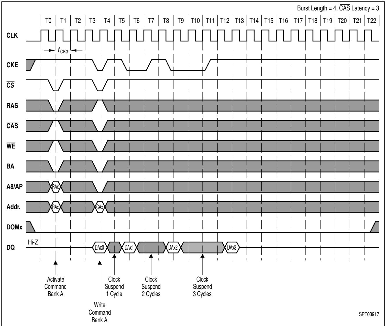
Figure 24 Clock Suspension During Burst Write CAS Latency = 3
