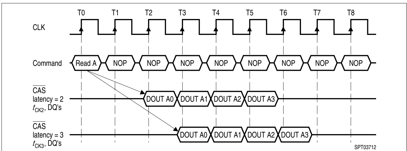
Figure 7 Burst Read Operation
