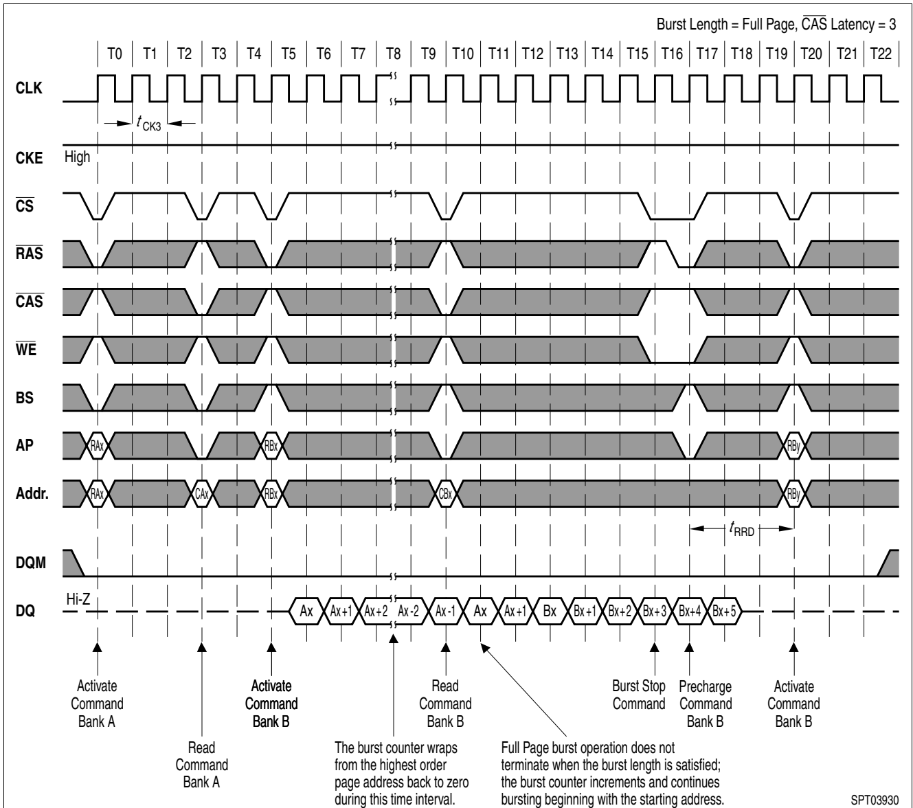
Figure 38 Full Page Burst Write, CAS Latency = 3
