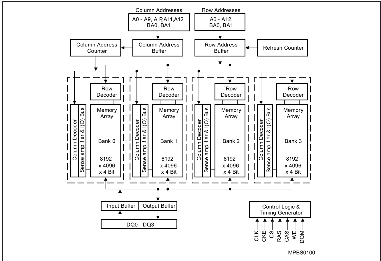
Figure 2 Block Diagram for 128M x 4 SDRAM (13/12/2 Addressing)
