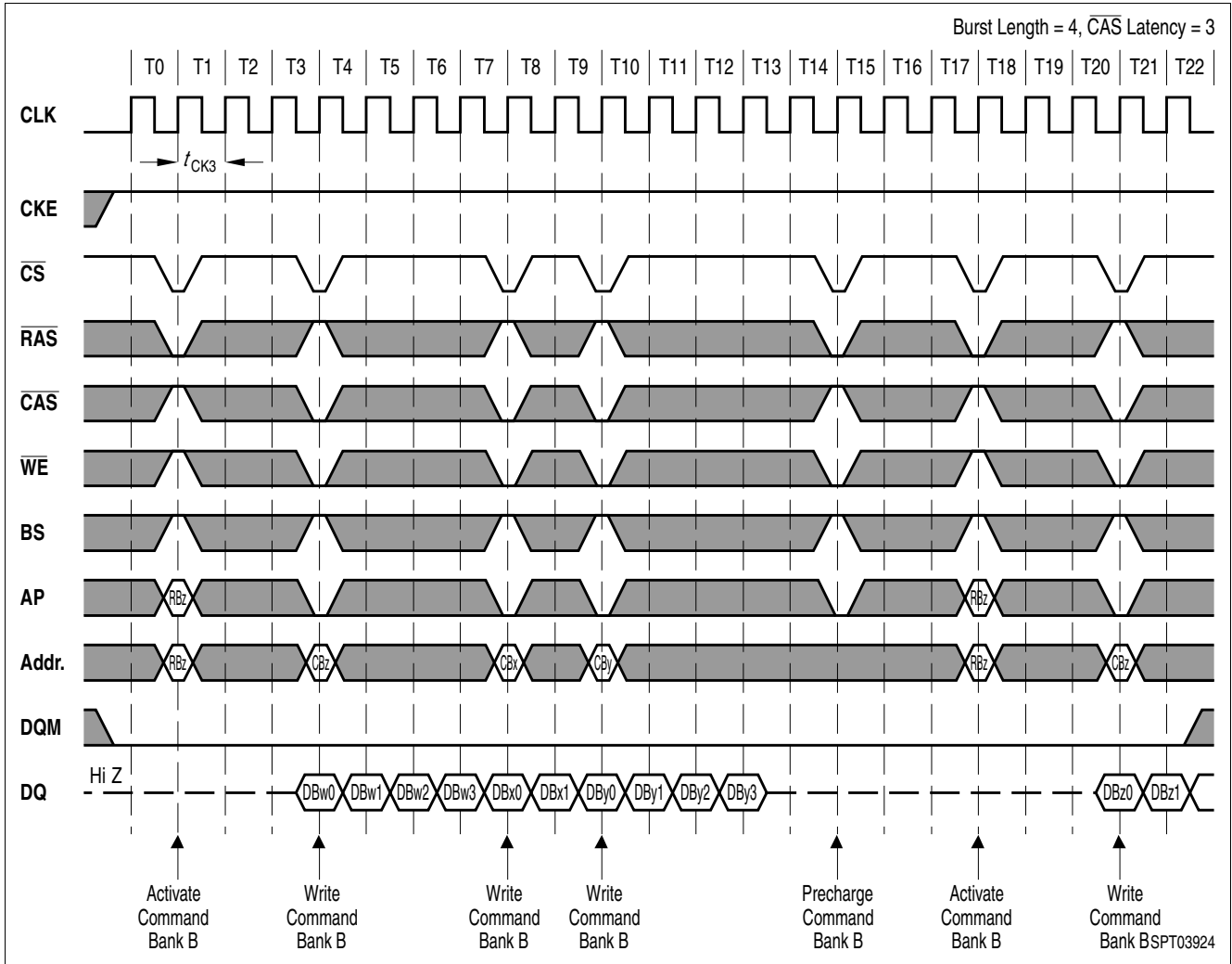
Figure 31 CAS Latency = 3
