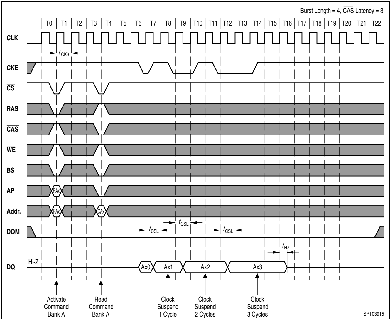
Figure 22 Clock Suspension During Burst Read CAS Latency = 3
