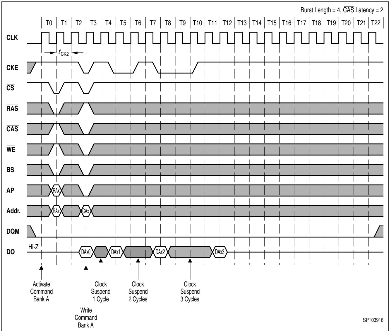
Figure 23 Clock Suspension During Burst Write CAS Latency = 2
