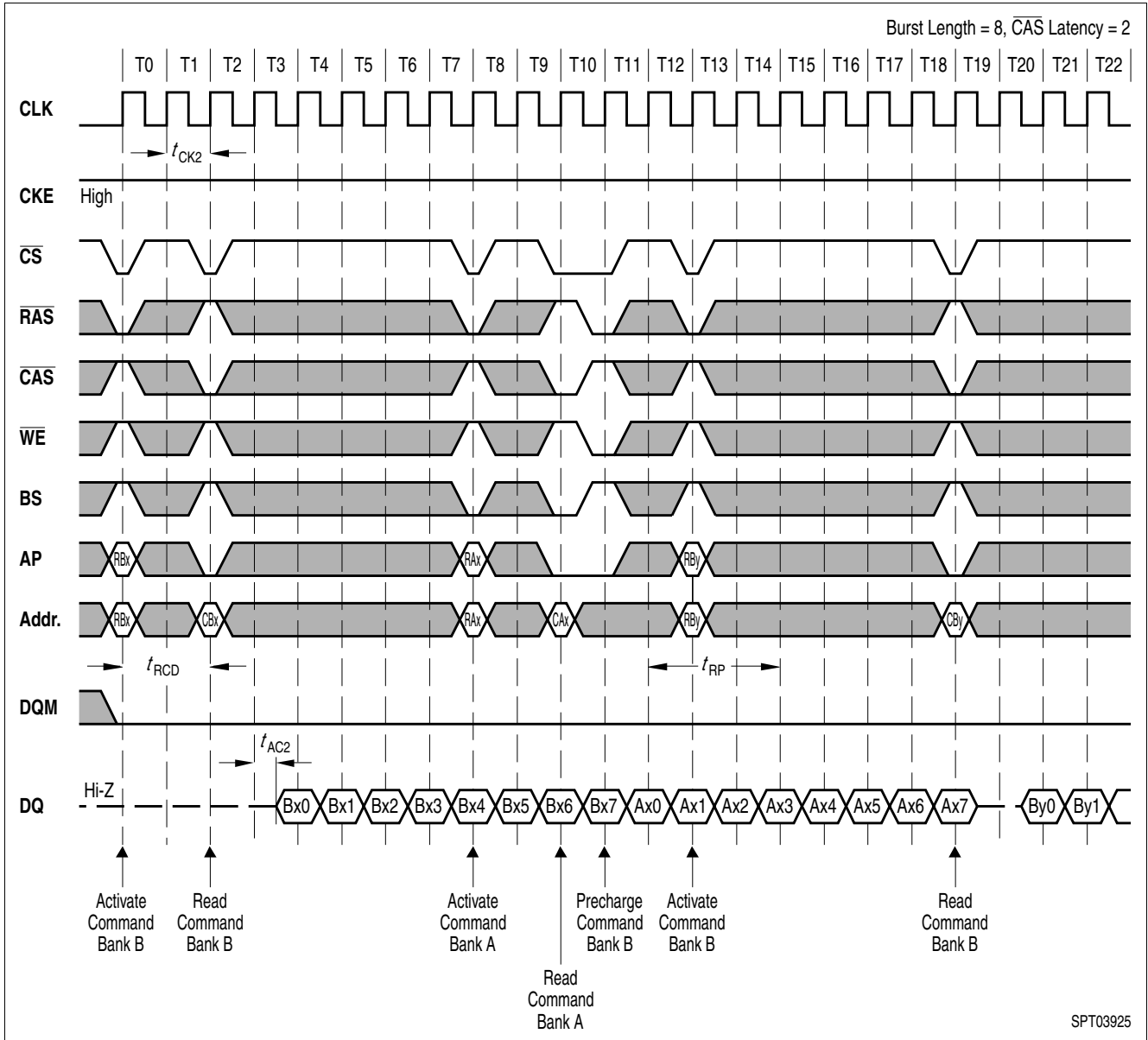
Figure 32 CAS Latency = 2
