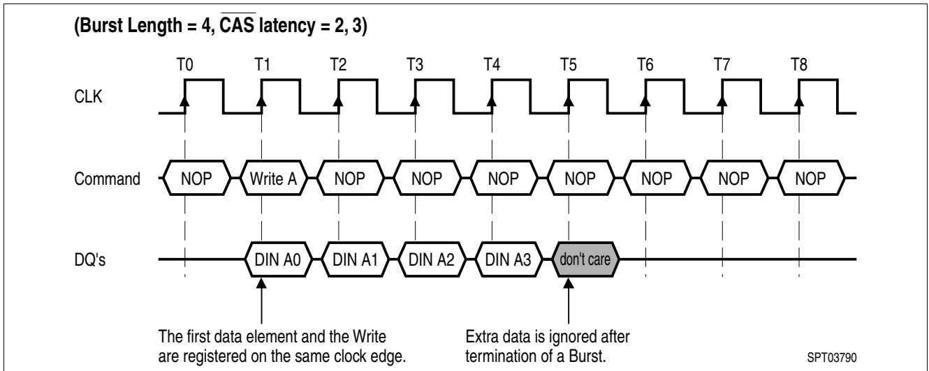
Figure 12 Burst Write Operation
