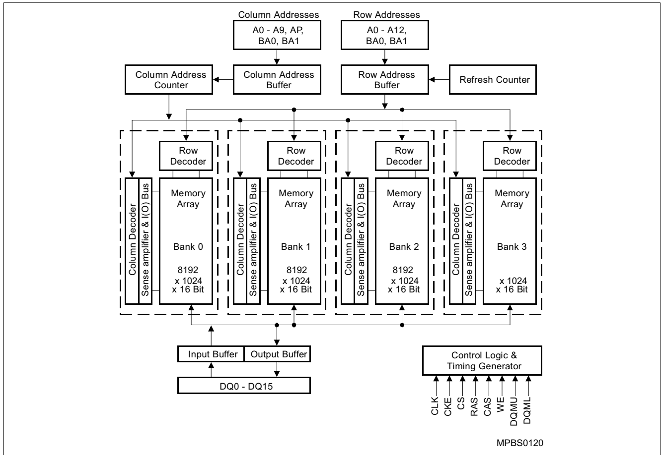
Figure 4 Block Diagram for 32M x 16 SDRAM (13/10/2 Addressing)
