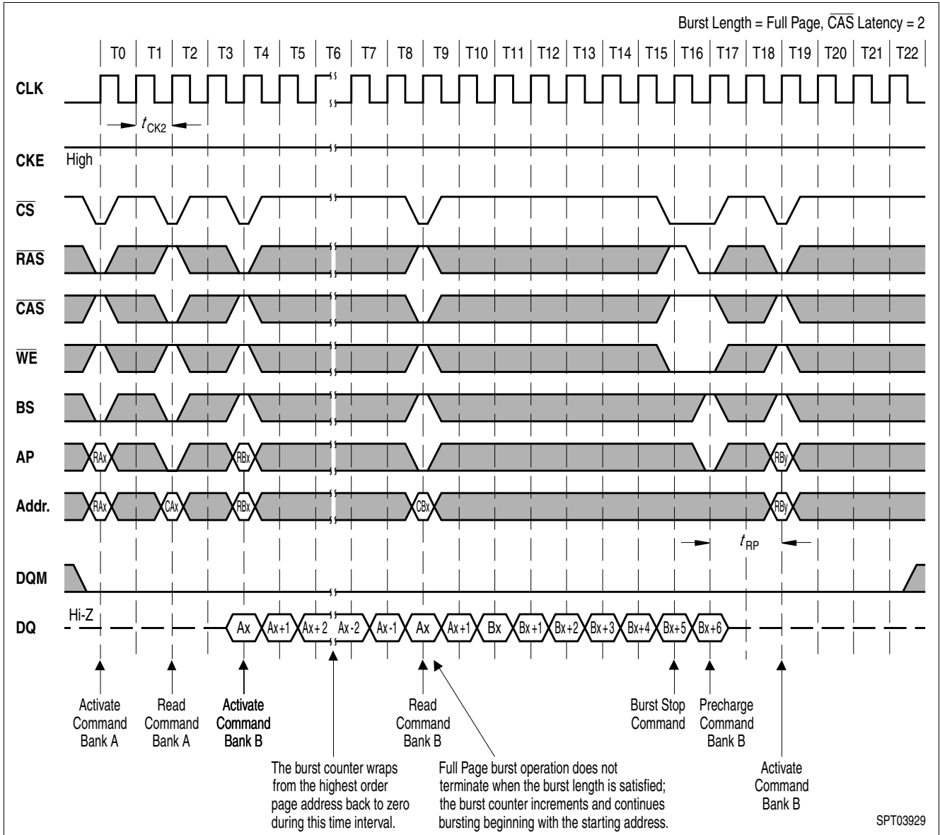
Figure 37 Full Page Burst Read, CAS Latency = 2
