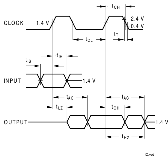
Figure 5 Measurement conditions for t_{AC} and t_{OH}
