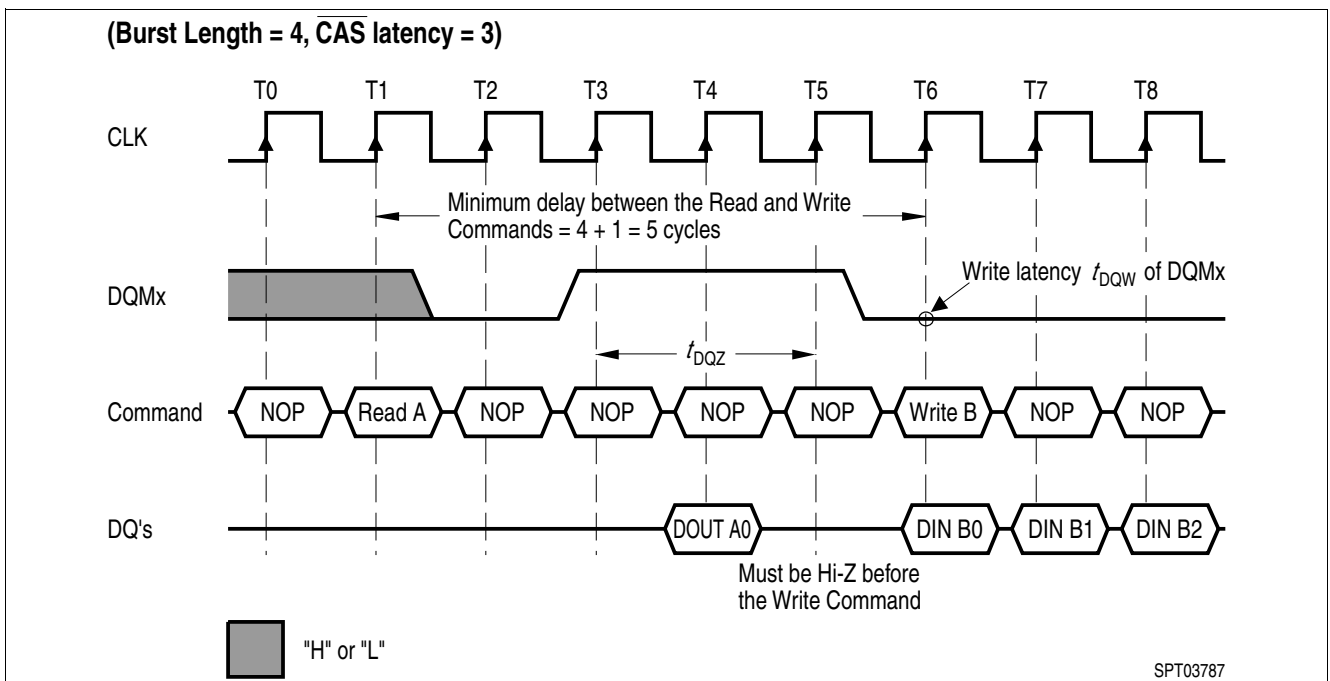
Figure 9 Read to Write Interval
