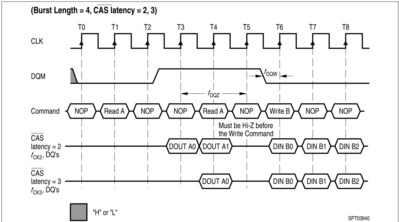
Figure 11 Non-Minimum Read to Write Interval
