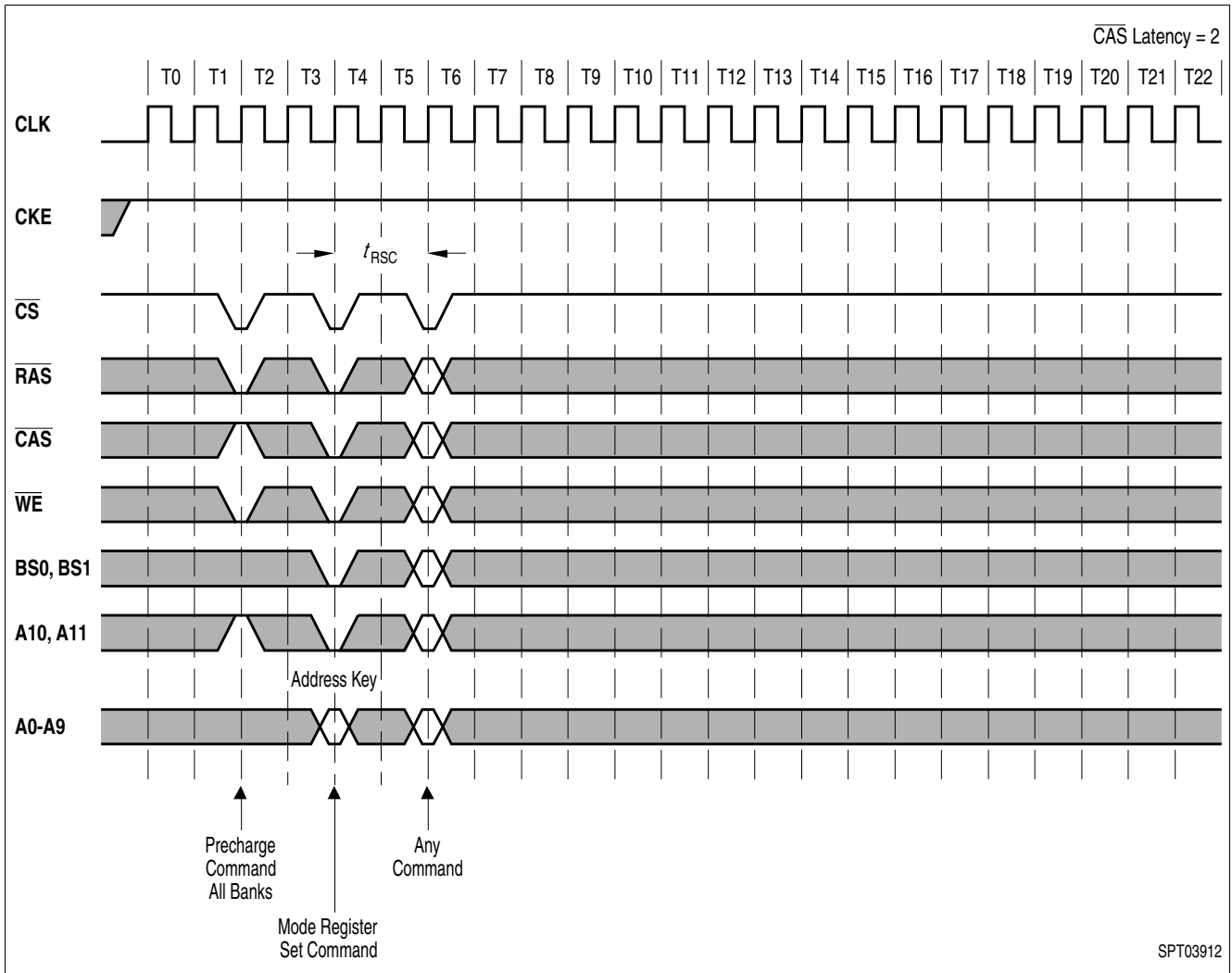
Figure 19 Mode Register Set
