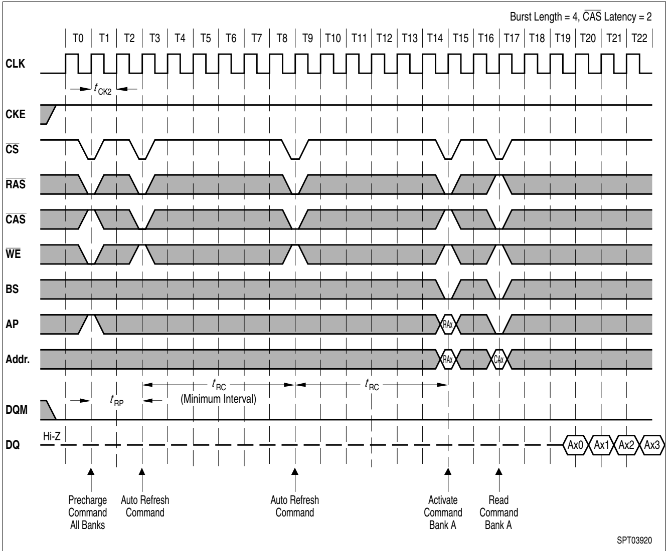
Figure 27 Auto Refresh (CBR)
