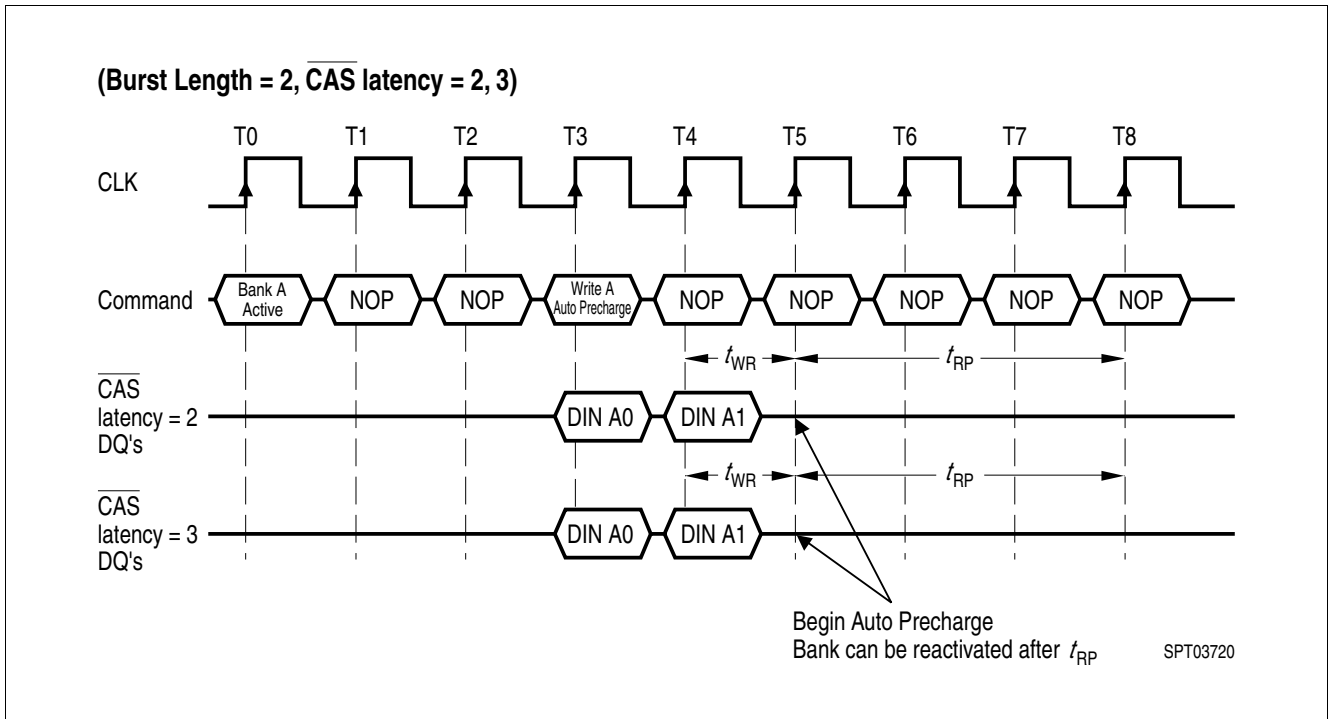
Figure 15 Burst Write with Auto-Precharge
