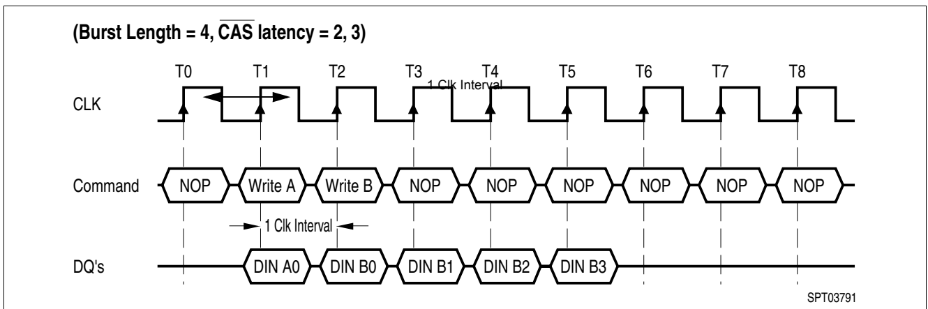
Figure 13 Write Interrupted by a Write
