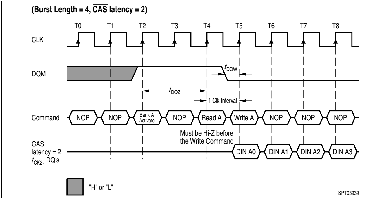
Figure 10 Minimum Read to Write Interval
