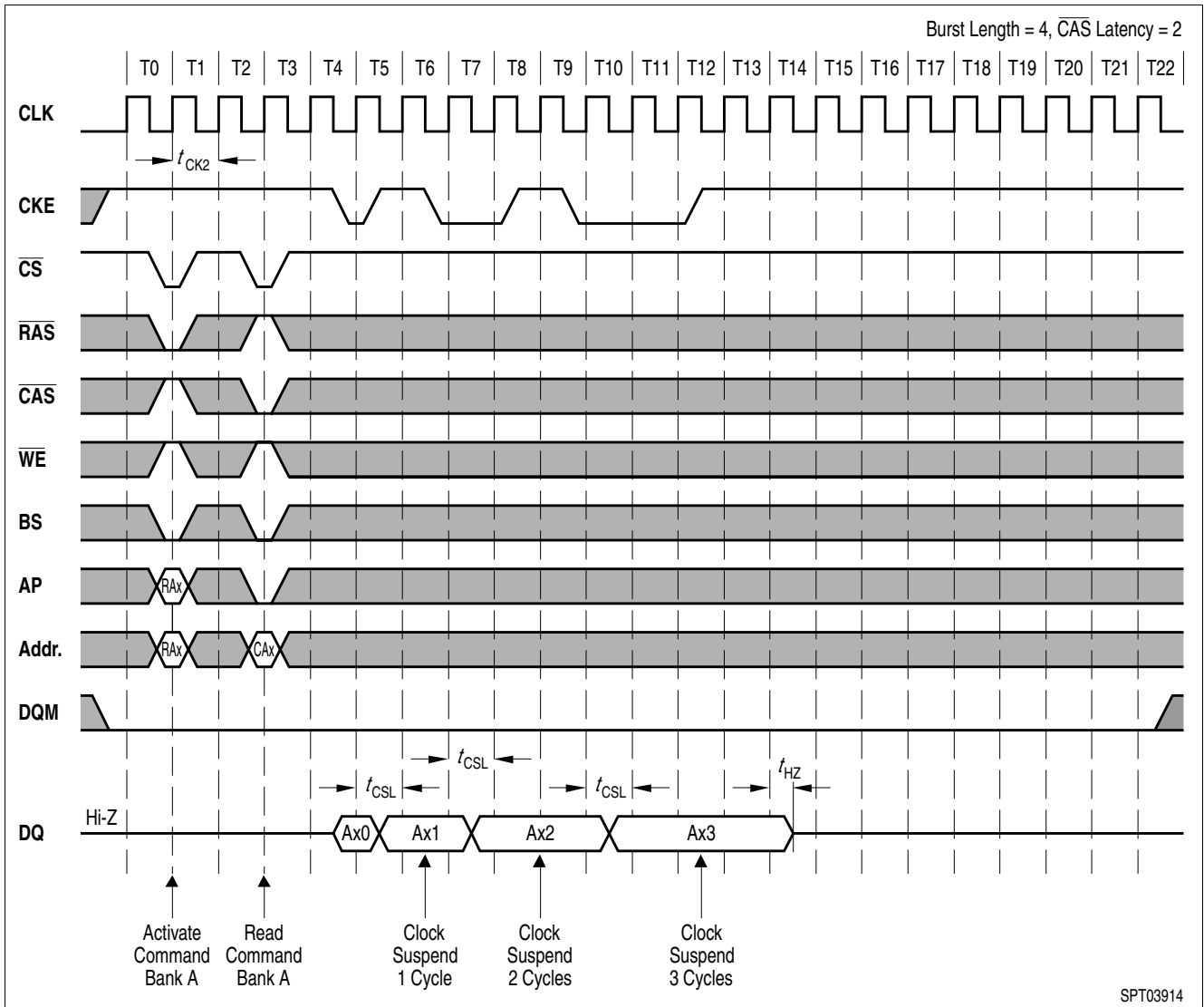
Figure 21 Clock Suspension During Burst Read CAS Latency = 2
