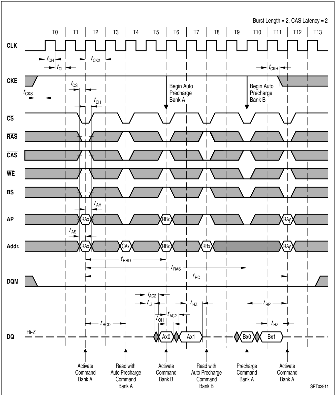
Figure 18 AC Parameters for a Read Timing
