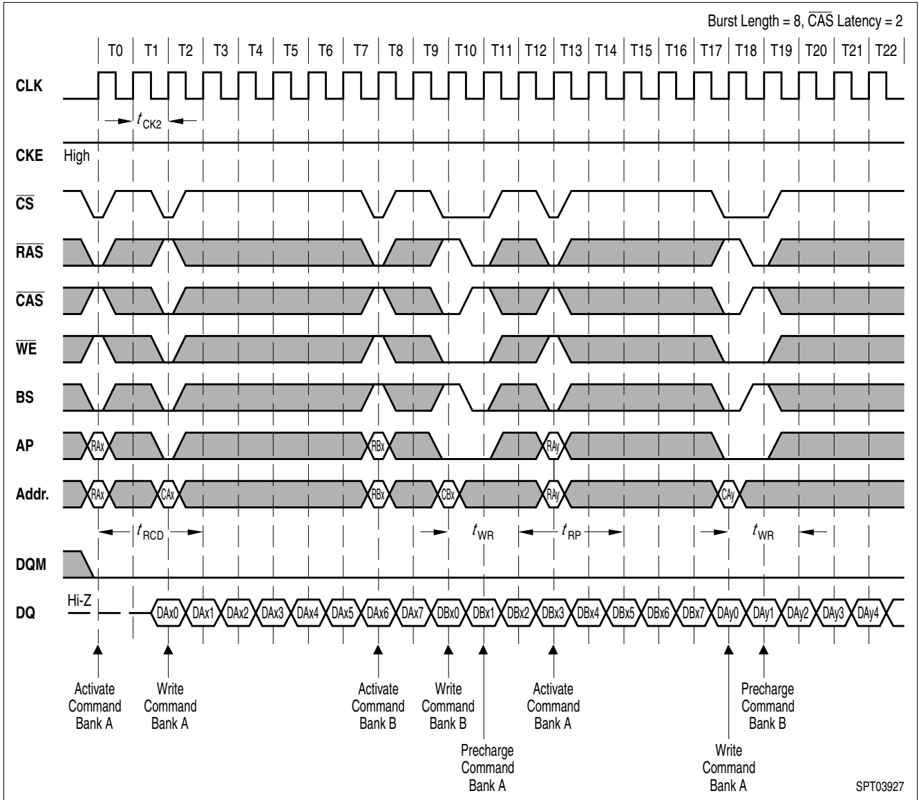
Figure 34 CAS Latency = 2
