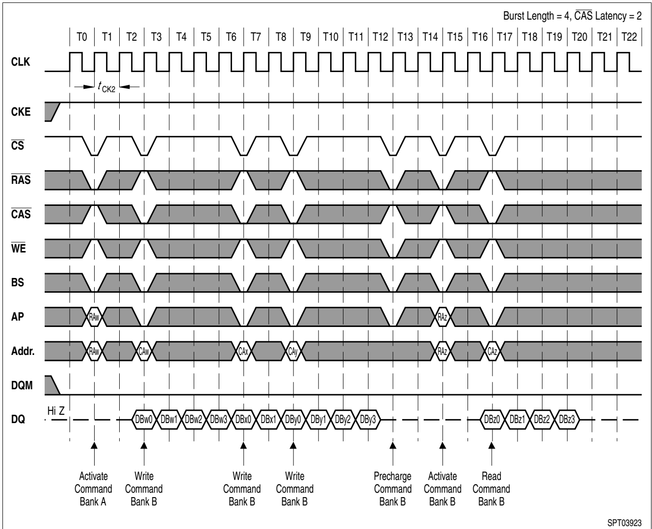
Figure 30 CAS Latency = 2
