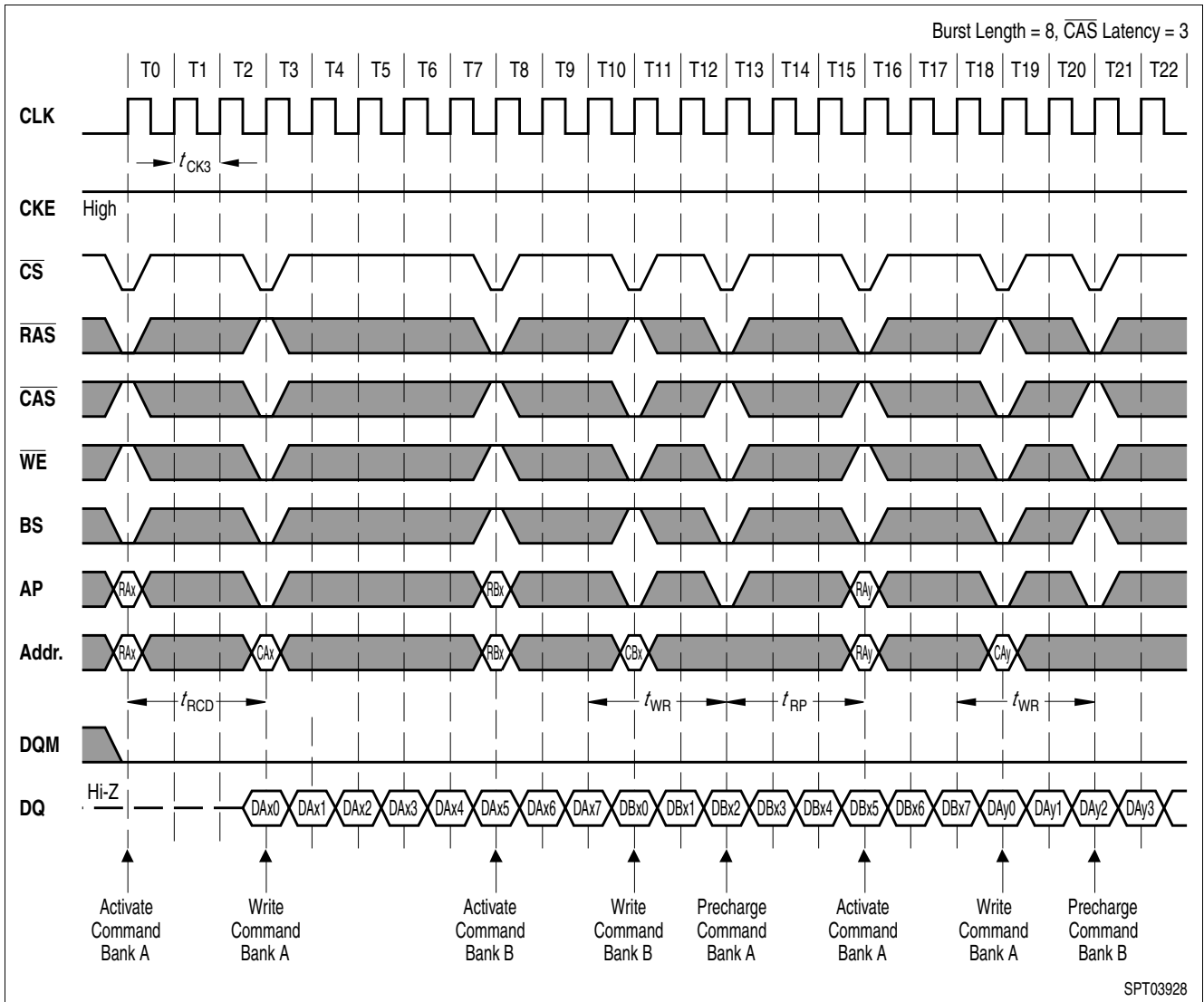
Figure 35 CAS Latency = 3
