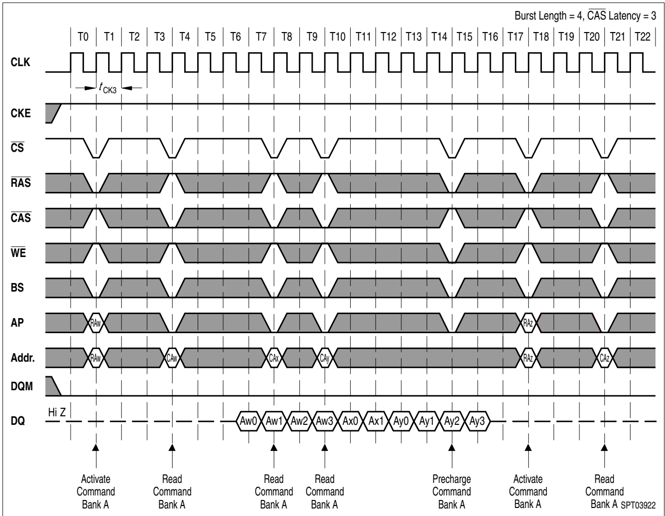
Figure 29 CAS Latency = 3
