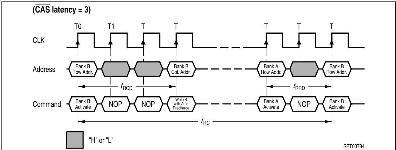
Figure 6 Bank Activate Command Cycle
