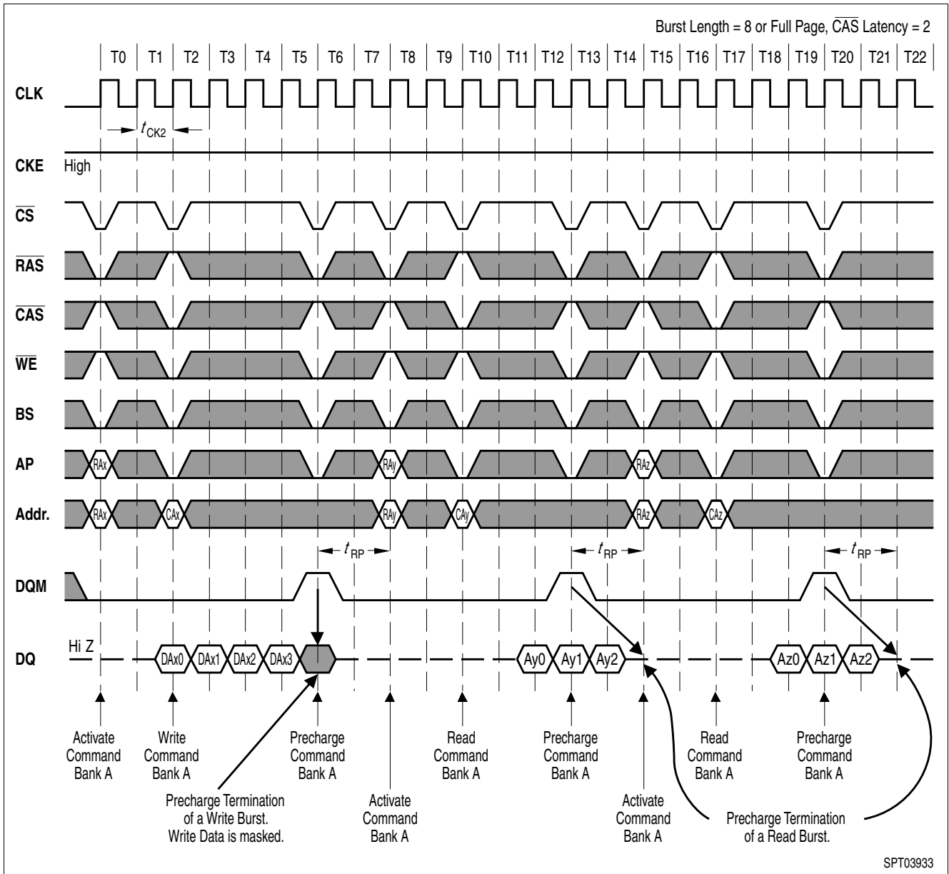
Figure 36 CAS Latency = 2
