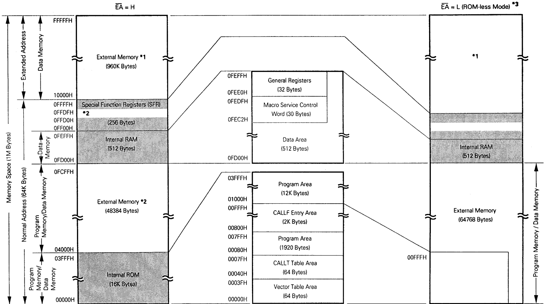
Fig. 2-2 \mu PD78213/78214 Memory Map
