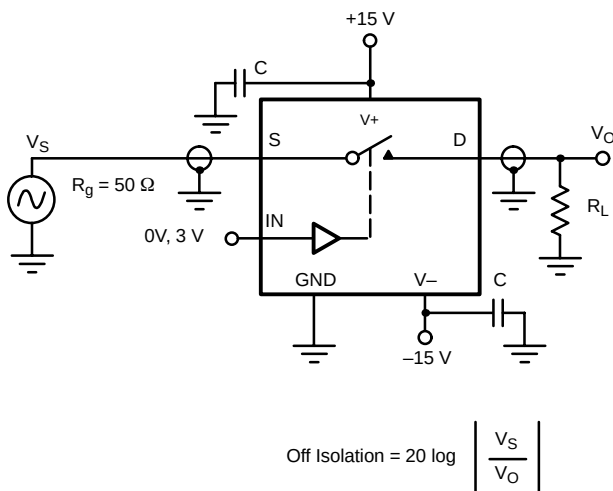
FIGURE 4. Off Isolation
