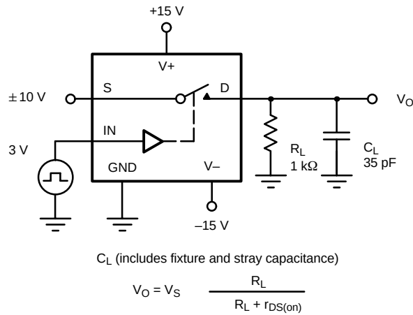
FIGURE 2. Switching Time
