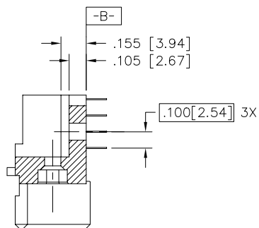
SECTION U-U
