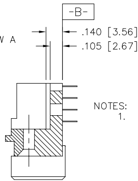
SECTION W-W
