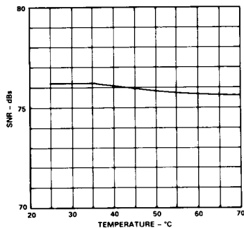
Figure 9. AD7341 SNR vs. Temperature
