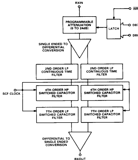
Figure 14. AD7371 Filter Section
