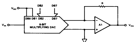
Figure 12. AD7341 Output Attenuator
