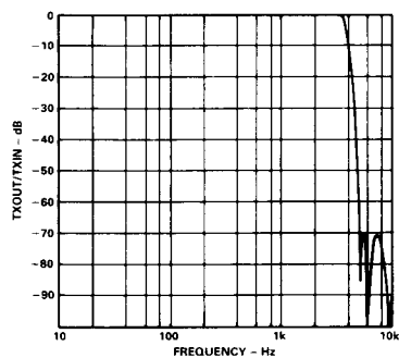
Figure 2. AD7341 Amplitude Response
