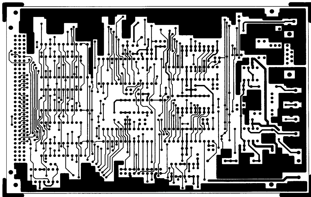
Figure 25. PCB Solder Side Layout for Figure 23
