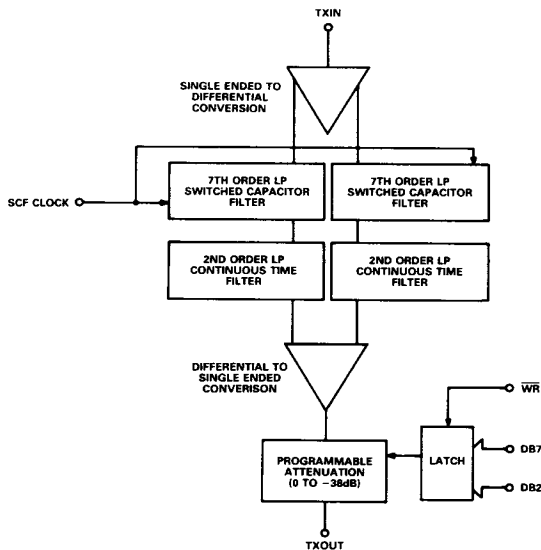
Figure 11. AD7341 Filter Section
