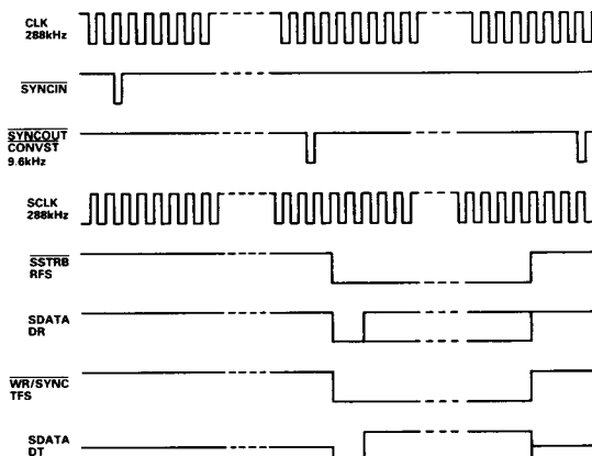
Figure 20. System Timing for Figure 19
