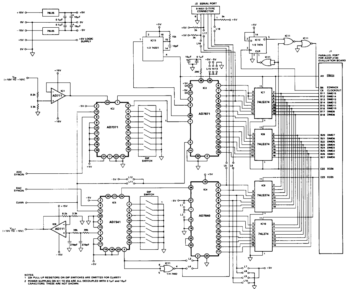
Figure 23. Circuit Diagram for Modem Analog Front End
