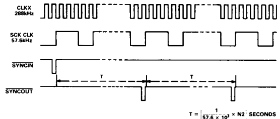
Figure 18. AD7341/AD7371 Timing Waveforms
