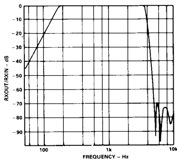
Figure 3. AD7371 Amplitude Response
