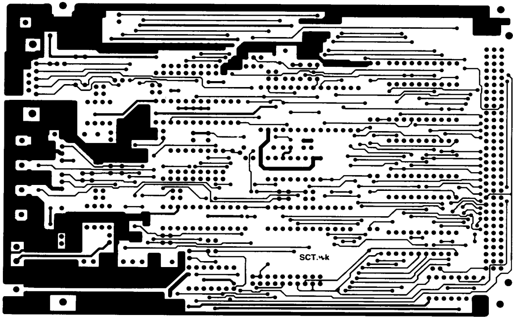
Figure 24. PCB Component Side Layout for Figure 23
