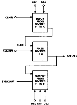
Figure 17. AD7341/AD7371 Clock Generation Circuitry
