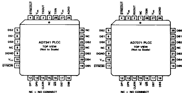
PLCC
