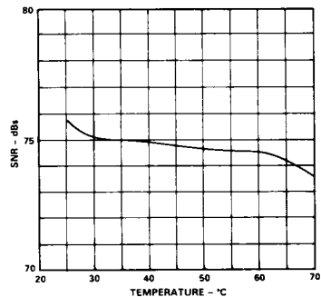
Figure 10. AD7371 SNR vs. Temperature
