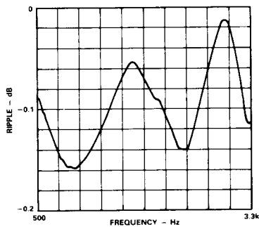
Figure 6. Passband Ripple in the AD7341/AD7371
