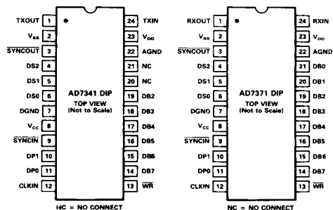
DIP
