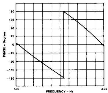
Figure 5. AD7371 Phase Response
