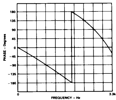
Figure 4. AD7341 Phase Response
