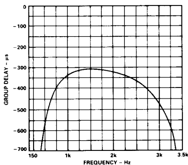
Figure 8. AD7371 Group Delay
