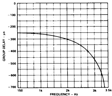
Figure 7. AD7341 Group Delay
