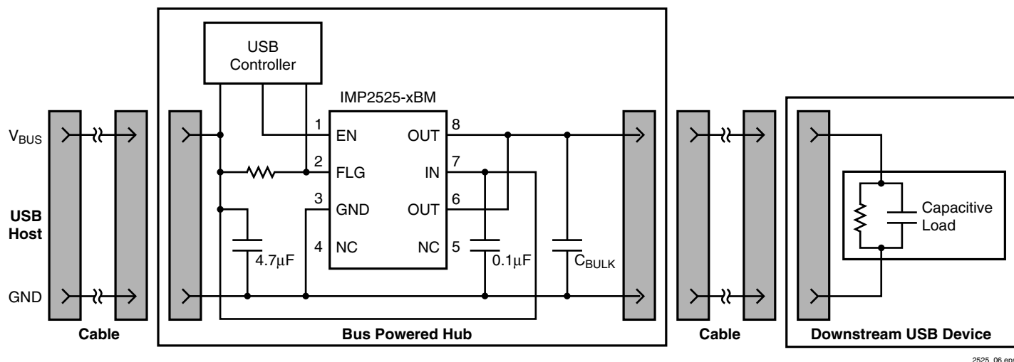
Figure 2. Soft-Start Application
