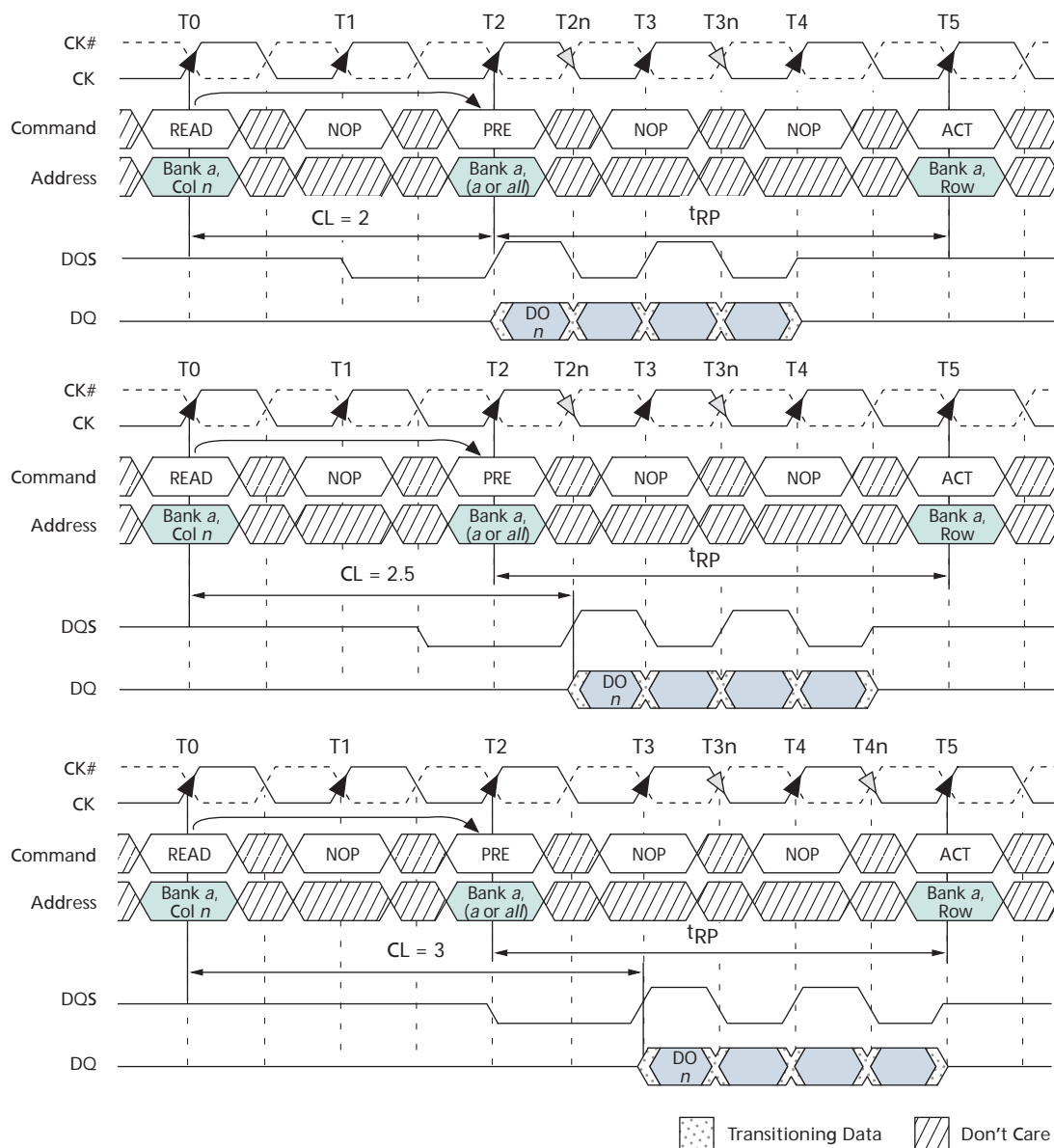
Figure 34: READ-to-PRECHARGE
