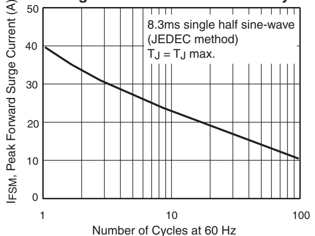
Fig. 6 - Maximum Non-Repetitive Peak Forwa Surge Current Unidirectional only
