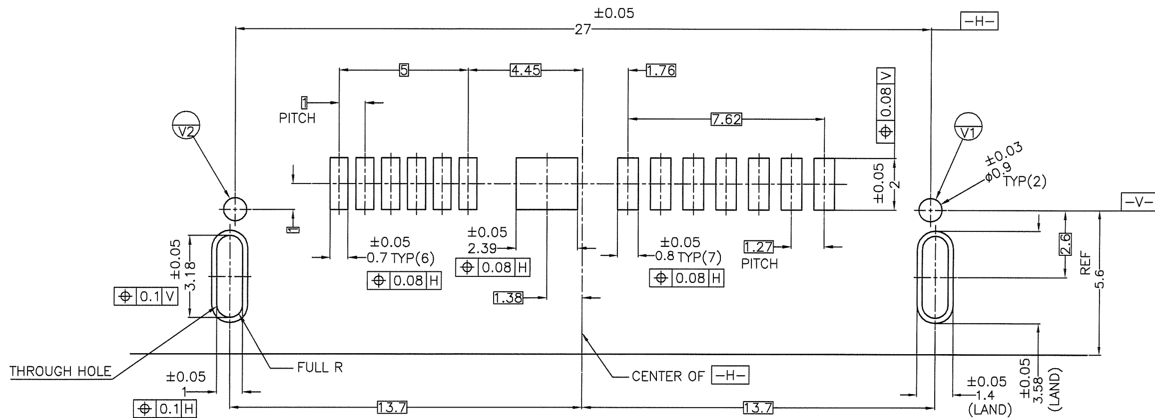
RECOMMENDED PCB PATTERN LAYOUT
