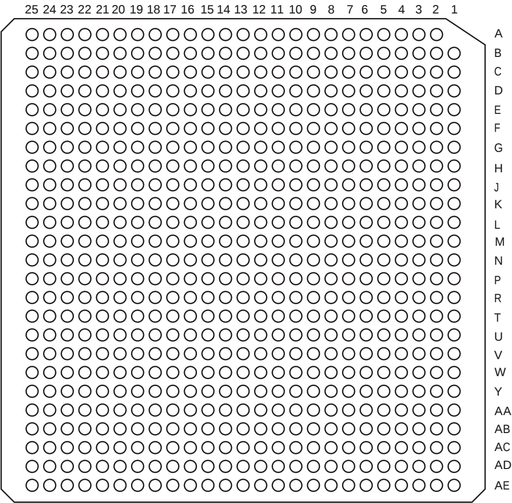
Figure 3-12 • 624-Pin CCGA (Bottom View)
