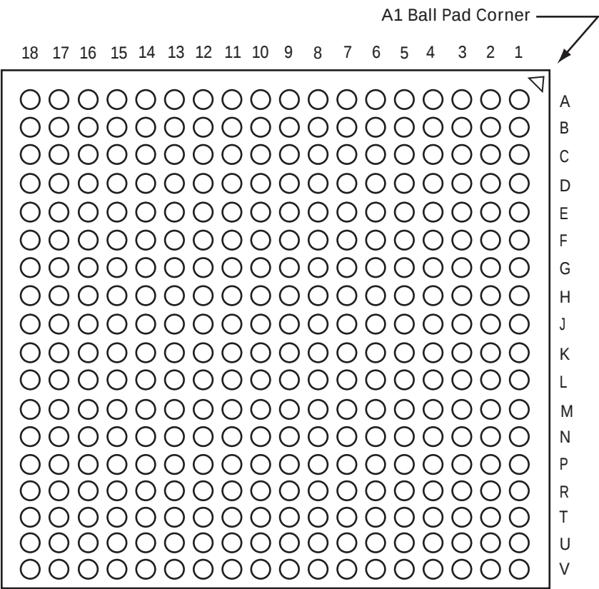
Figure 3-4 • 324-Pin FBGA (Bottom View)
