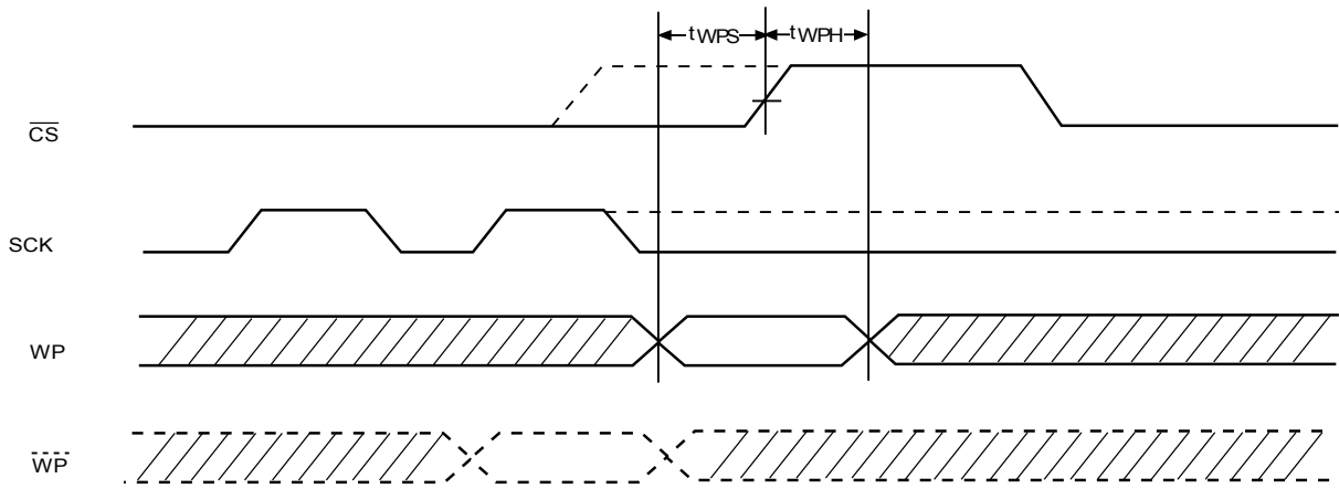
Figure 7. WP Timing
