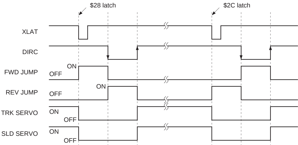
Timing Chart 5-23.
