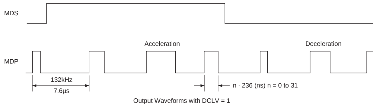
Timing Chart 1-14
