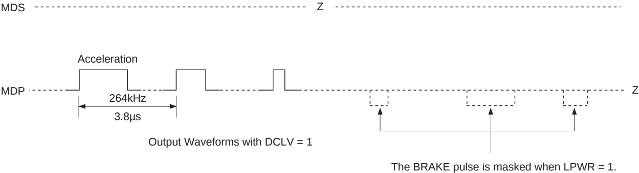
Timing Chart 1-17
