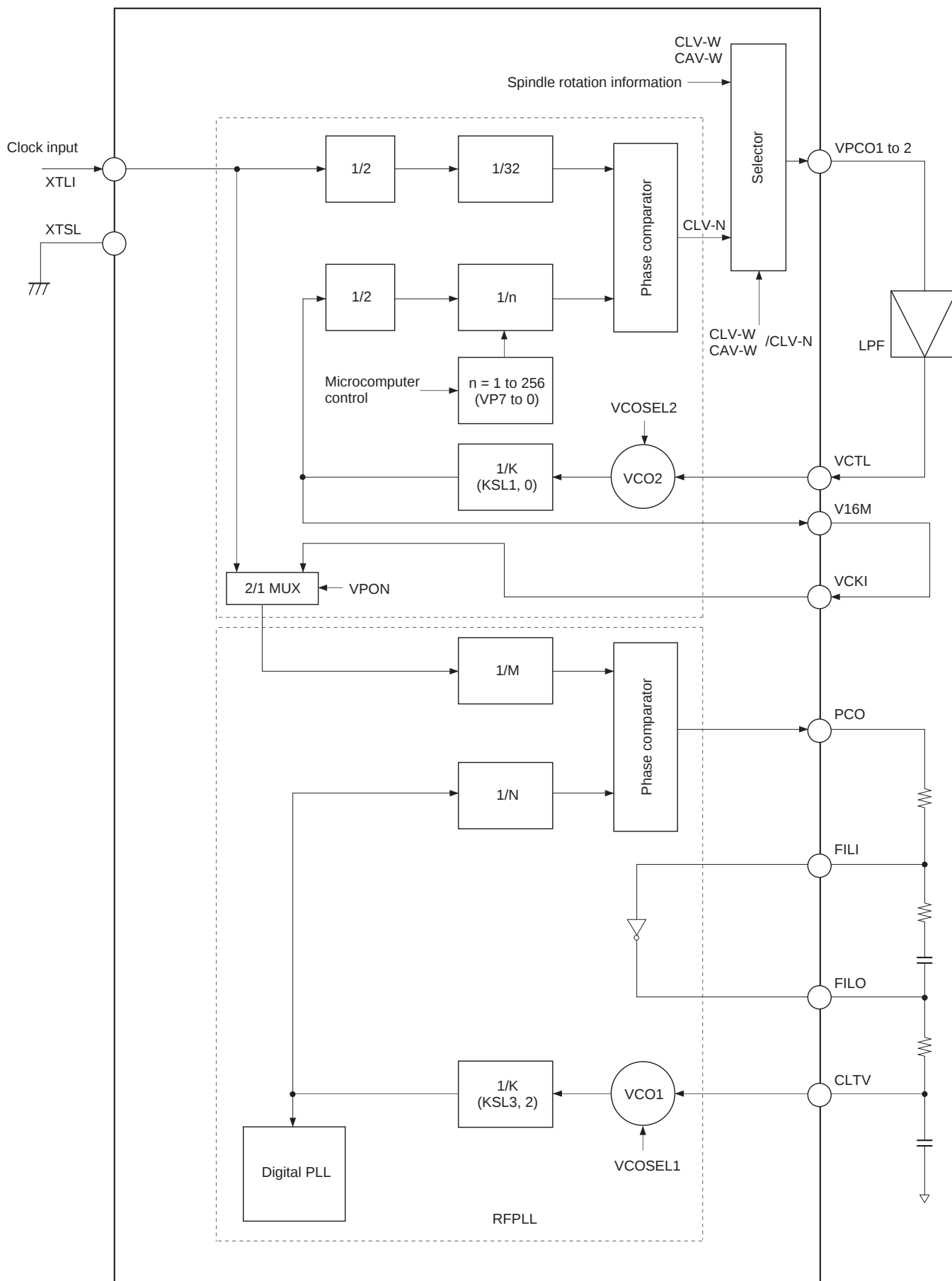
Block Diagram 4-1
