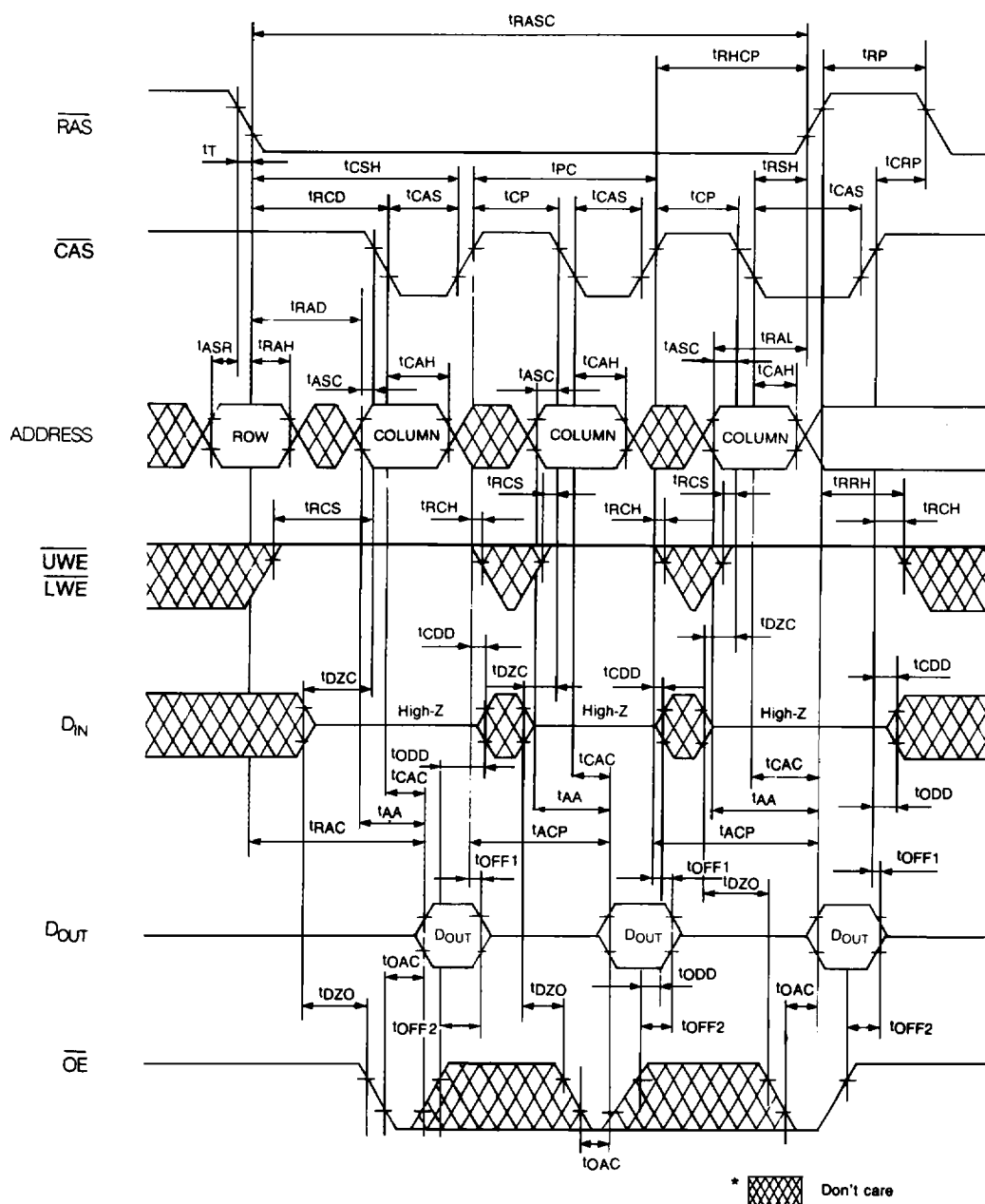
FIGURE 8. FAST PAGE MODE READ CYCLE
