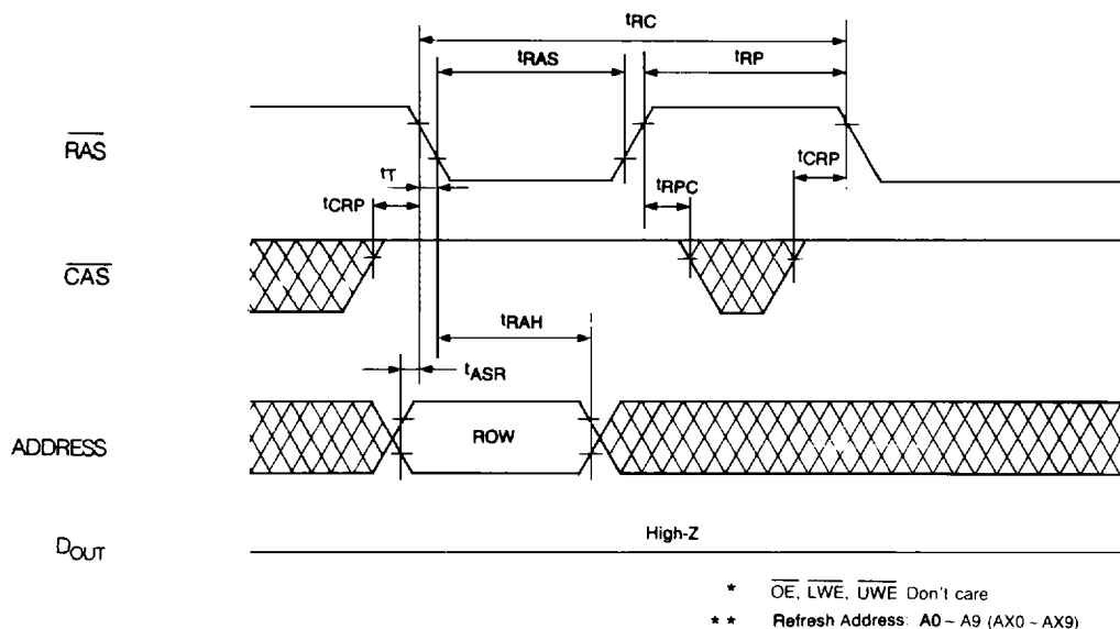
FIGURE 5. RAS-ONLY REFRESH CYCLE
