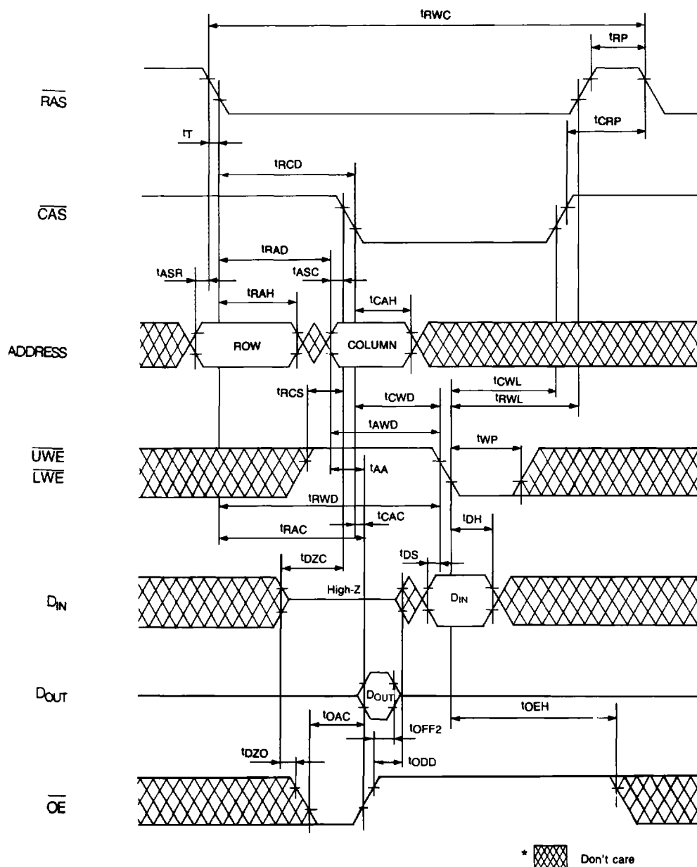
FIGURE 4. READ-MODIFY-WRITE CYCLE
