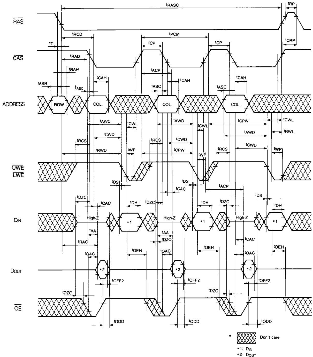
FIGURE 11. FAST PAGE MODE READ-MODIFY-WRITE CYCLE
