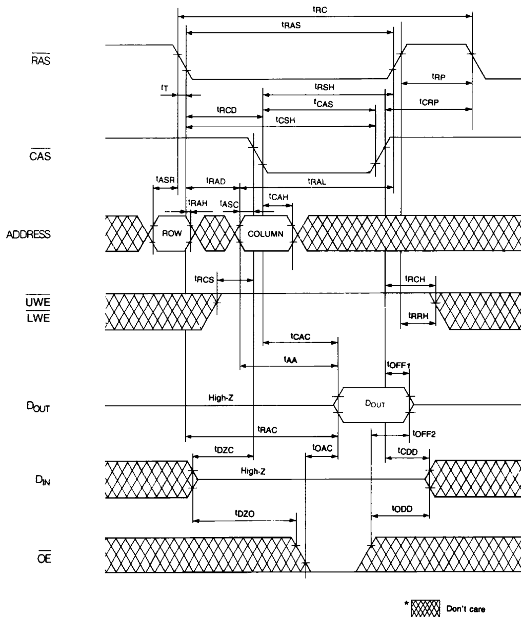
FIGURE 1. READ CYCLE
