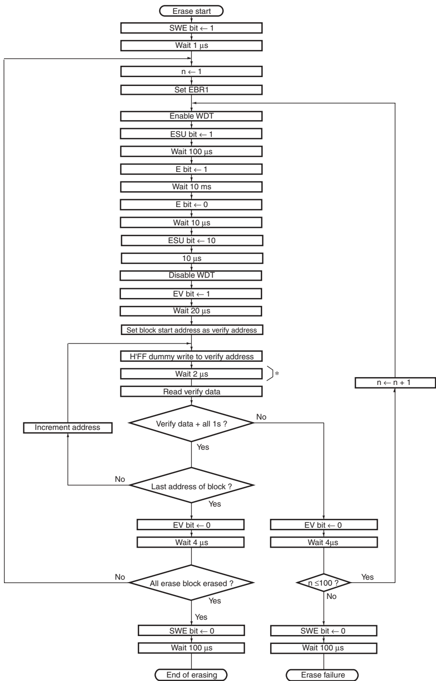
Figure 7.4 Erase/Eraser-Verify Flowchart
