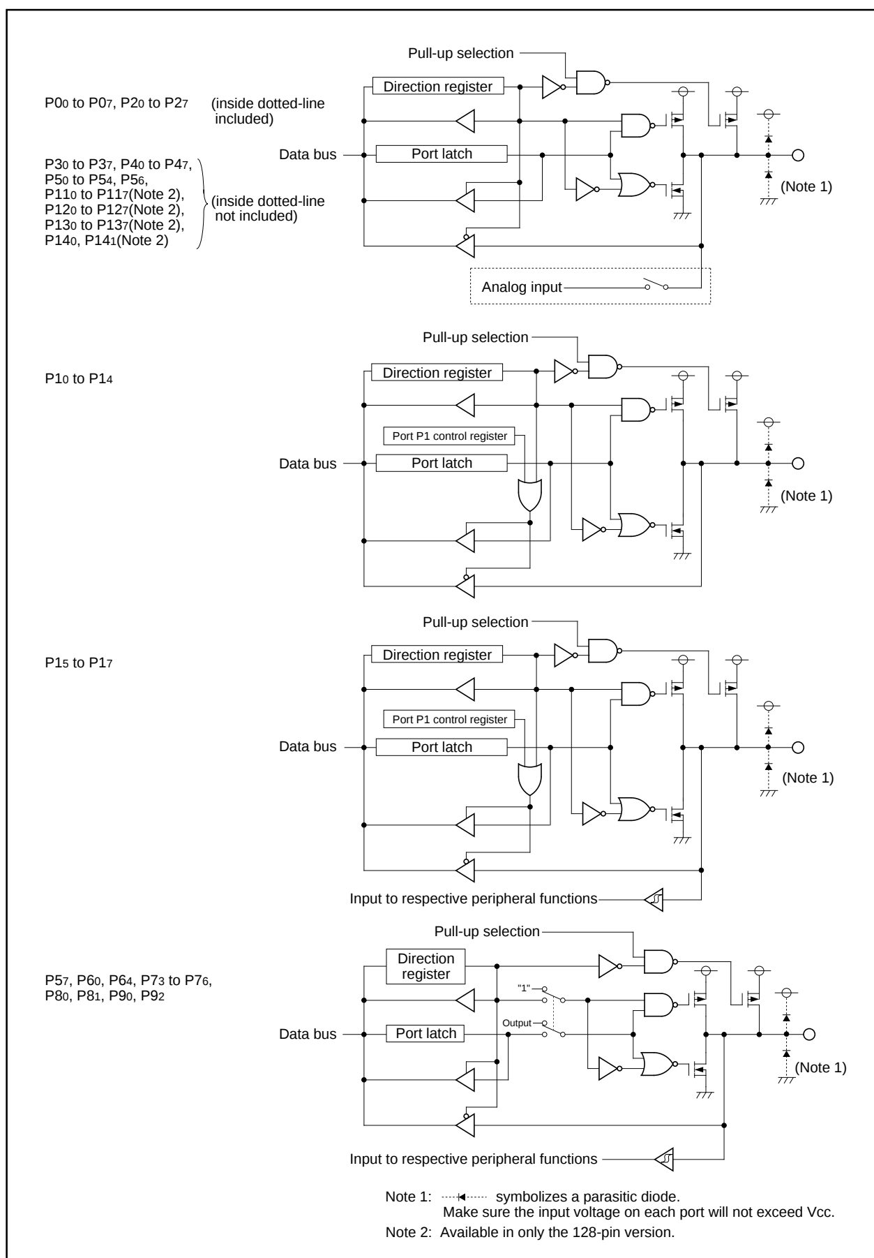
Figure 1.25.1. I/O Ports (1)
