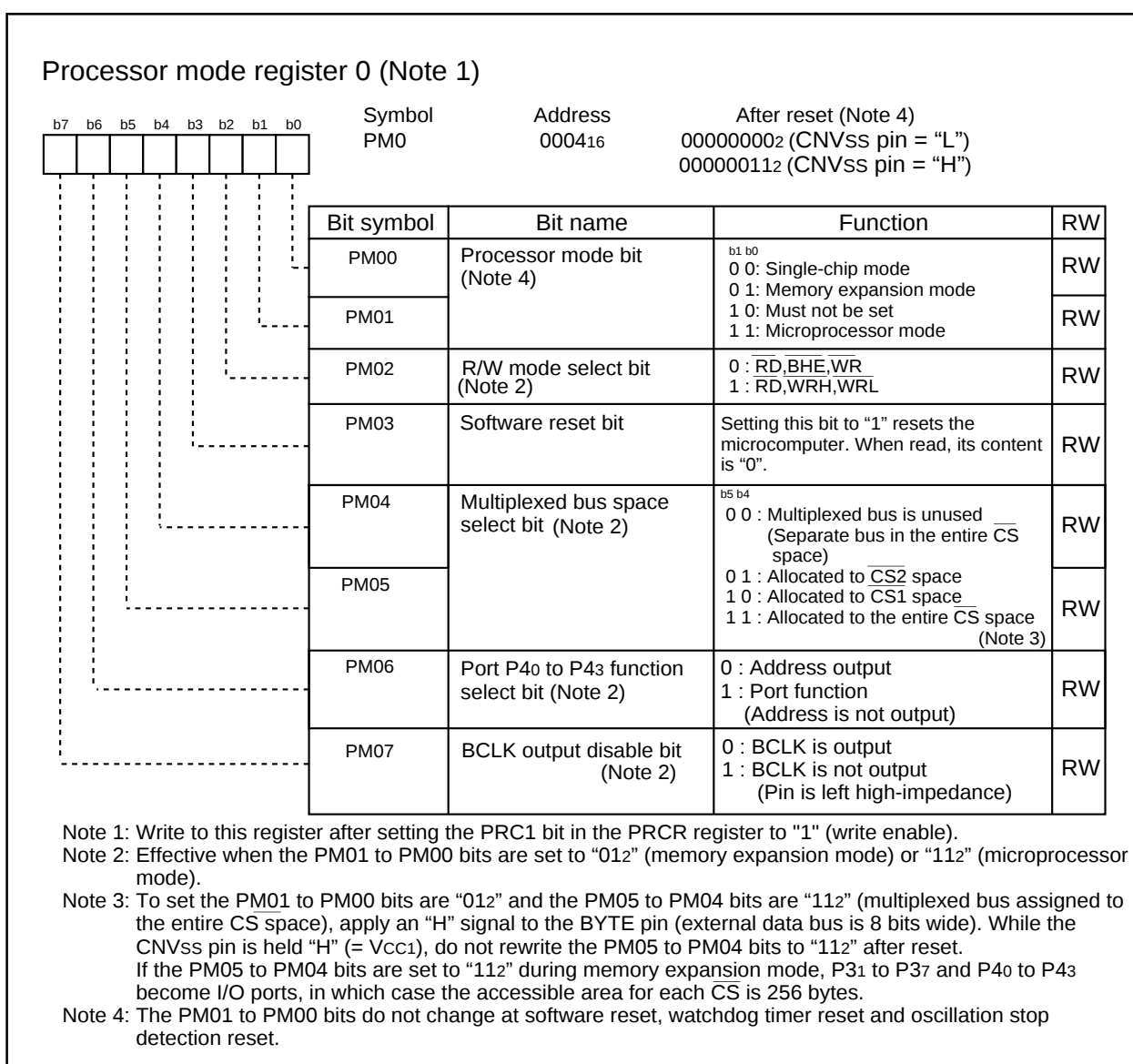
Figure 1.6.1. PM0 Register
