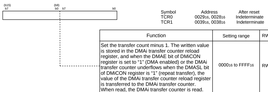
Figure 1.13.4. SAR0, SAR1, DAR0, DAR1, TCR0, and TCR1 Registers
