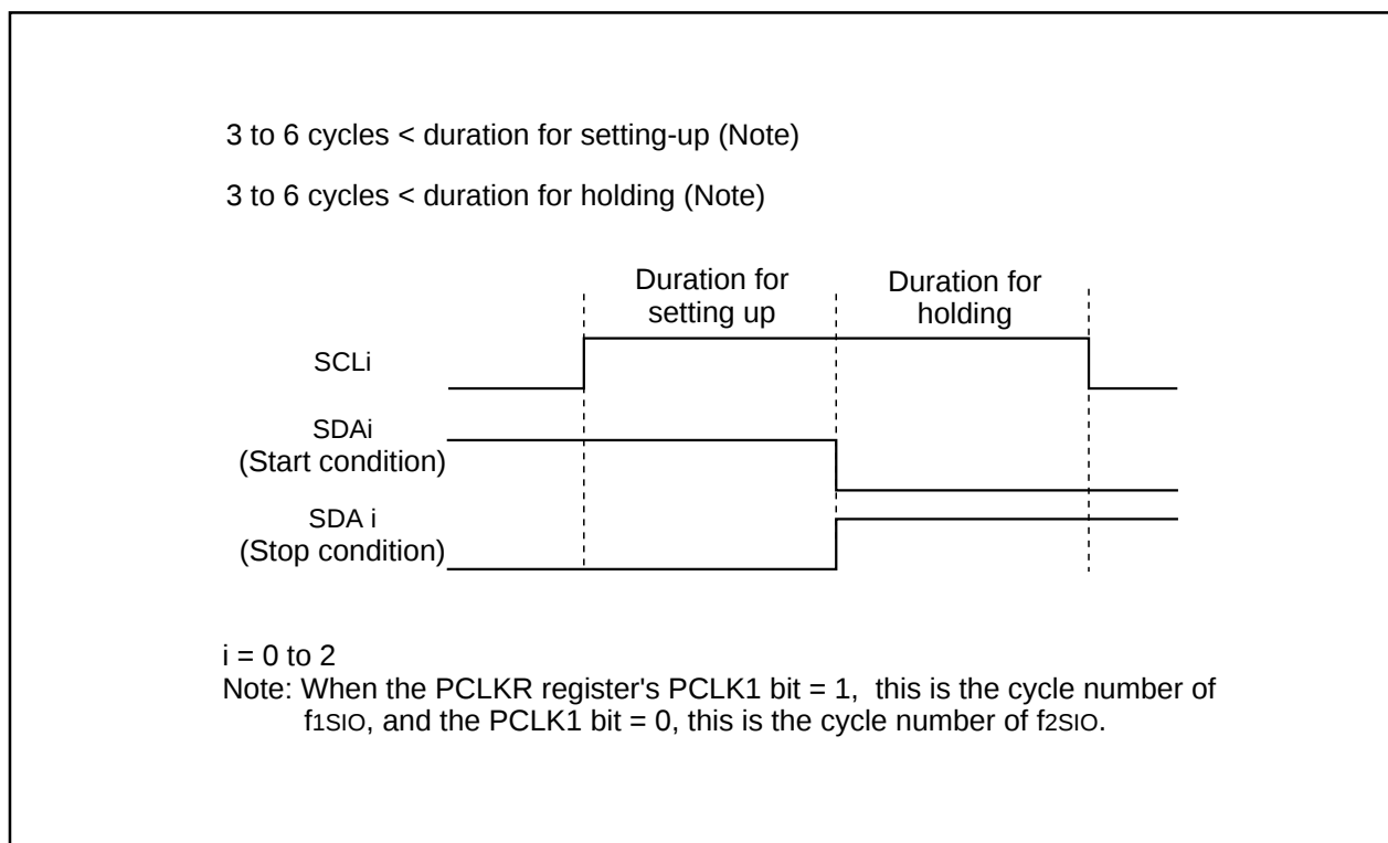
Figure 1.20.3. Detection of Start and Stop Condition
