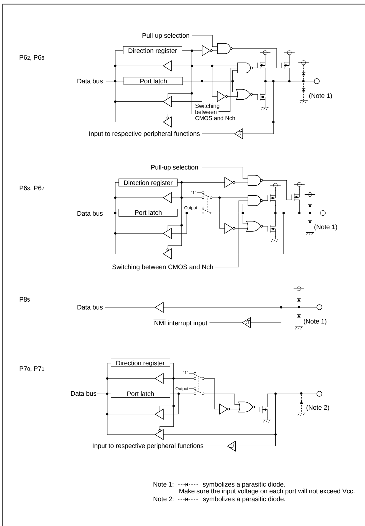
Figure 1.25.3. I/O Ports (3)
