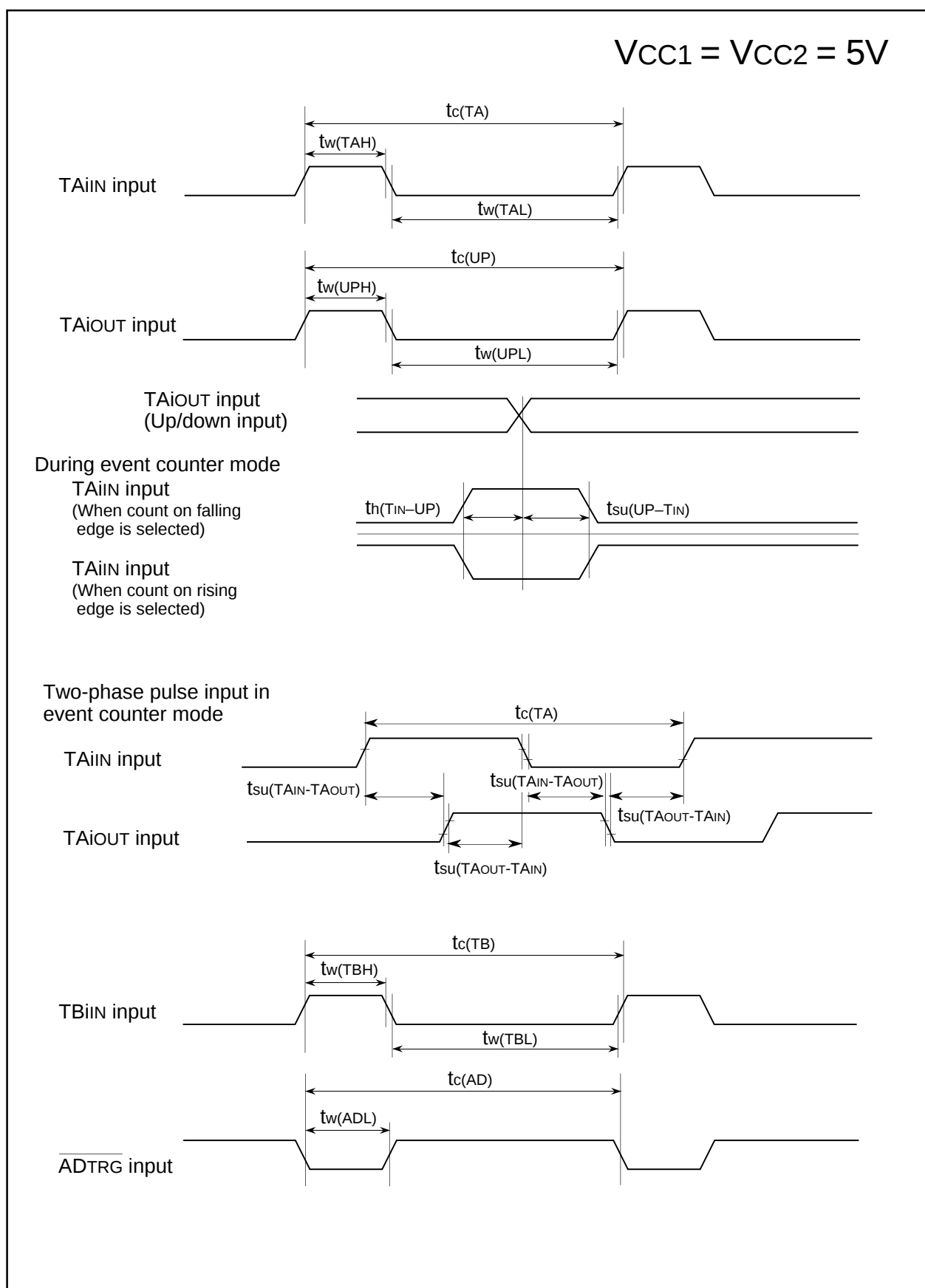
Figure 1.26.2. Timing Diagram (1)
