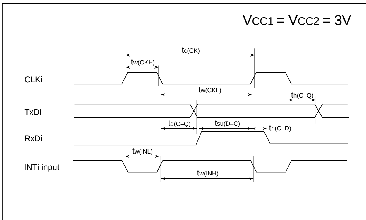
Figure 1.26.13. Timing Diagram (2)
