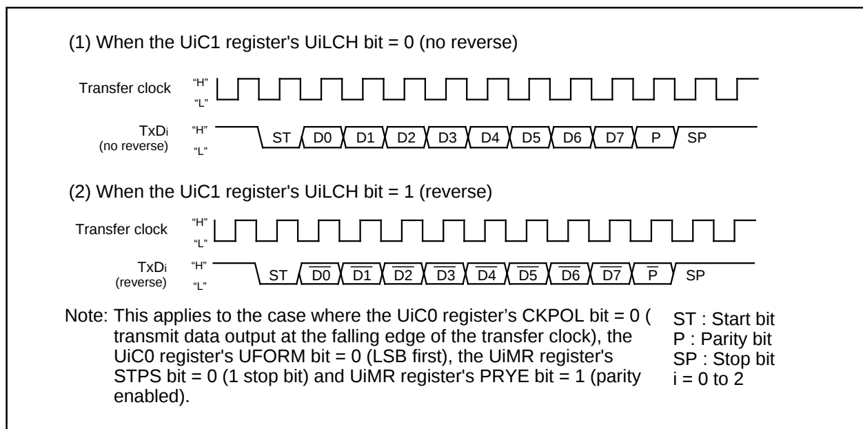
Figure 1.19.4. Serial Data Logic Switching
