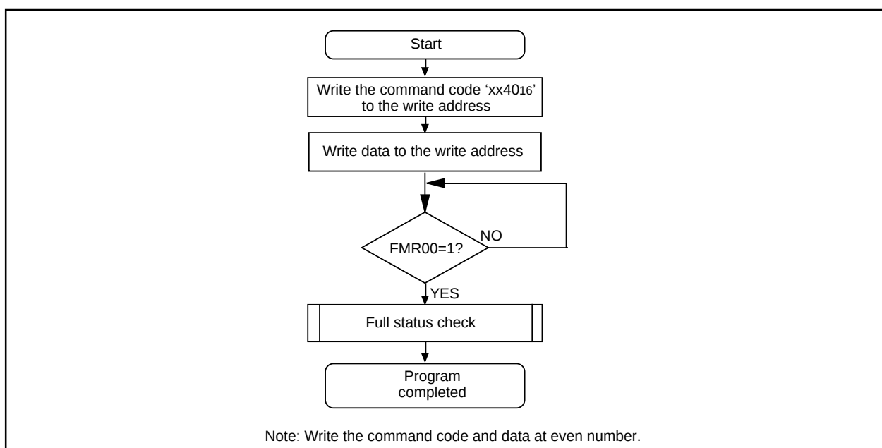
Figure 1.27.8. Program Command
