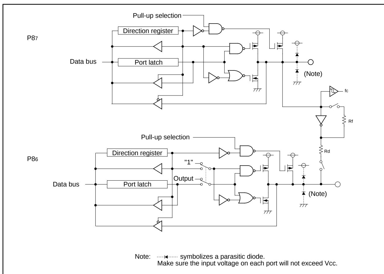
Figure 1.25.5. I/O Ports (5)
