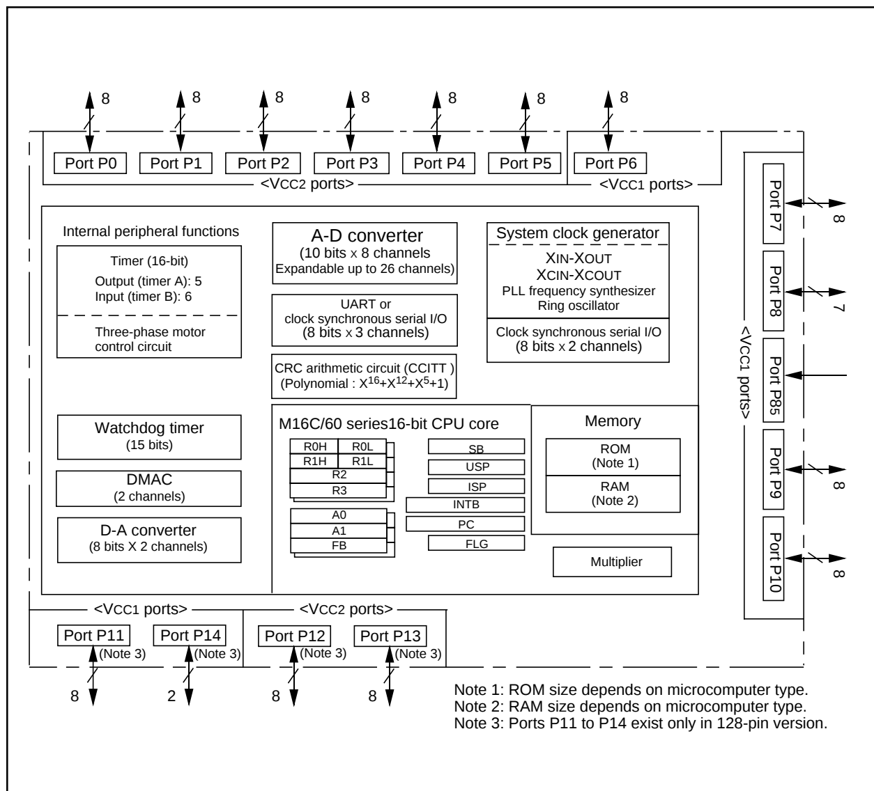
Figure 1.1.1. Block Diagram
