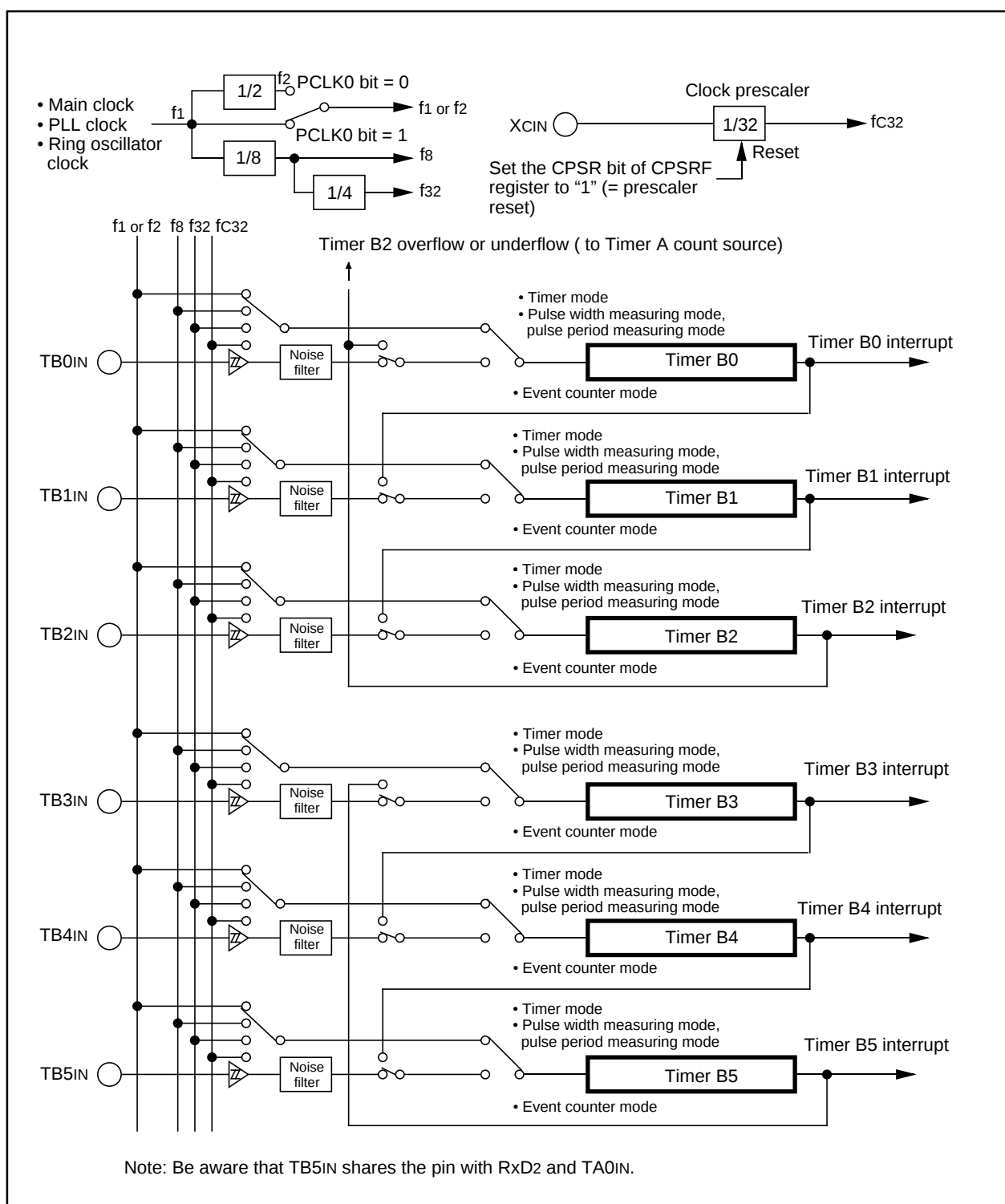
Figure 1.14.2. Timer B Configuration
