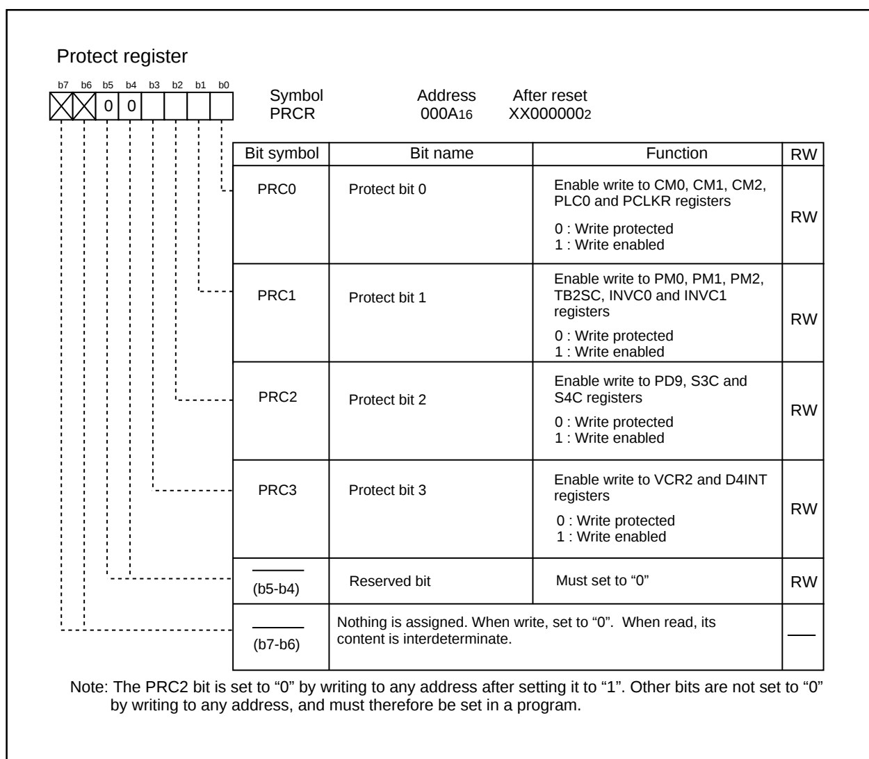
Figure 1.10.1. PRCR Register
