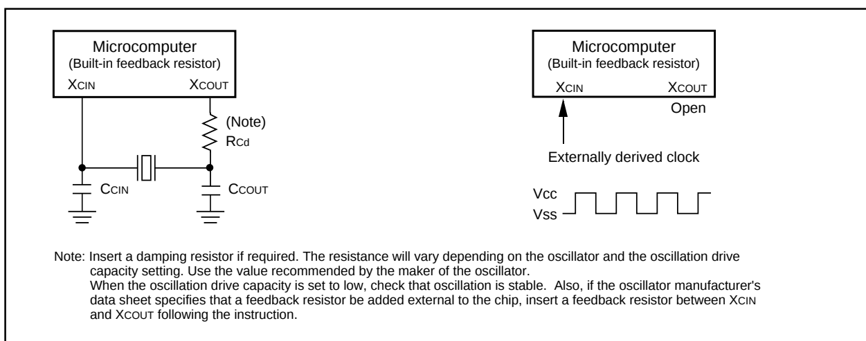
Figure 1.9.8. Examples of Sub Clock Connection Circuit
