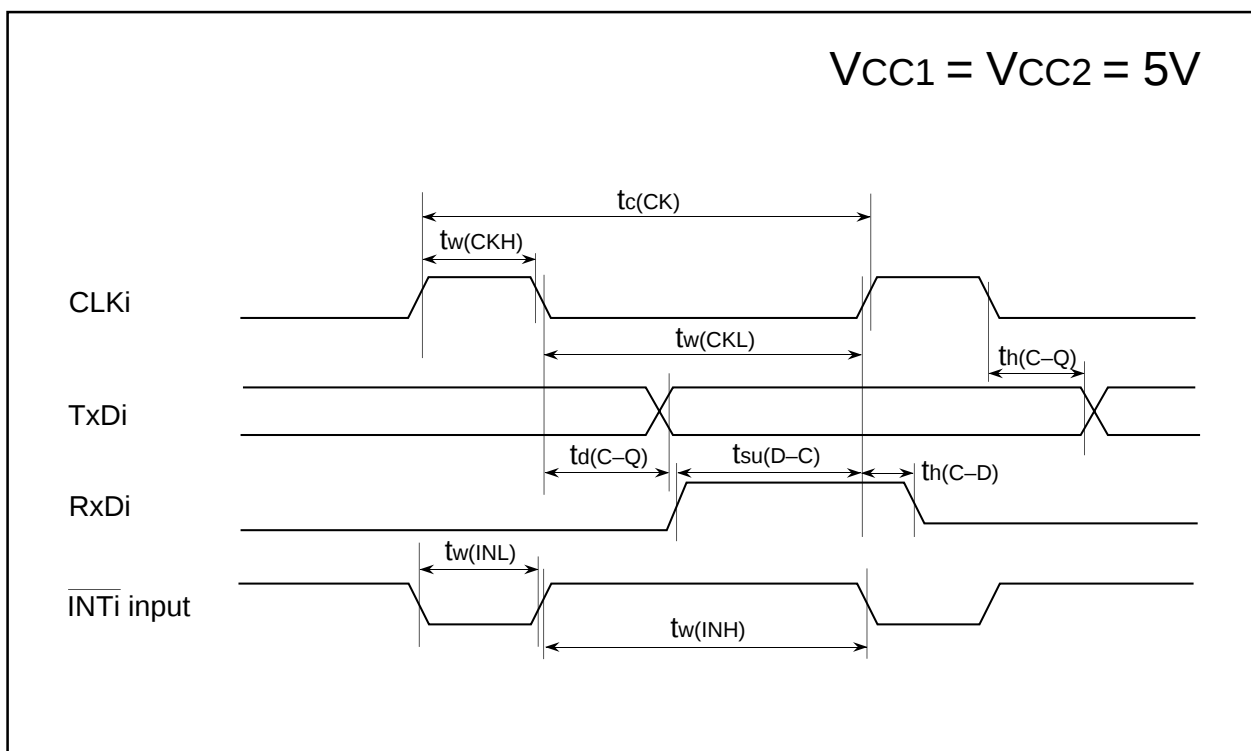
Figure 1.26.3. Timing Diagram (2)
