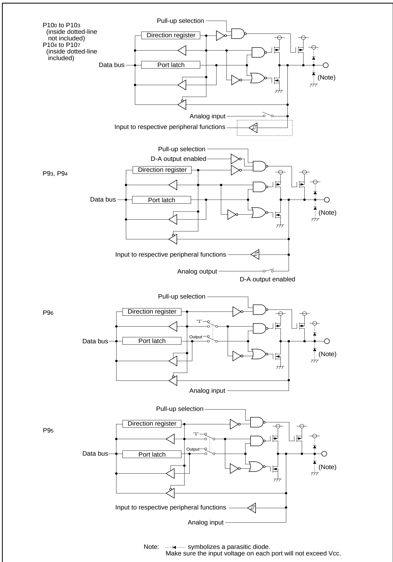
Figure 1.25.4. I/O Ports (4)
