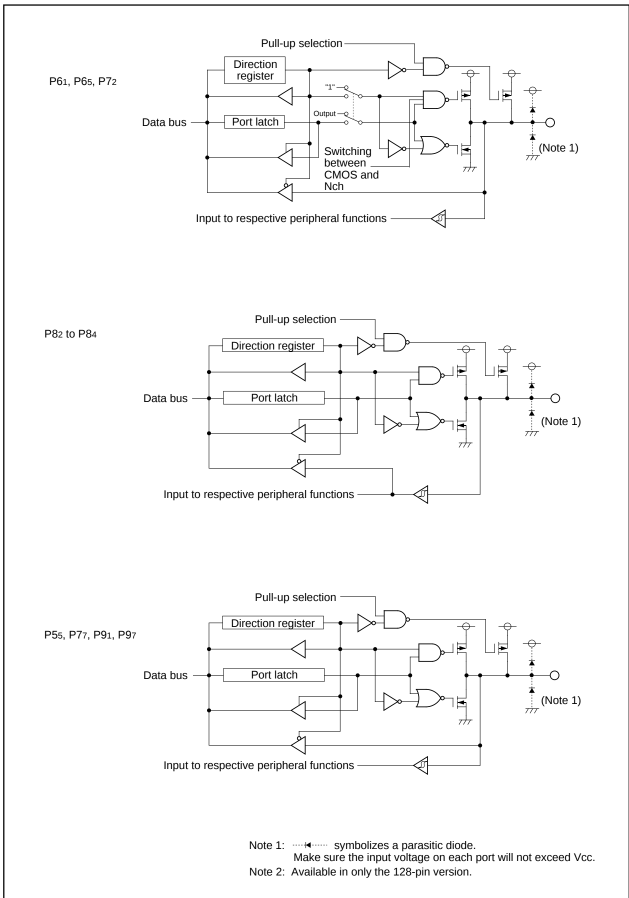
Figure 1.25.2. I/O Ports (2)
