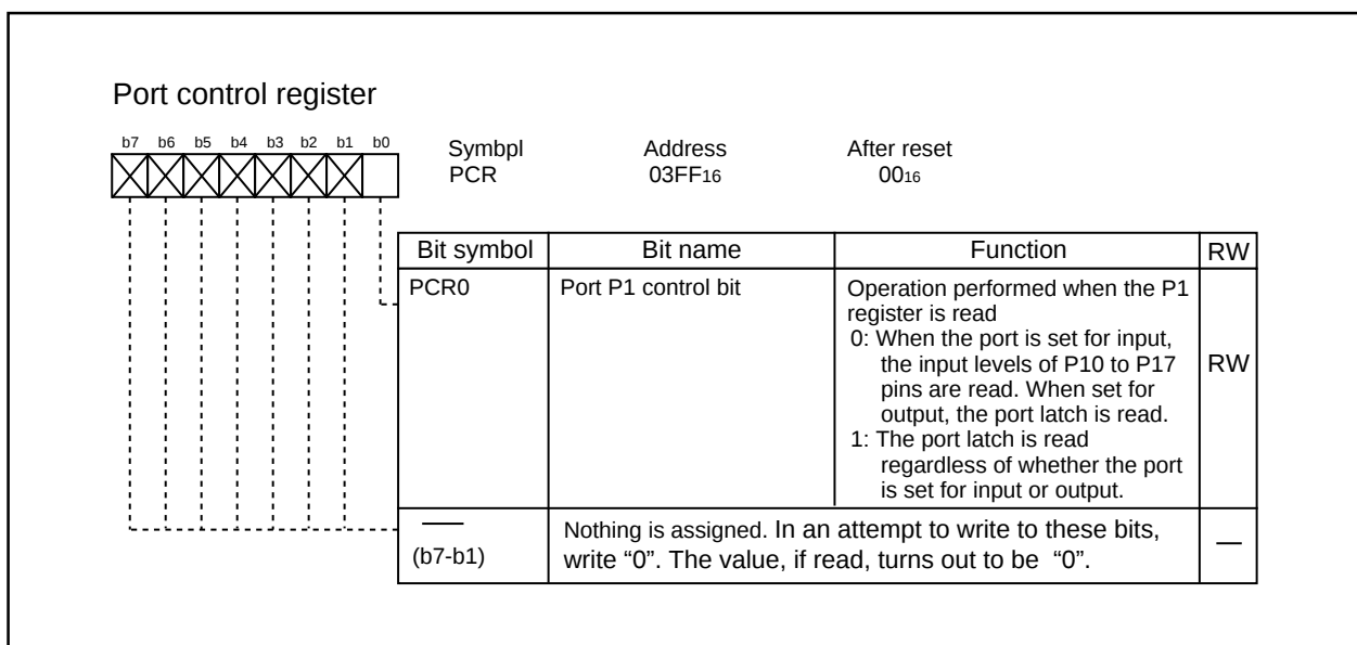
Figure 1.25.11. PCR Register
