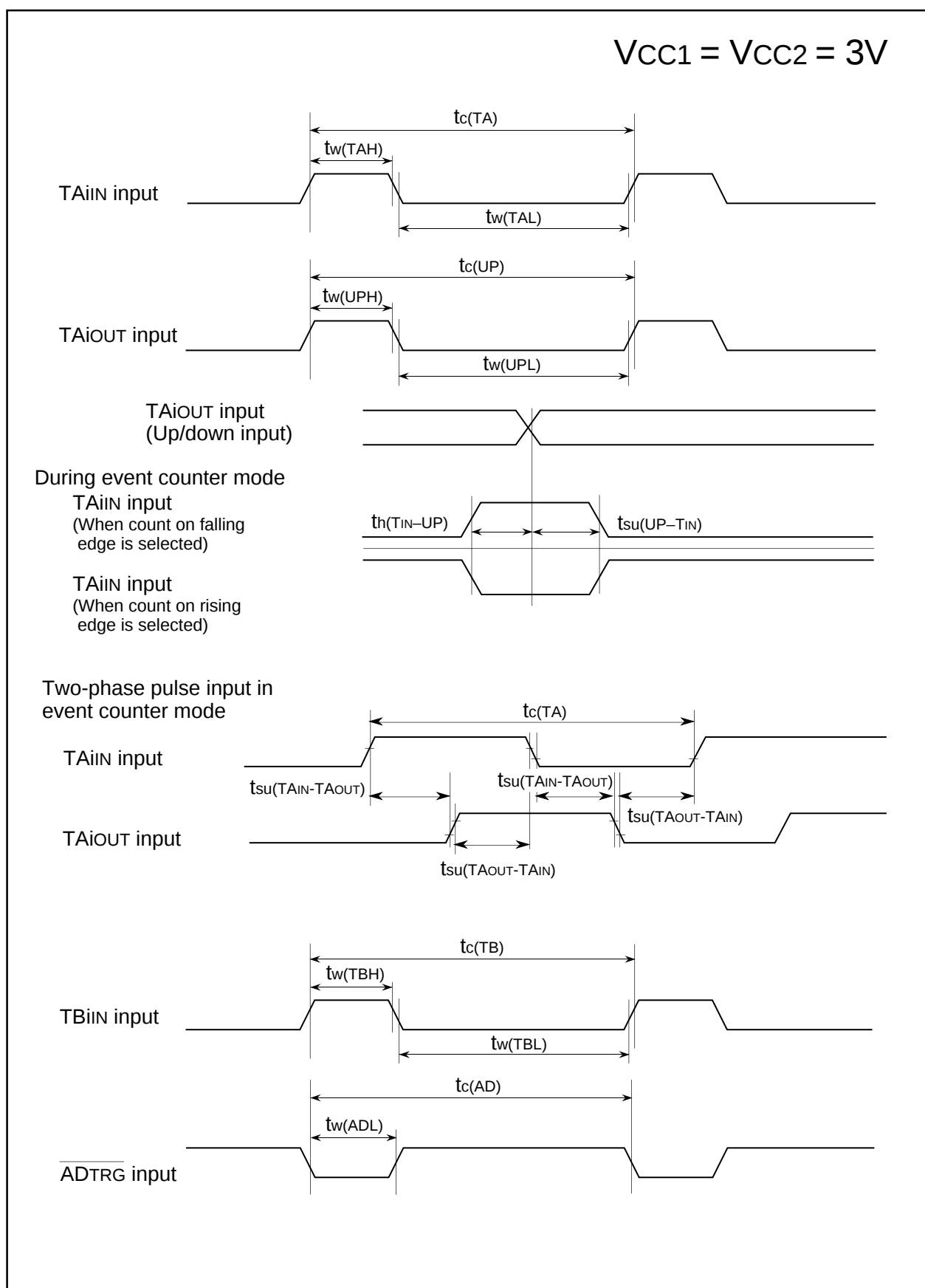
Figure 1.26.12. Timing Diagram (1)
