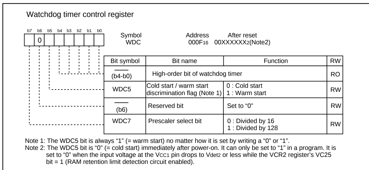
Figure 1.5.5. WDC Register
