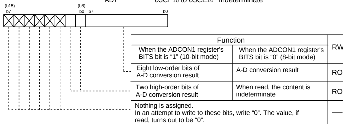
Figure 1.22.3. ADCON2 Register, and AD0 to AD7 Registers
