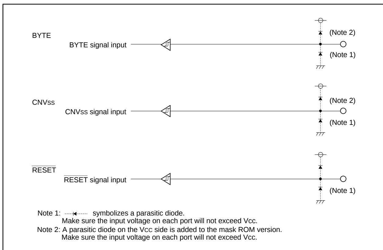
Figure 1.25.6. I/O Pins
