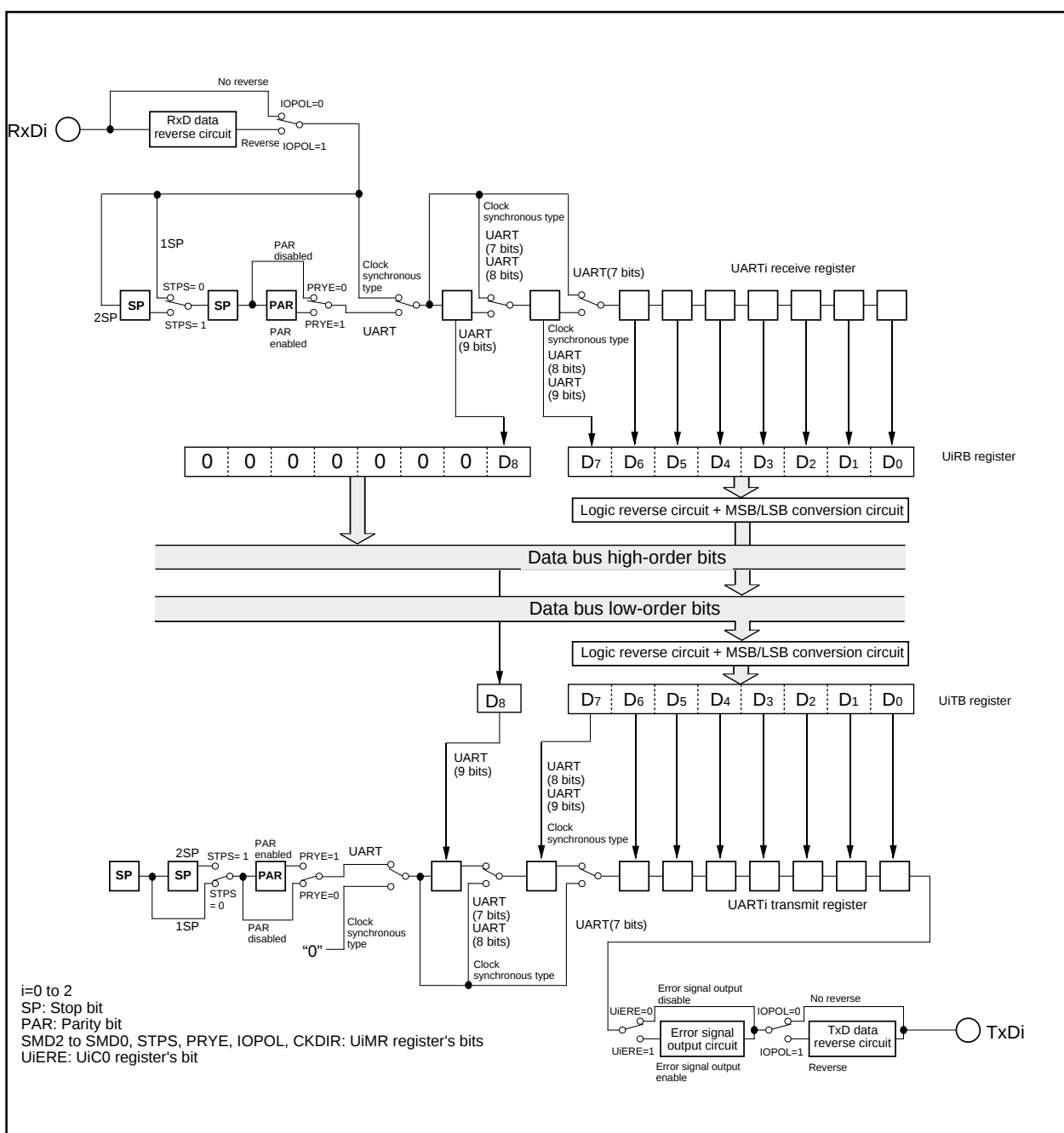
Figure 1.17.2. UARTi Transmit/Receive Unit
