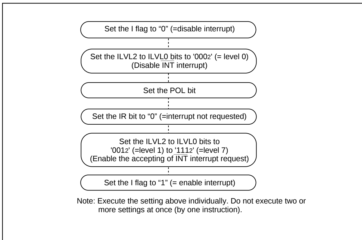
Figure 1.1.1. Procedure for Changing the \overline{\text{INT}} Interrupt Generate Factor
