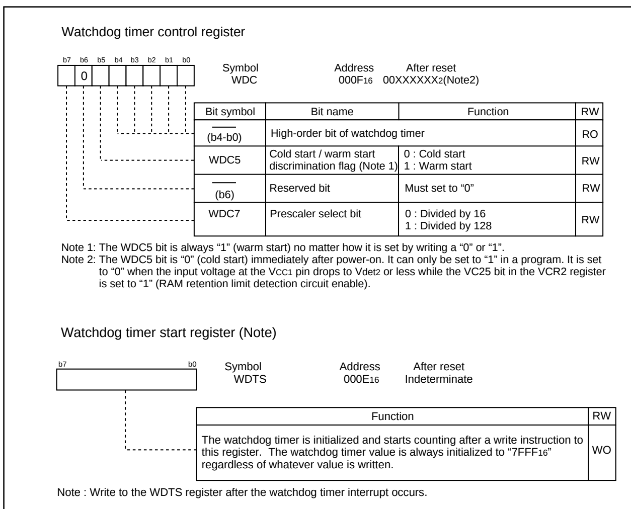
Figure 1.12.2. WDC Register and WDS Register
